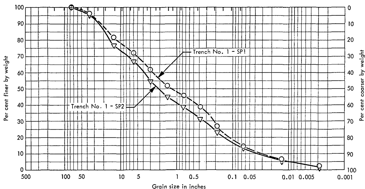
Figure 4.1 Grain size distribution curve for Trench No. 1.
