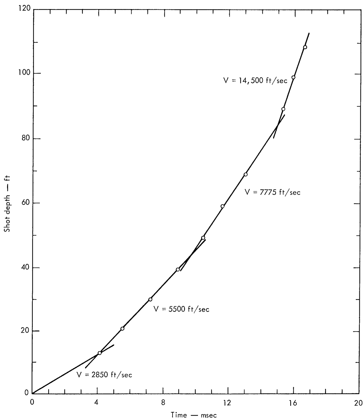
Figure A1 Average velocities (slant-distance corrected)
