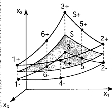
Twelve-noded cohesive element
