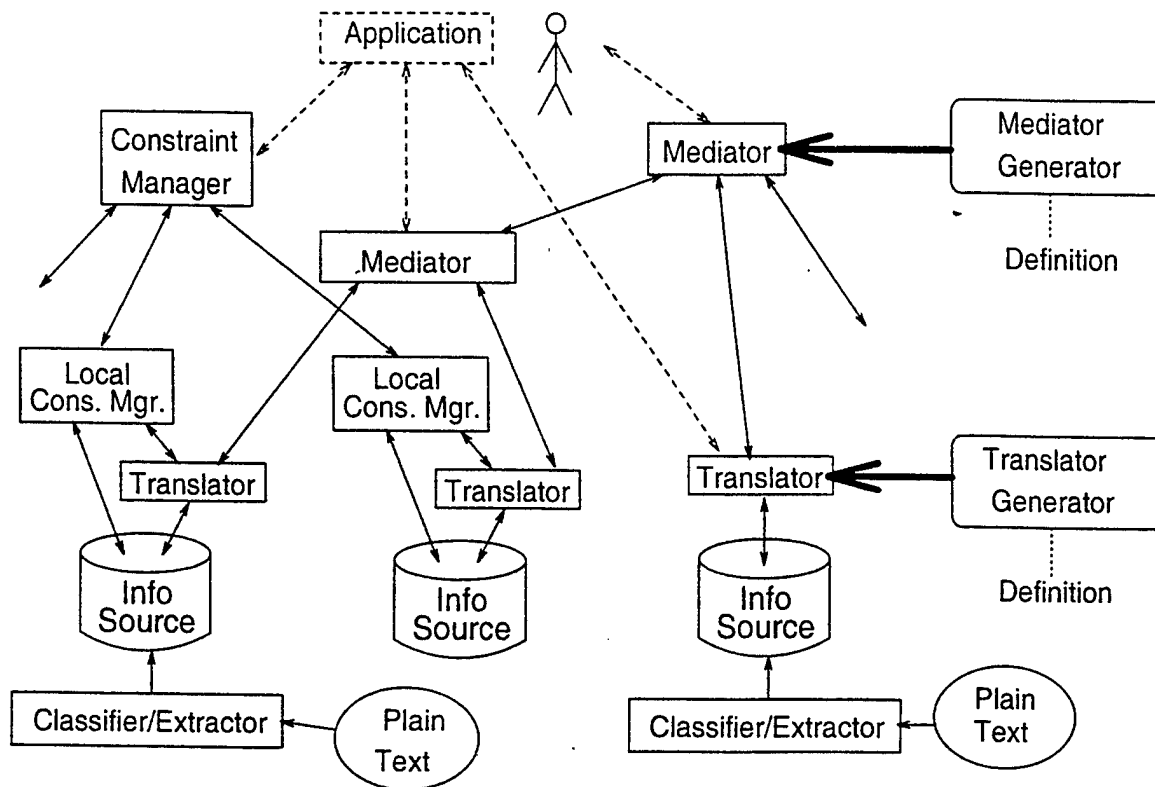
Figure 1: Tsimmis Architecture
