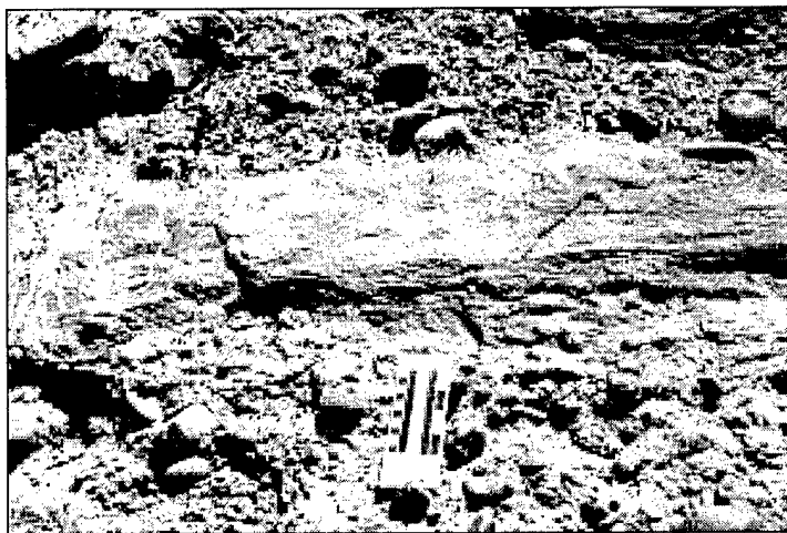
Figure 23. Close-up of planar bedded and cross bedded sand strata within gravel sequence shown in Figure 22.
