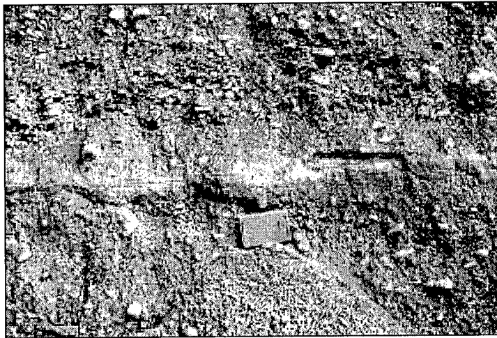
Figure 15. Planar bedded sand interbedded within clast-supported gravel.
