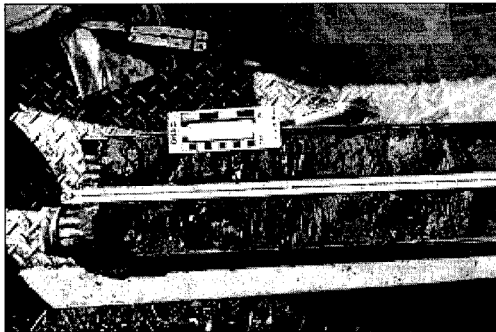
b. Split sample showing a brittle, laminated silt.
