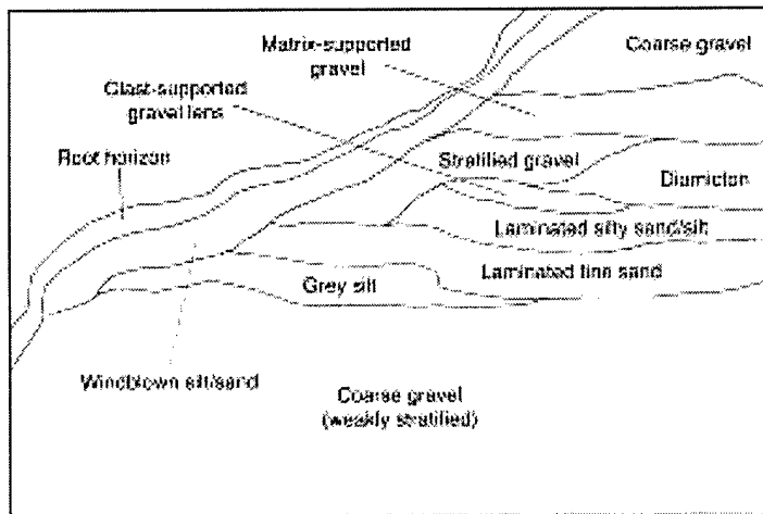
Figure 21. View of Ship Creek section shown in Figure 19, having deformed sand below debris flow deposits. The entire section is capped by a 1.5-m-thick loess deposit.
