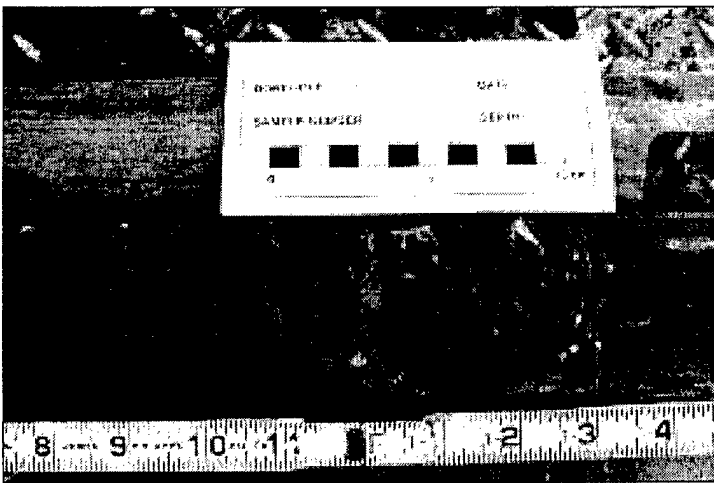
Figure 35. Close-up of poorly sorted diamict (sample 11, AP-3895). Sample has fractured because of a well-developed fissility in the sample.
