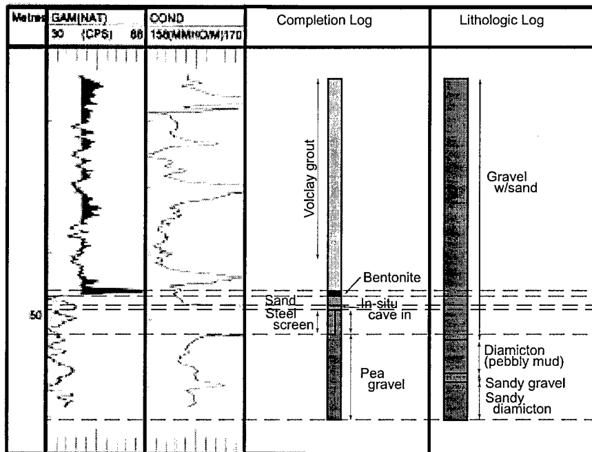
Figure 42. Comparison of geophysical, well completion, and lithologic logs for AP-3469 and A-3888. Natural gamma counts decrease in both wells below the base of the grout. A sharp increase in conductivity in AP-3888 reflects the stainless steel screen placed near the bottom of the well.
