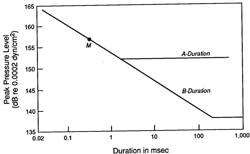
FIGURE 1 The 1968 Impulse Noise Criterion
