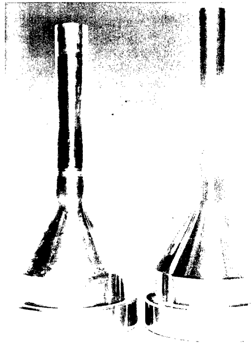
FIGURE 13.—Deformed, quenched, and tempered tool steel extrusion ram (left) compared with a maraging steel replacement. (Photograph supplied by Vasco, a Teledyne company.)
