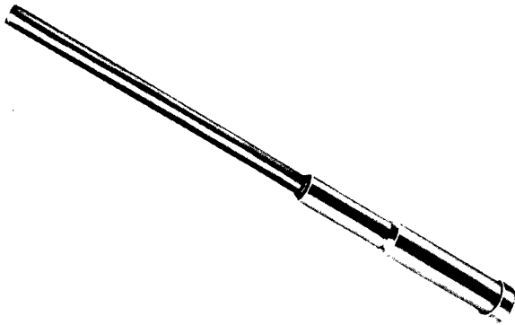
FIGURE 8.—Aluminum die casting core pin manufactured from 250-grade VAR maraging steel; \frac{1}{8} -inch diameter x 12 inches long. (Photograph supplied by Vasco, a Teledyne company.)
