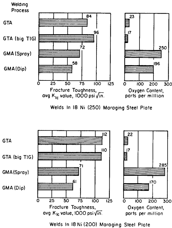
FIGURE 67.—Relationship of oxygen content to fracture toughness in maraging steel welds (ref. 119).
