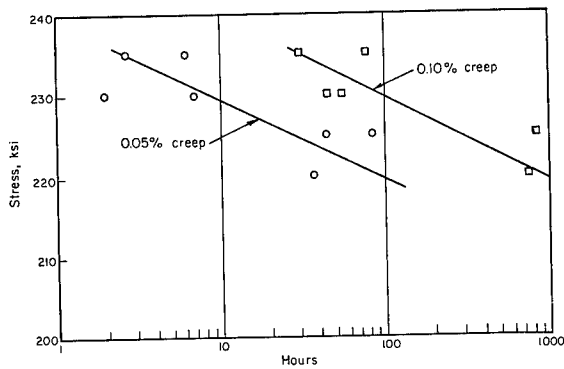
FIGURE 75.—Results of creep tests at 600° F on specimens of 300-grade maraging steel (ref. 143). Condition: Aged at 900° F for 3 hours. Transverse specimens of 0.070-inch sheet. See table 41 for tensile properties of this heat (heat D).
