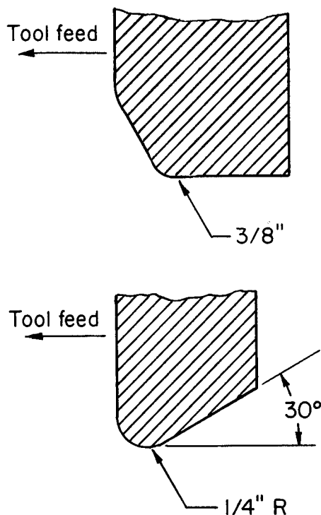
FIGURE 50.—Shear-forming tools for cold-forming maraging steels. These tools are suitable for materials under \frac{3}{16} inch thick (ref. 106).
