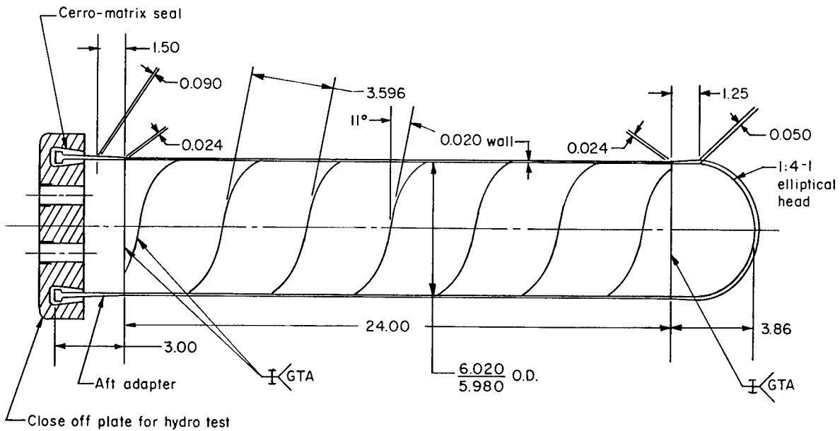
FIGURE 6.—Helically welded rocket-motor case (ref. 13).
