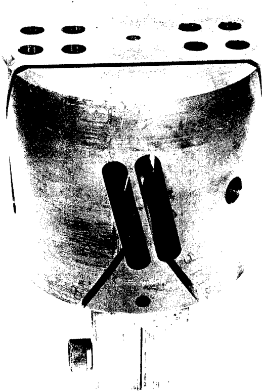
FIGURE 17.—Universal flexure made from VAR 300-grade maraging steel. (Photograph supplied by Vasco, a Teledyne company.)
