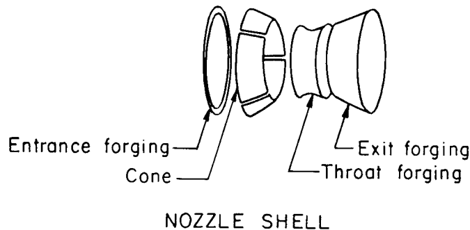
FIGURE 1.—260-inch, short-length case and nozzle shell components.
