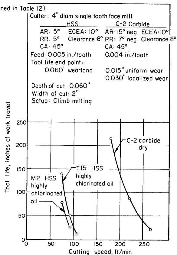
FIGURE 58.—Effect of cutting speed and tool material on tool life in face milling fully aged 18 Ni 250-grade maraging steel (ref. 113).
