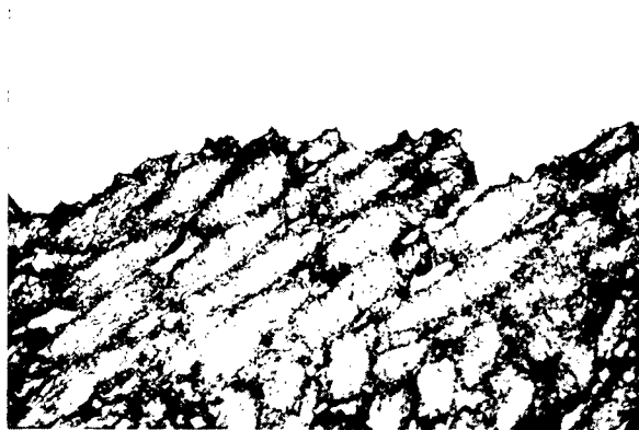
FIGURE 62.—Photomicrographs of the profiles of fracture through 18 Ni 250-grade maraging steel weld metal deposited by the gas-tungsten arc process (ref. 116) \times 375 .
