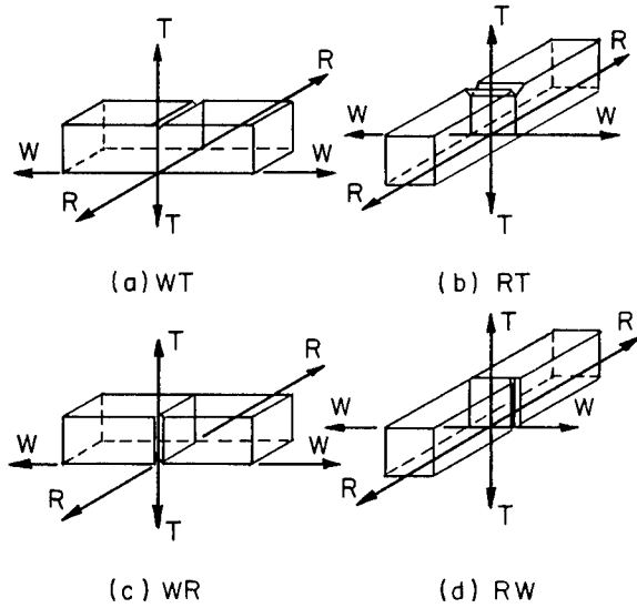
FIGURE 83.—Crack-propagation directions. R=rolling direction W=width direction T=thickness direction
