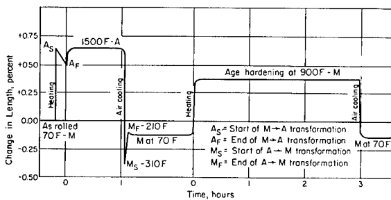
FIGURE 68.—Diagrammatic representation of the dimensional changes that occur during heat treatment of the 18 Ni 250 grade of maraging steel (ref. 100)
