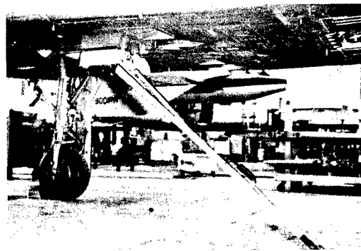
FIGURE 25.—Maraging steel arresting hook for Northrop F-5 tactical fighter.
