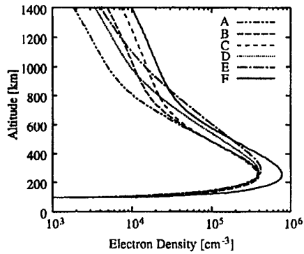
Fig.1 Profiles of background magnetospheric electron density
