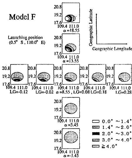
Fig.3 Final locations and incident angle, when parameters of a and LG change (model F)
