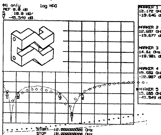
Fig. 3. Waveguide bend in E-plane and its multimode response
