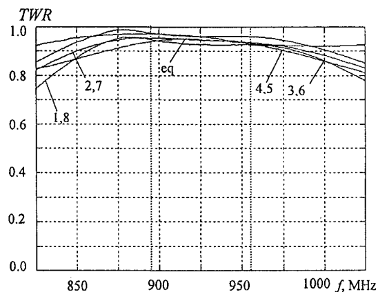
Fig.7. TWR characteristics with matching network.
