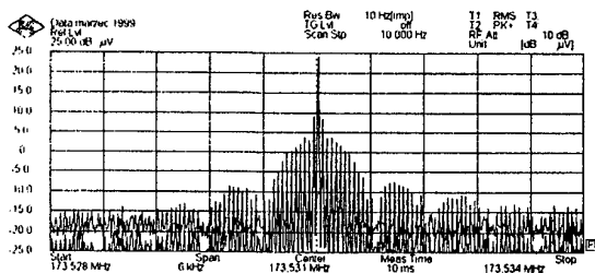
Fig. 3. Spectrum in the vicinity of one spectrum line
