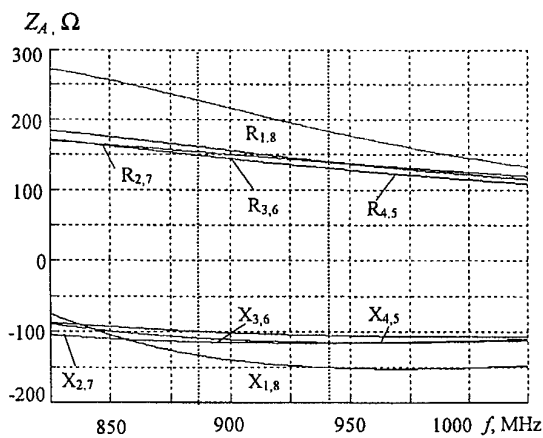
Fig.4. Partial impedance of input ports antenna array.
