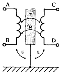
Fig. 1. Electrical and magnetic coupling existing in transformers. A - B primary winding, C - D secondary winding.
