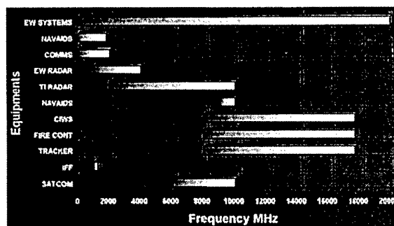
Figure 2. Sensor/Frequency Chart
