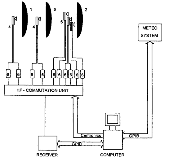
1, 3, 2-: parabolas of INTELSAT 601, 602, and ASTRA/EUTELSAT (multi-beam INTELSAT) receivers, respectively; 4, 5-: front-end PLL receivers/down-converters; 6 - DC/HF-coupler [3]
