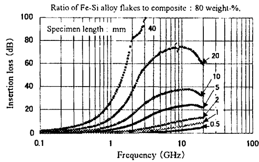
Fig. 7 Frequency characteristics of insertion loss of feed-through type EMI filter.
