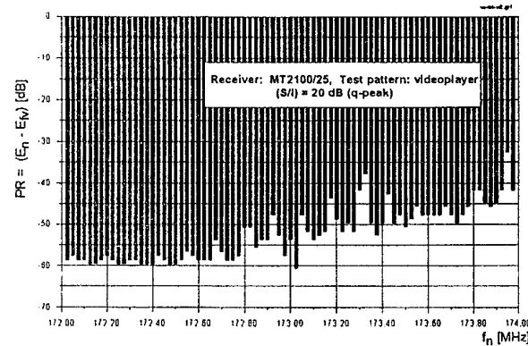
Fig. 12 Receiver MT 2100/25
