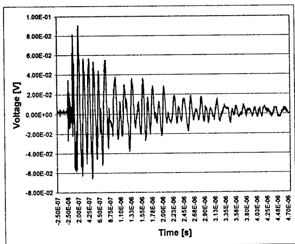
Fig. 6. Time Domain Waveform
