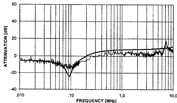
Fig. 9. Calculated and measured transformer attenuation (EMI currents).
