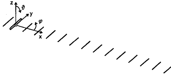
Fig. 2: 15-element Yagi Uda antenna with co-ordinate system.
