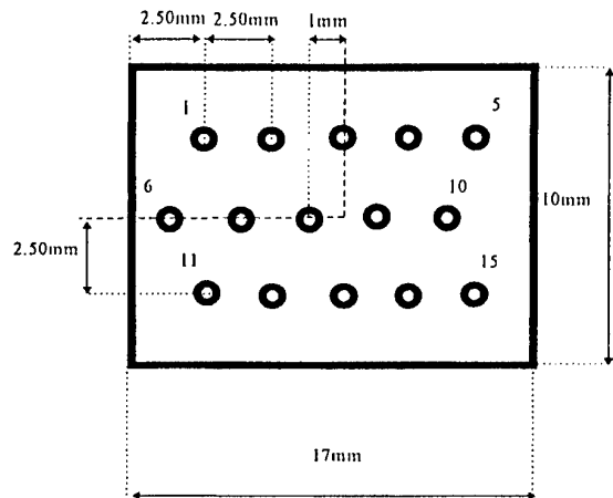
fig.4 Geometry of 15 pin D connector
