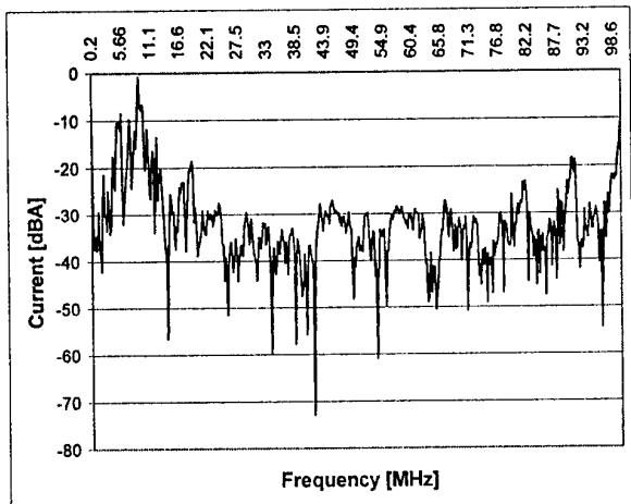
Fig. 7. Current Spectra (Position 1)
