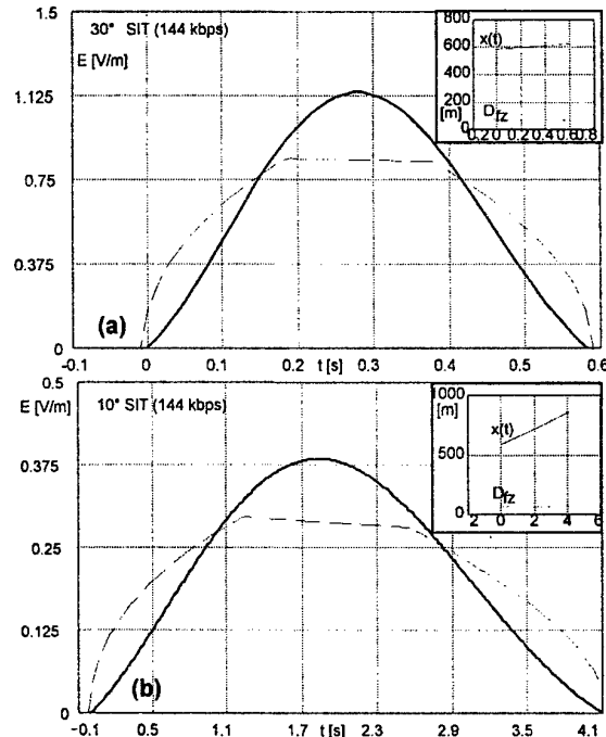
Figure 3. Amplitude of electromagnetic field strength during aircraft travel through the main beam radiated by the antenna of a SIT (144 kbps) for antenna elevation angle a) \epsilon=30^\circ b) \epsilon=10^\circ ( x(t) - distance to the analysed points, D_{fz} - distance to the far zone)
