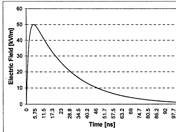
Fig. 4. Electromagnetic Pulse
