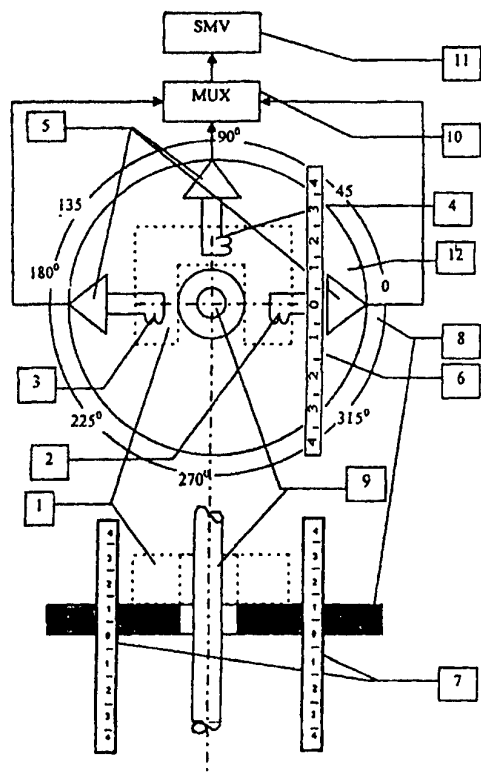
Fig. 5. Instrument installation scheme: 1 - box with "point" sensors; 2, 3, 4 - "point" induction sensors; 5 - preamplifiers of sensors; 6 - measuring ruler for component H_\rho ; 7 - measuring ruler for component H_z ; 8 - measuring limb for component H_\varphi ; 9 - investigated cable; 10 - sensor commutator; 11 - selective microvoltmeter; 12 - movable measuring table.
