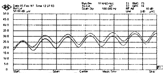
Fig. 4. Test pattern: H-sweep. Resolution bandwidth: 10 KHz
