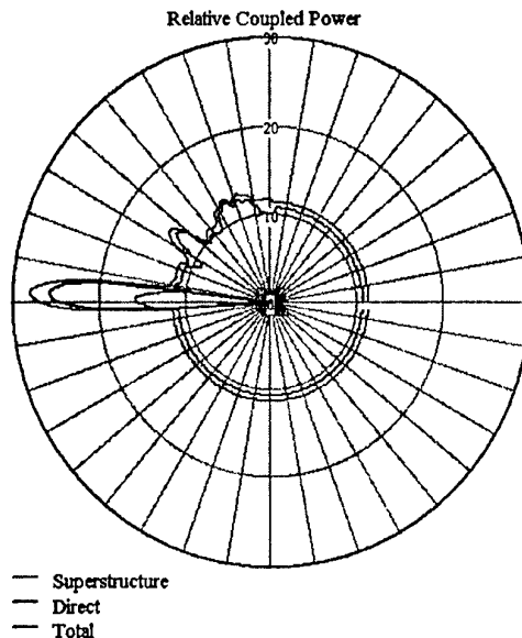
Figure 7. Polar Plot
