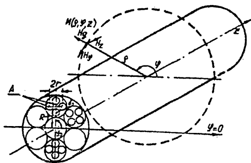
Fig. 4. Attitude of measuring point M(\rho, \varphi, z) near a cable
