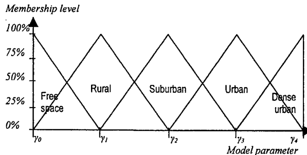
Fig. 5. Classification of propagation environment by means of fuzzy sets (from S. Faruque [9])
