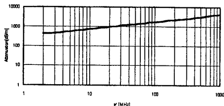
Fig.3 Relative attenuation for CEF material
