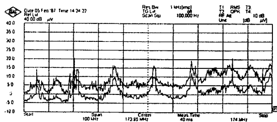
Fig. 2. Test pattern: H-sweep. Resolution bandwidth: 1 KHz. Detectors used: peak - upper curve; rms - lower curve
