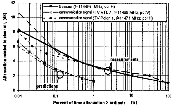
Fig. 2. Cumulative distributions of atmospheric attenuation exceeded in percent of total time of campaign duration in Wrocław for EUTELSAT II Hot Bird satellite signals [4], [5], [7].
