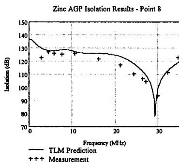
Fig. 9: Comparison between isolation measurements and TLM predictions.
