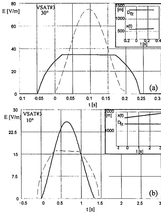
Figure 7. Amplitude of electromagnetic field strength during passage of the aircraft through the main beam of the VSAT#3 antenna for elevation angle of the antenna (a) \epsilon=30^\circ ; (b) \epsilon=10^\circ
