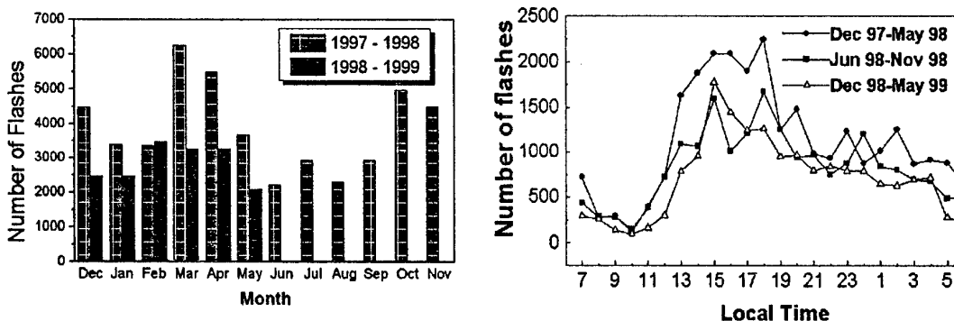
Fig. 1. Monthly variation (left) and diurnal variation (right) of lightning activity over Indonesia (6°N-11°S and 95°E -141°E). December 1997 to May or June 1998 correspond to the El Niño period and the other months correspond to the normal period.
