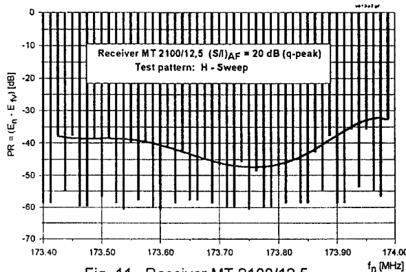
Fig. 11 Receiver MT 2100/12.5
