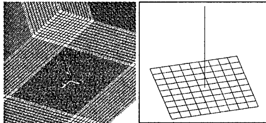
Fig. 10: TLM and NEC models of a 10 metre whip monopole on a ground plane
