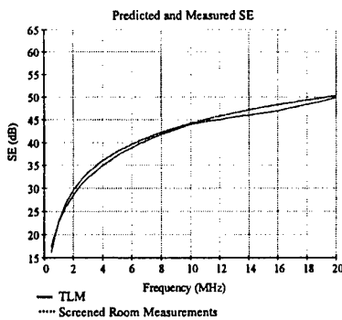
Fig 7: Comparison with experimental data of the TLM model of the screened room with a flectron panel
