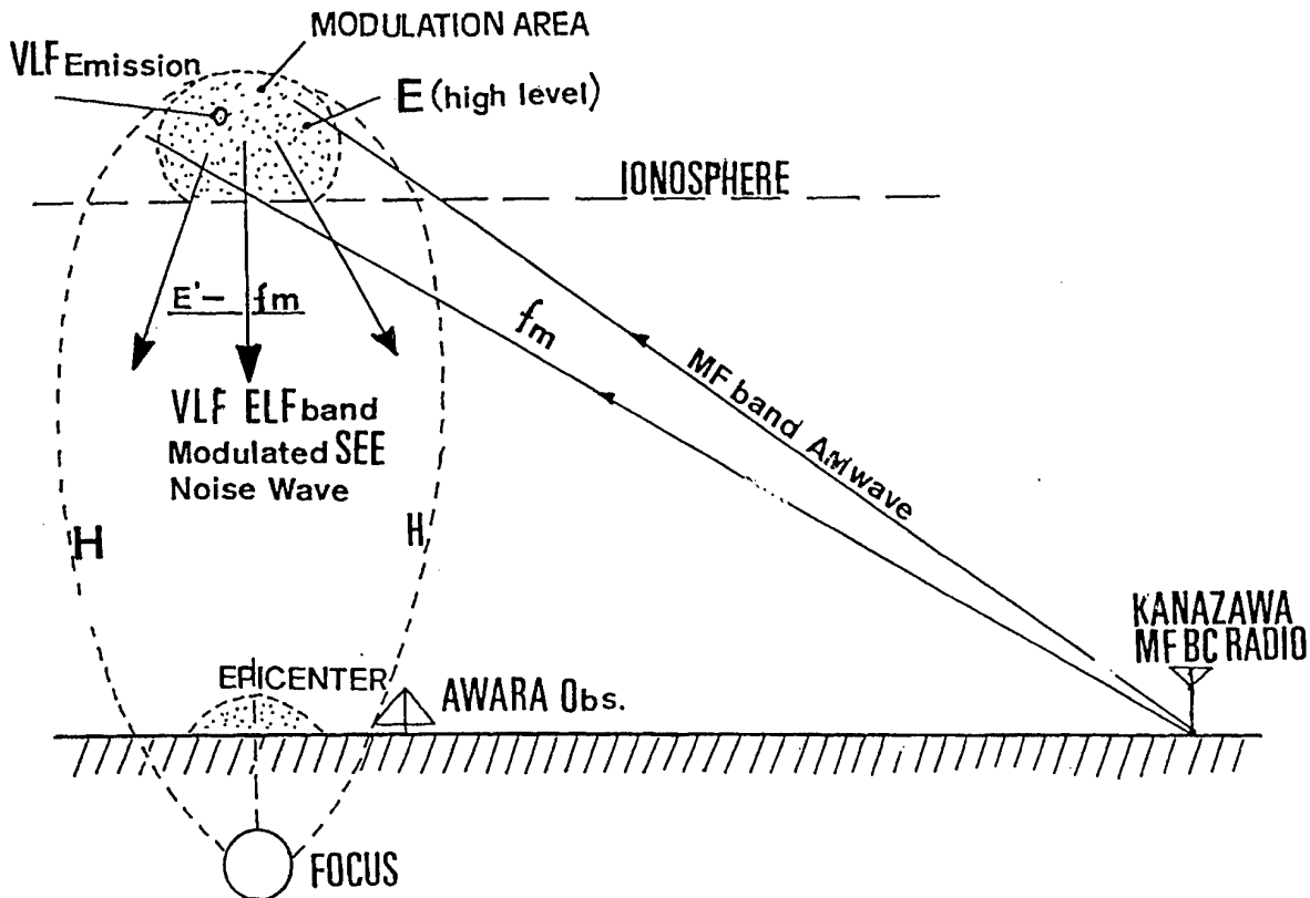
Fig. 4 A geometry profile of the vertically profile of the vertically relationship between the energy transmission path of MF broadcasting stations from Kanazawa, location of bottom of ionosphere, focus and epicenter of earthquake and the location of Awara obs. 10 km from epi.
