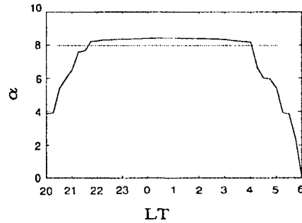
Fig.4 Variation of a with LT.
