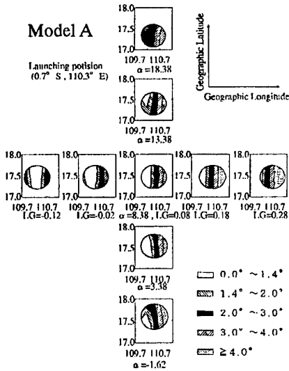
Fig.2 Final locations and incident angle, when parameters of a and LG change (model A)
