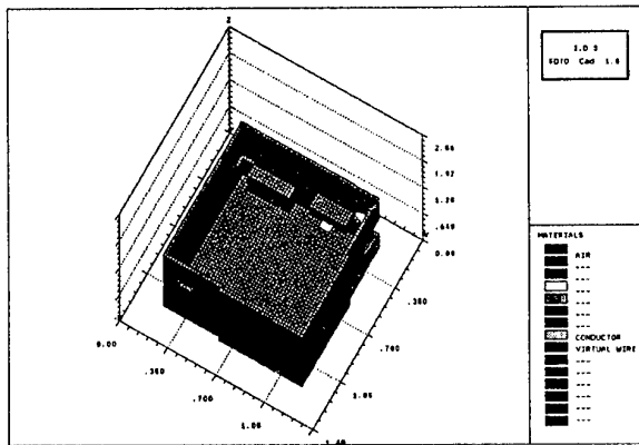
Fig. 5 – Internal view
