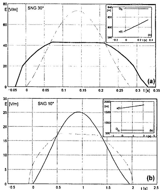
Figure 6. Amplitude of electromagnetic field strength during aircraft travel through the main beam radiated by the antenna of a typical SNG for antenna elevation angle (a) \varepsilon=30^\circ , (b) \varepsilon=10^\circ
