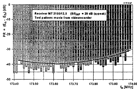
Fig. 10 Receiver MT 2100/12.5
