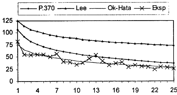
Fig. 1. Measurement results in Vilnius district (160 MHz). Here and below - R , km, vs. E_R , dB( \mu V/m)
