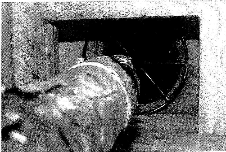
Figure 33(a). Core buster installed at the entrance to the augmeter tube of the NFESC test cell model.
