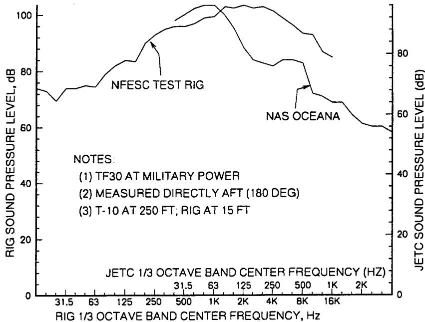
Figure 15. Comparison of the T-10 test cell noise spectrum with noise generated by the NFESC test cell model.
