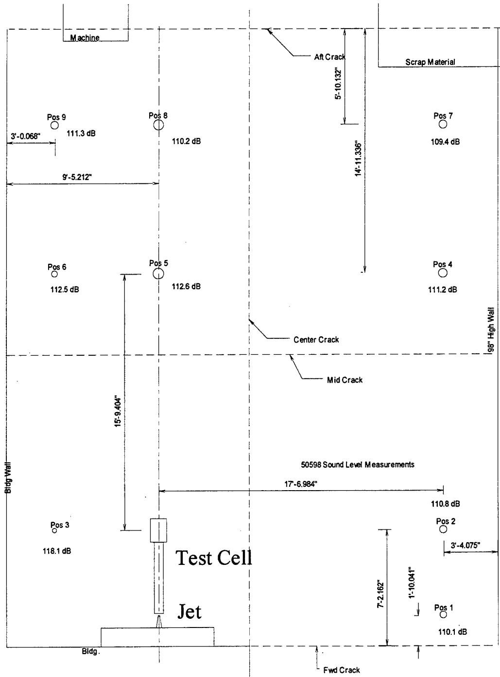
Figure 13. Plan view of the vicinity of the NFESC test cell model.
