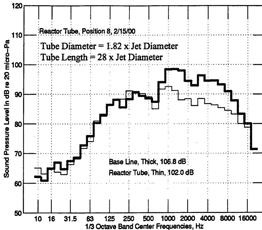
Figure 37. The effect of a single tube placed at the engine nozzle on Sound emissions from the NFESC test cell.
