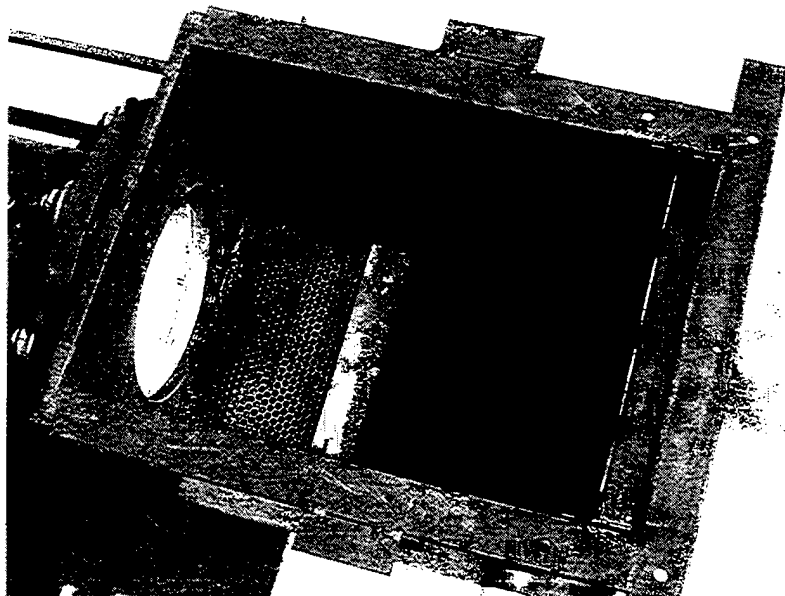
Figure 46. Curved ramp tested in the exhaust stack of the NFESC test cell.
