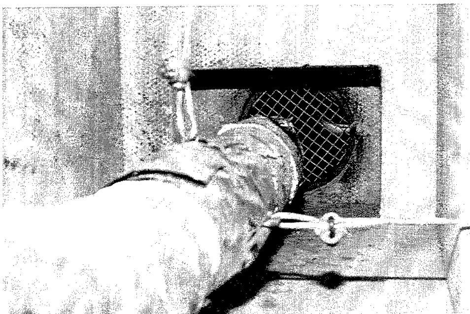
Figure 33(b). Screen installed at the entrance to the augmeter tube of the NFESC test cell model to break up large scale turbulence.
