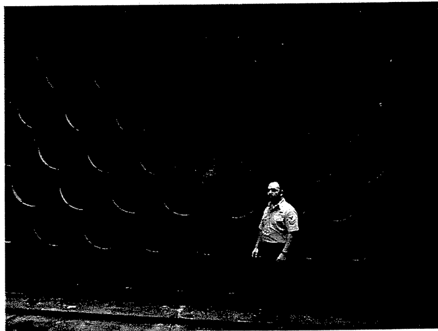
Figure 10. Rectifier tubes installed at the end of the augmenter tube of the hush house at NAF Atsugi.
