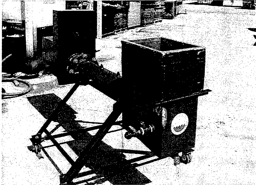
Figure 39. High exhaust stack added to NFESC test cell physical model.
