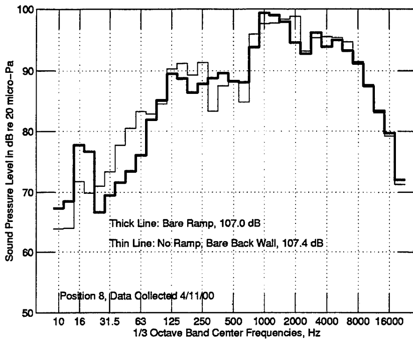
Figure 43(a). Comparison of the acoustic performance of the NFESC model exhaust stack with 45-degree ramp and the exhaust stack without the ramp. The augments tube thus discharges against the back wall of the exhaust stack. Neither the ramp nor walls of the stack are insulated.
