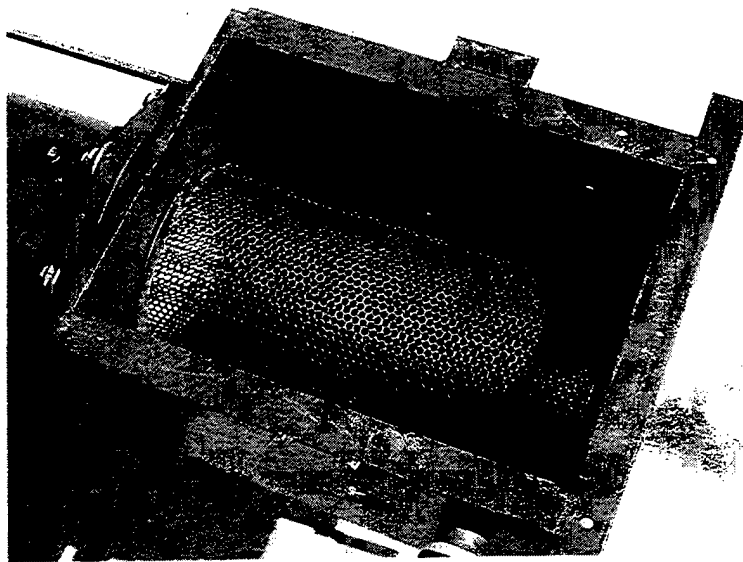
Figure 48. Colander installed at the end of the augmenter tube of the NFESC test cell.
