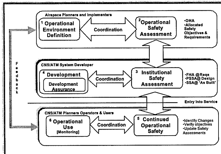
Figure 5-1. Overview of the CNS/ATM safety assessment process
