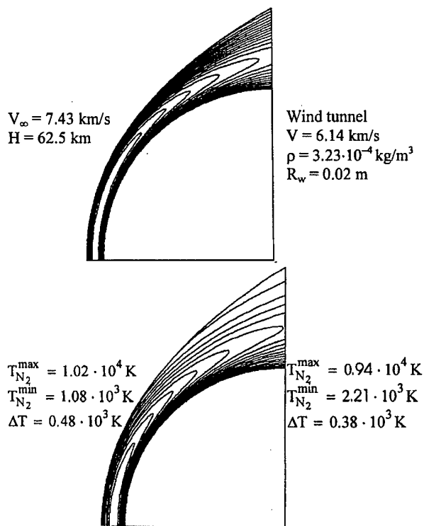
Fig.5. T_{N_2} isolines in the shock layer
