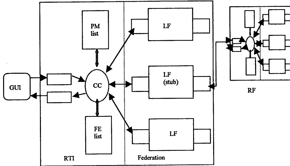
Figure 1 AMASE Architecture
