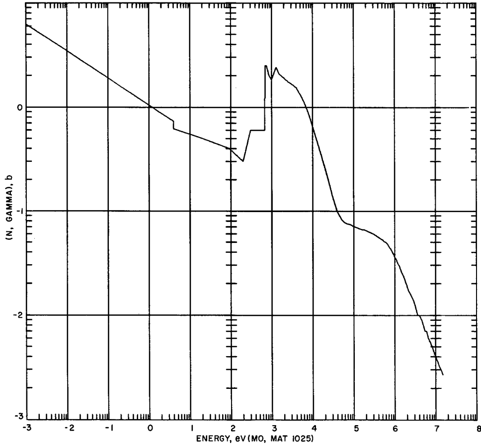
Fig. 34. Molybdenum Smooth (n,γ) Cross Section
