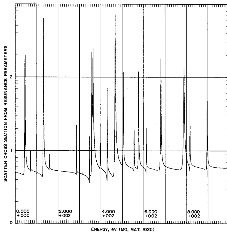
Fig. 48. Molybdenum Elastic Scattering Cross Section from Resonance Parameters, 4-1000 eV
