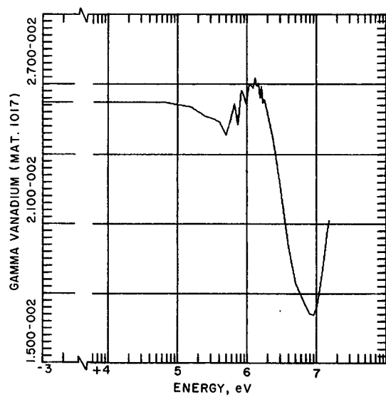
Fig. 29 Vanadium \gamma
