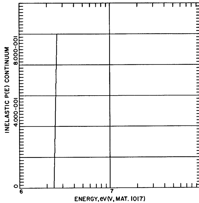
Fig. 84. Vanadium--Probability for Inelastic Scattering to the Continuum
