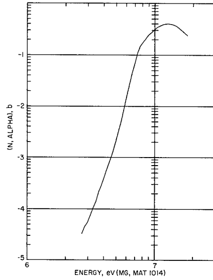
Fig. 6 Magnesium (n,α) Cross Section
