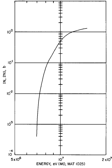
Fig. 33 Molybdenum (n,2n) Cross Section
