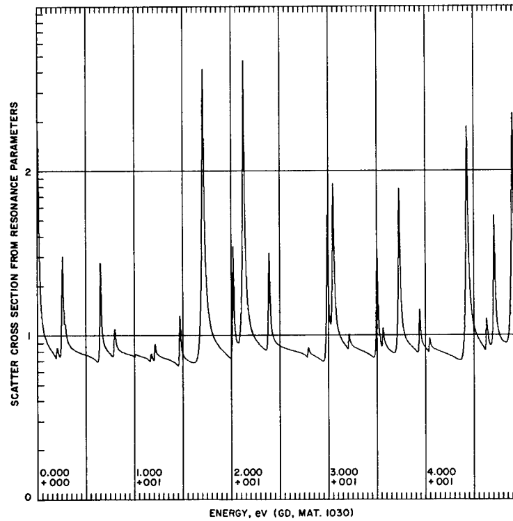
Fig. 51. Gadolinium Elastic Scattering Cross Section from Resonance Parameters below 50 eV
