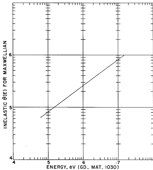
Fig. 95. Gadolinium-- \theta(E) for Inelastic Scattering
