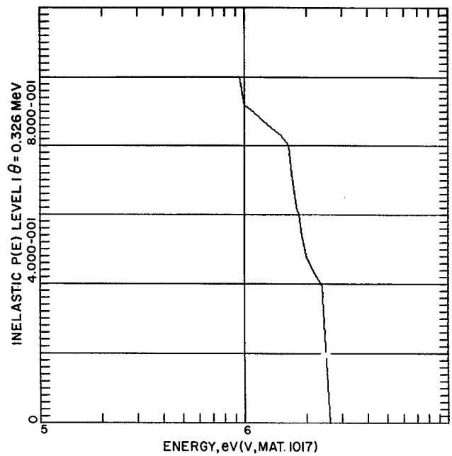
Fig. 80. Vanadium--Probability for Inelastic Scattering to the First Level
