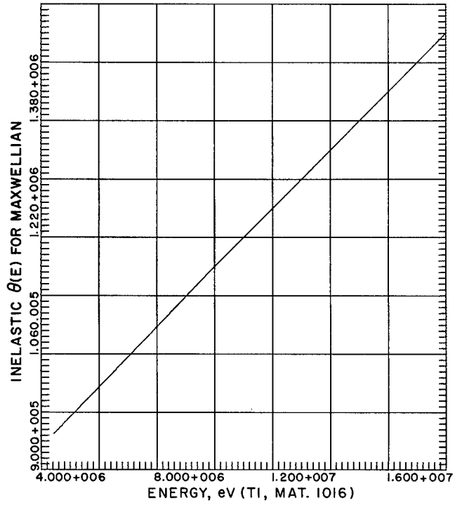
Fig. 78. Titanium-- \theta(E) for Inelastic Scattering
