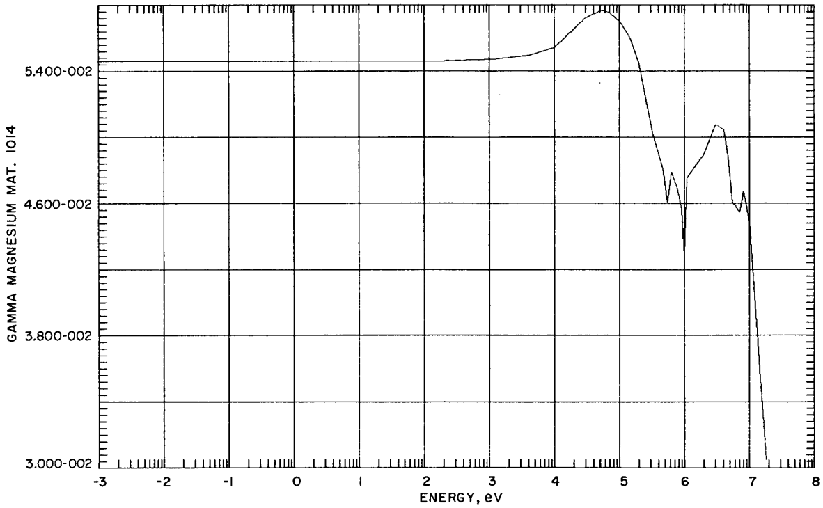
Fig. 9. Magnesium \gamma
