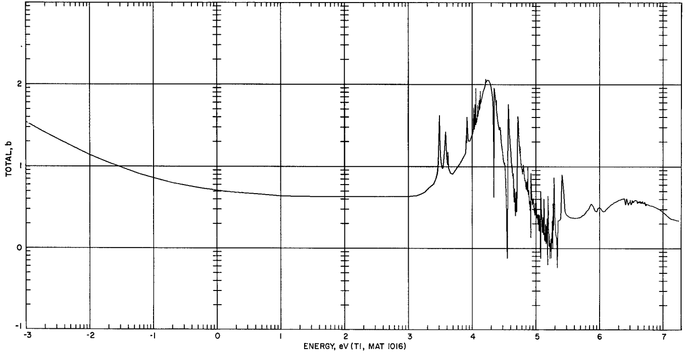
Fig. 10. Titanium Total Cross Section
