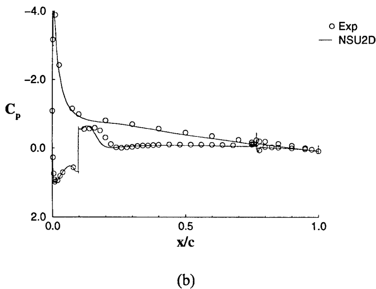
FIGURE 87. (a) STREAMLINES AND (b) SURFACE PRESSURE DISTRIBUTIONS FOR A NACA 23012m WITH k/c = 0.0083 QUARTER-ROUND ICE SHAPE LOCATED AT x/c = 0.1 AND \alpha = -6
