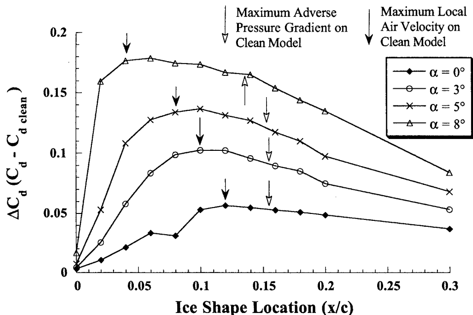
FIGURE 56. DRAG INCREASE DUE TO SIMULATED ICE SHAPE AT VARIOUS LOCATIONS (NACA 23012m, forward-facing quarter round, boundary layer tripped for case with simulated ice at x/c \geq 0.04 , Re = 1.8 million)
