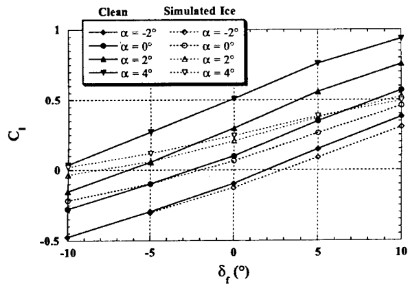
(a) Lift
