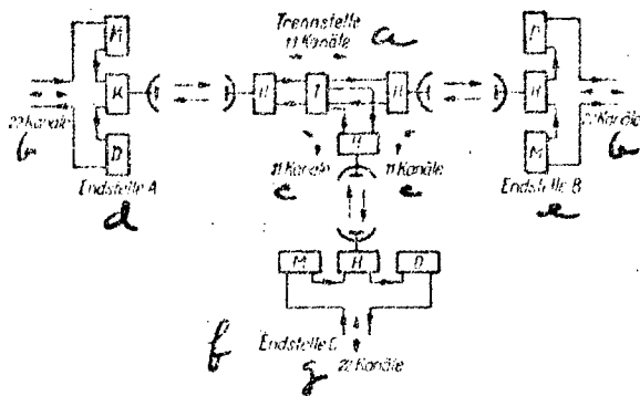
Figure 17 Radio Relay with Shunting Point
