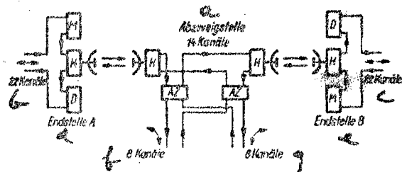
Figure 16 Radio Relay with Shunting Point
