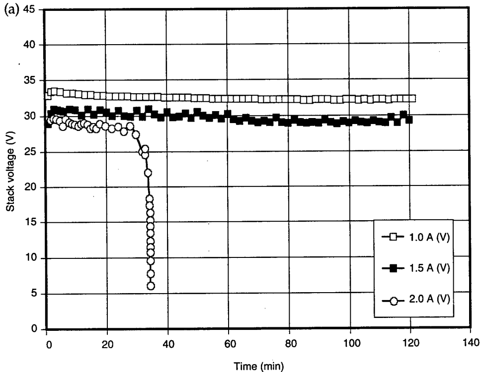
Figure 7. Constant current discharge performance of 50-W fuel cell stack (CECOM 764) at 20 °C: (a) voltage vs time and (b) power vs time. H 2 inlet pressure = 3 psi; air inlet pressure = 5 psi; H 2 purging: 10 s/5 min; cooling by fan; dry H 2 and dry air fill.
