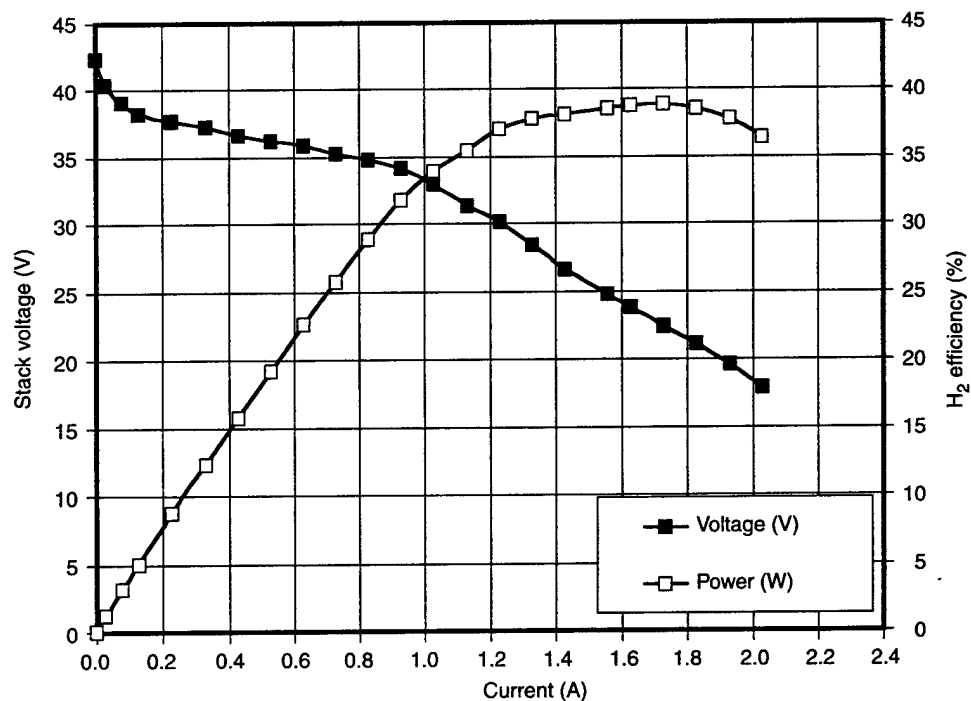
Figure 12. Discharge performance of 50-W fuel cell stack (CECOM 762) at 25 °C. Dry air and dry H 2 fill; H 2 pressure = 3 psi; air pressure = 5 psi; H 2 purging: 10 s/5 min; at 2.03 A, stack temperature increased to 52 °C.
