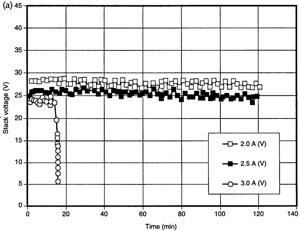
Figure 9. Constant current discharge performance of 50-W fuel cell stack (CECOM 764) at -5^{\circ}\text{C} : (a) voltage vs time and (b) power vs time. \text{H}_2 inlet pressure = 3 psi; air inlet pressure = 5 psi; \text{H}_2 purging: 10 s/5 min; cooling by fan; dry \text{H}_2 and dry air fill.
