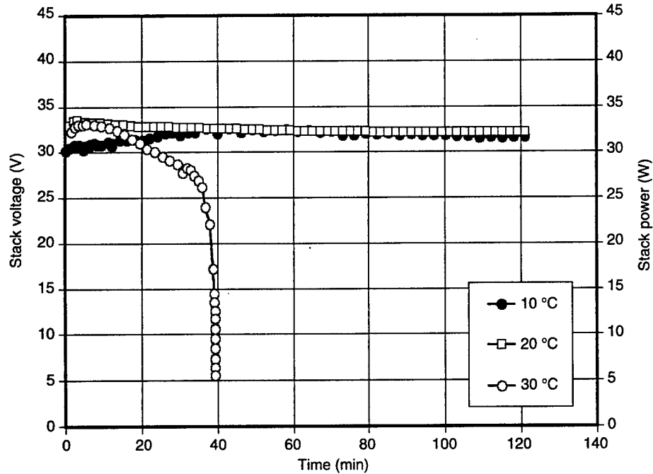
Figure 4. Constant current discharge ( I = 1.0 \text{ A} ) performance of 50-W fuel cell stack (CECOM 764) at different environmental temperatures. \text{H}_2 inlet pressure = 3 psi; air inlet pressure = 5 psi; \text{H}_2 purging: 10 s/5 min; cooling by fan; dry \text{H}_2 and dry air fill.
