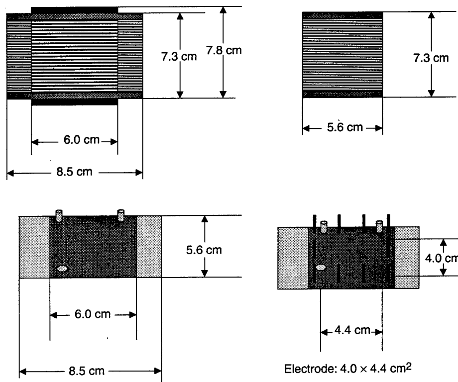
Figure 1. Dimensional drawing of 50-W fuel cell stack (42 cells, CECOM 762 or 764). Dry weight (before electrolyte membrane was humidified): 637 g (including two electric wires and two H 2 tubes, and excluding air or water tubes); wet weight (after membrane was humidified): 643 g.
