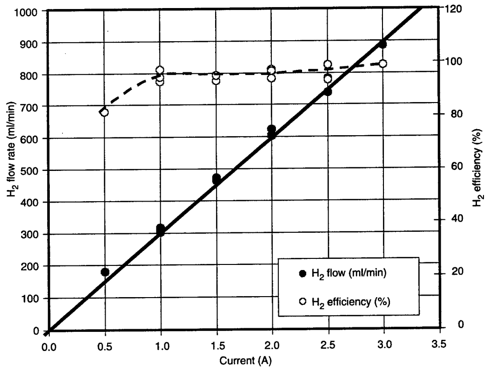
Figure 10. Effect of current on H_2 flow rate and H_2 efficiency for 50-W fuel cell stack (CECOM 764, containing 42 single cells connected in series).
