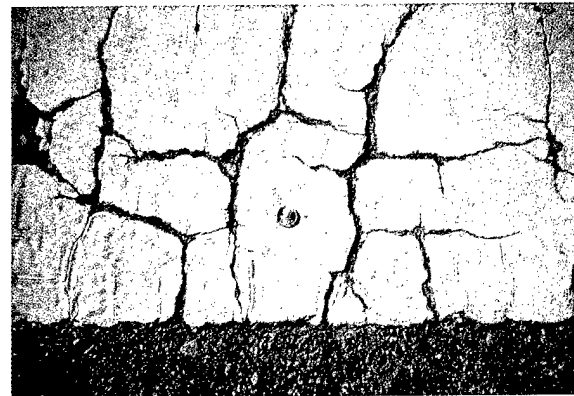
Advanced stage of APC.
