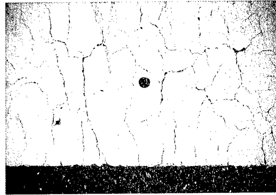
Early stage of APC.
