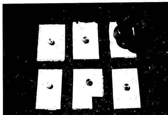
Elcometer adhesion tester and 3/4" pull-off pucks attached to paint samples.
