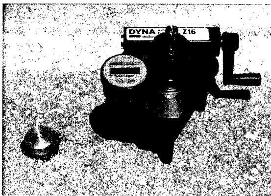
Proceq Dyna Tester and 2" pull-off puck.
