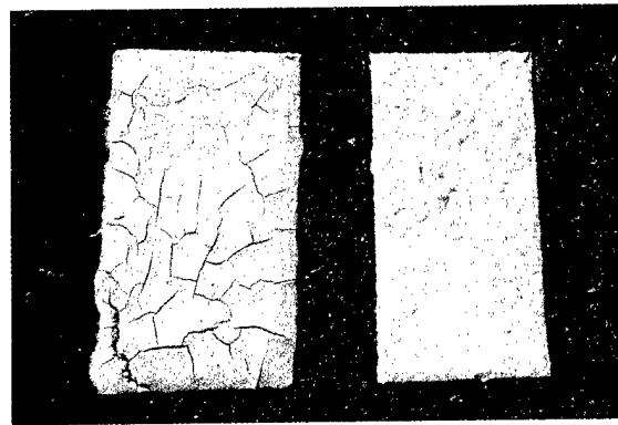
Paint I (left), Paint HB (right).
