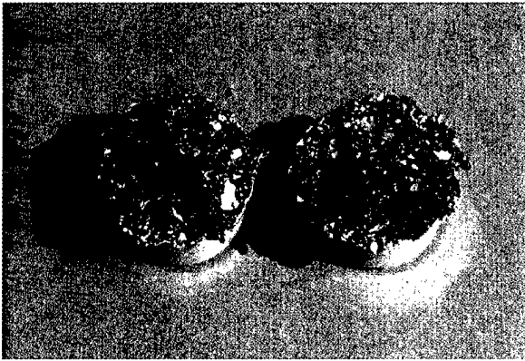
Paint with attached chunks of AC indicate paint adhesion > AC cohesive strength.
