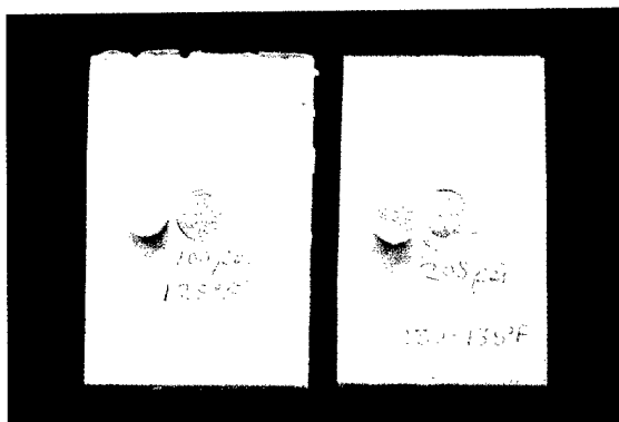
Pull-off pucks and samples with resulting paint cohesive failures.
