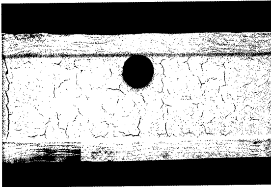
Paint I cracking at > 30 mils DFT.
