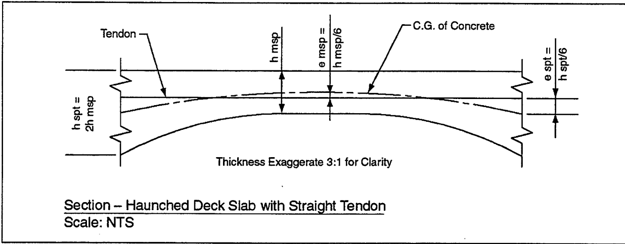
Figure 10-4 Section – Haunched Deck Slab with Straight Tendon
