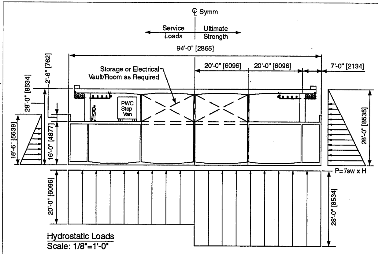
Figure 7-1 Hydrostatic Loads
