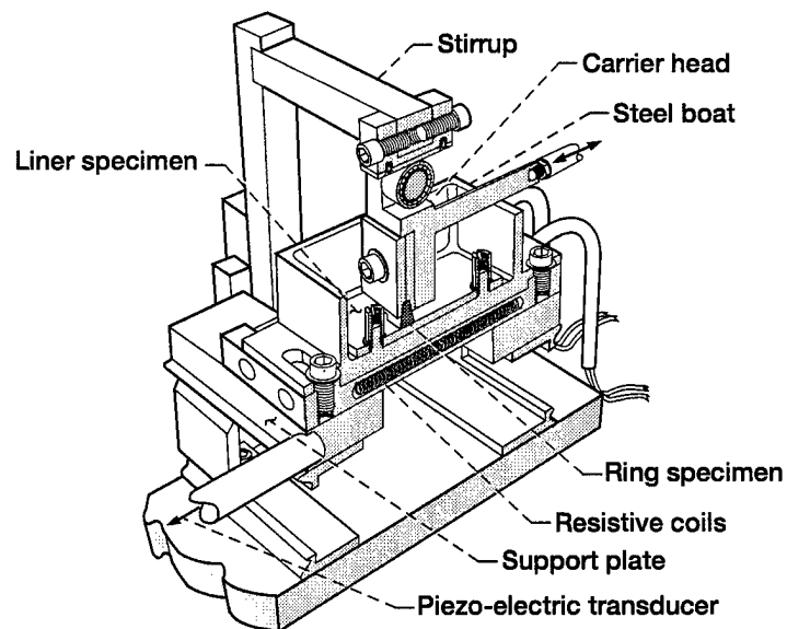
Figure 3.—Schematic of the reciprocating wear rig.
