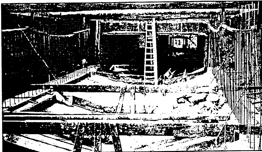
Figure 76. Section of the Broad St. Canal showing reinforced concrete canal construction, 1914 (from Sewerage & Water Board 1914).
