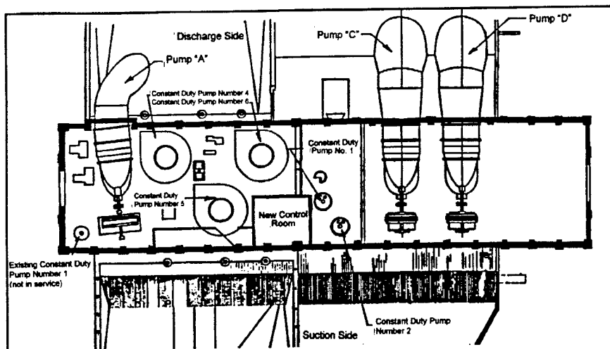
Figure 102. Drainage Pumping Station No. 7. Plan of existing station (NODCOE).
