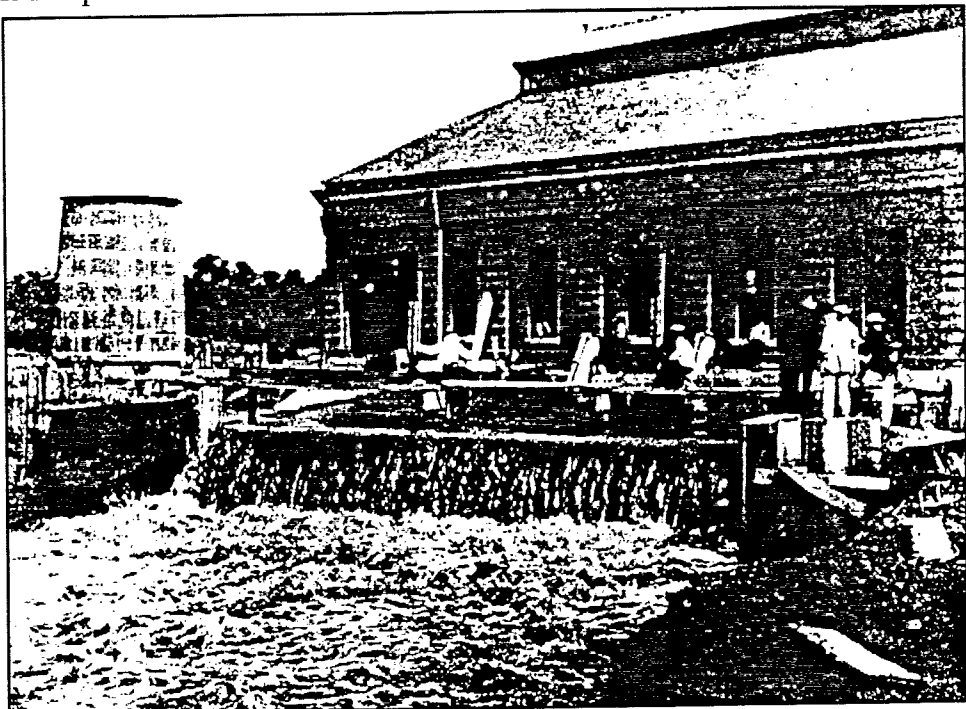
Figure 21. Drainage Pumping Station No. 1 during pump testing, 1904. The original caption states: "...shows one pump throwing 250 cubic feet of water per second over a weir erected for testing capacity of pumps. There are three similar pumps at this station" (from Sewerage & Water Board 1904).
