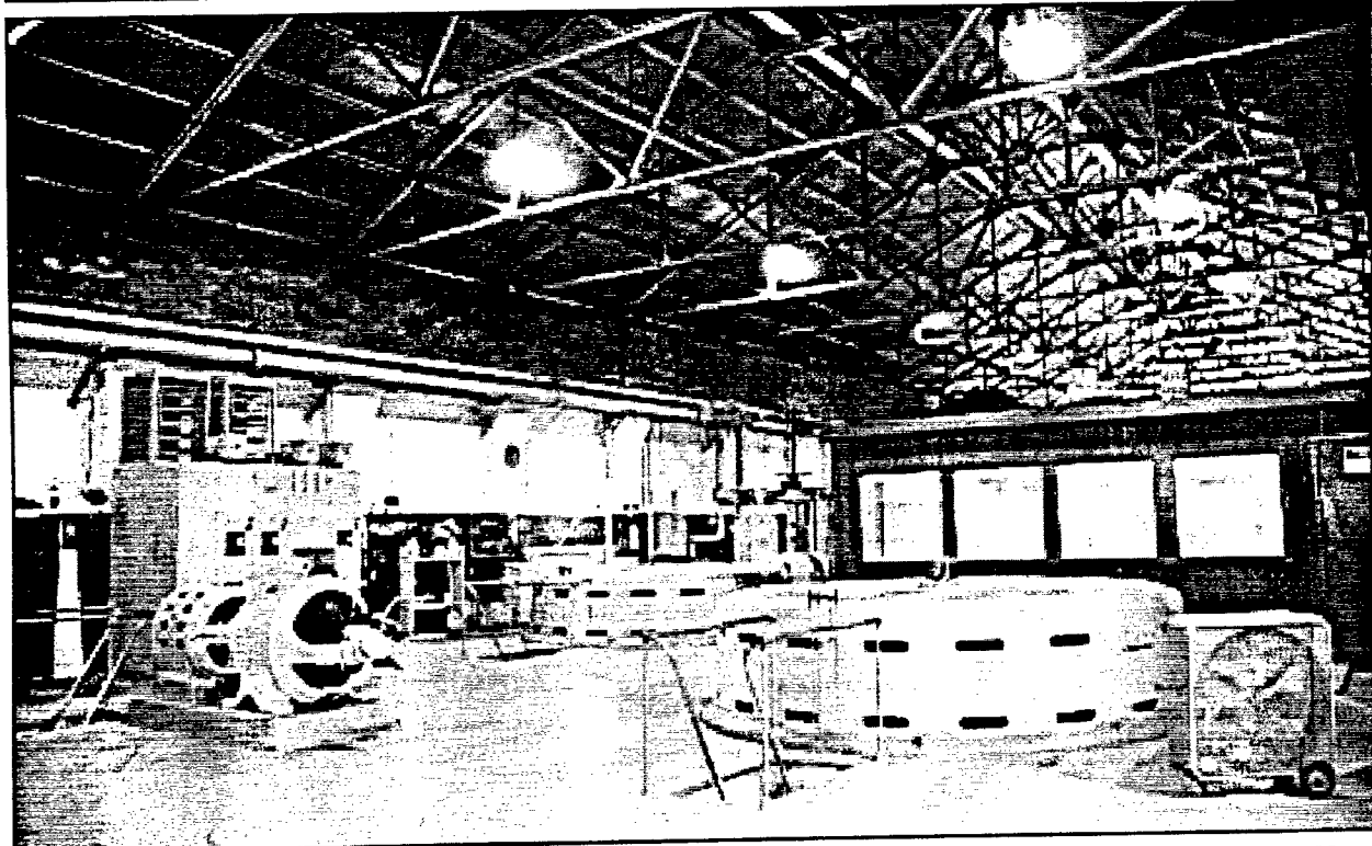
Figure 64. Drainage Pumping Station No. 7. View of interior, showing motor covers of 250 cfs centrifugal "flathead" pumps.
