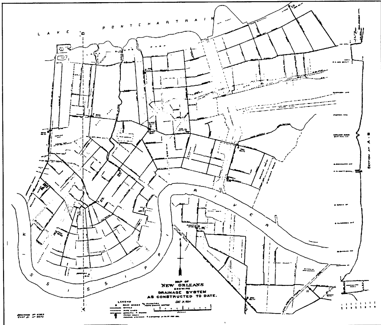
Figure 12. The New Orleans Drainage System as constructed to 1954 (from Sewerage & Water Board 1954).
