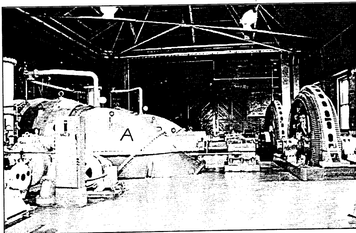
Figure 35. Drainage Pumping Station No. 1. View of northern end of interior, showing 12' Wood screw pumps and motors.
