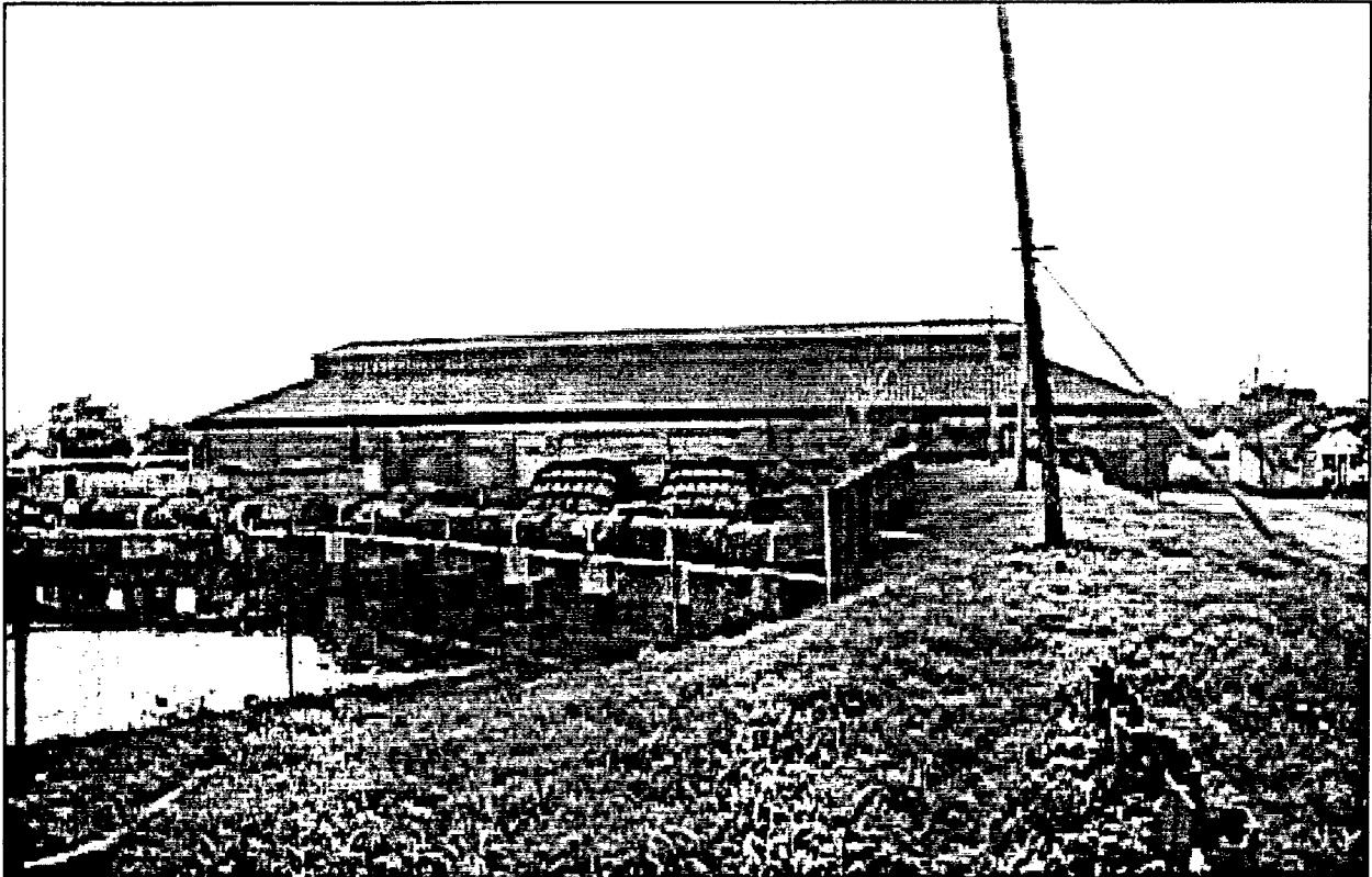
Figure 43. Drainage Pumping Station No. 3, viewed from the northwest. Discharge basin and discharge pipes of 14' Wood screw pumps are visible.
