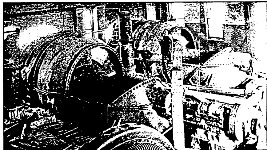
Figure 24. Interior view of Drainage Pumping Station No. 1, showing two 12' Wood screw pumps during installation, ca. 1914-1915 (from Sewerage & Water Board 1914).
