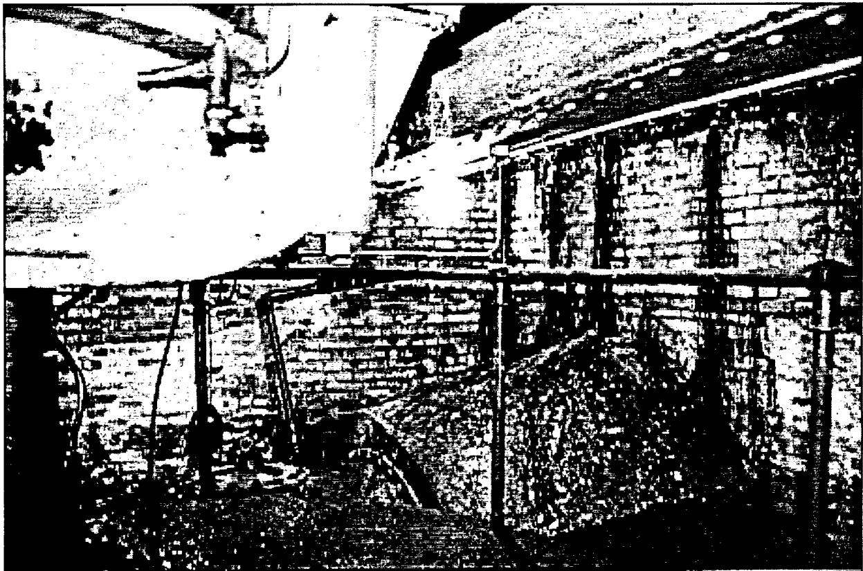
Figure 20. Vertical centrifugal pump pit, showing top of discharge pipe at right. These original pump pits, dating to 1897-1903, have been altered or eliminated at all stations except at Drainage Pumping Station No. 7, shown here.
