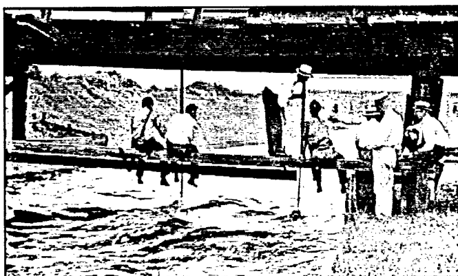
Figure 28. Testing of the 12' Wood screw pumps at Drainage Pumping Station No 1 (background), ca. 1915. Pitot tubes have been placed in the Metairie Relief Canal to measure the velocity of flow. This data was used to calculate the efficiency of the pumps. Tulane engineering students are holding the tubes while engineers record data (from Sewerage and Water Board 1915).
