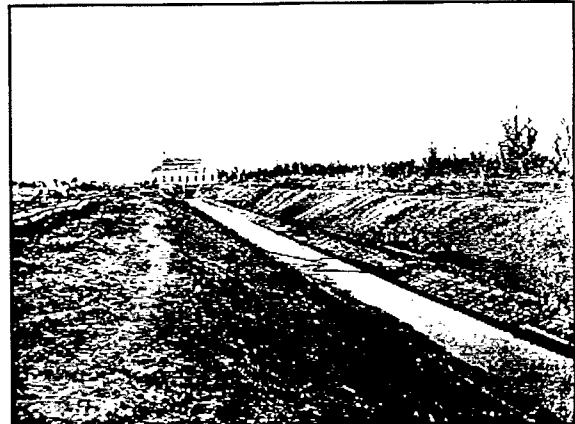
Figure 70. Melpomene Outfall Canal, 1906. The canal was timber lined and the banks graded, 1905-1906. Drainage Pumping Station No. 1 is in the background (From Sewerage & Water Board 1906a).
