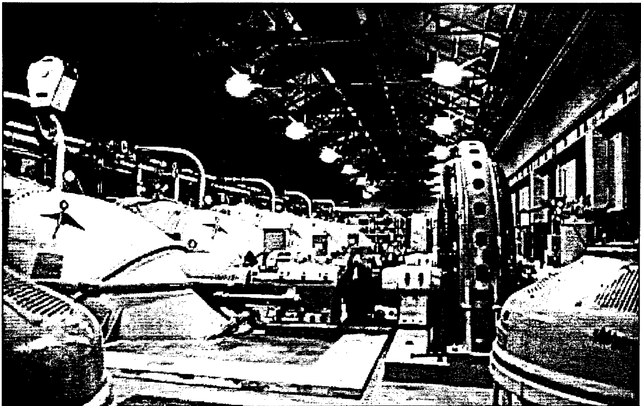
Figure 60. Drainage Pumping Station No. 6. View of interior looking east; in the foreground are 250 cfs vertical centrifugal pump motors. The remainder of the pumps are Wood screw pumps; in the foreground are two 12' pumps, and in the background are four 14' pumps.
