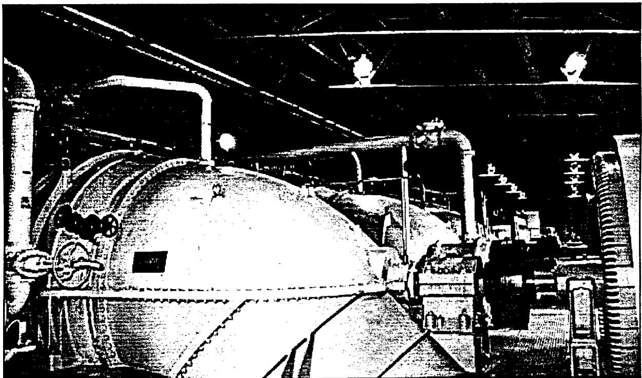
Figure 37. Drainage Pumping Station No. 1. View of interior looking south from central portion of building. Foreground, prototype Wood screw pump on display; center, 250 cfs vertical screw pump motors.
