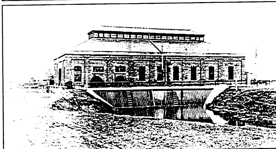
Figure 14. Drainage Pumping Station No. 3 as originally constructed, 1909 (from Sewerage & Water Board 1909).
