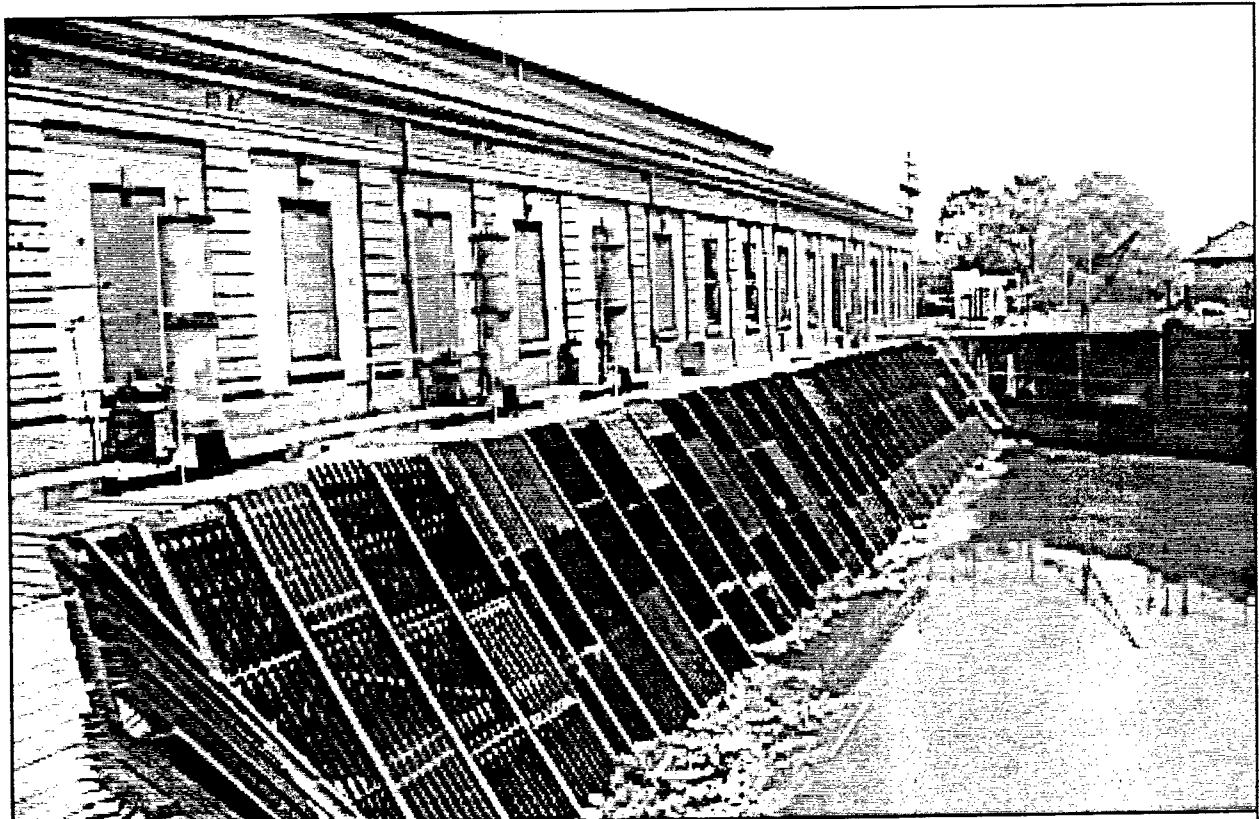
Figure 63. Drainage Pumping Station No. 7. Viewed from the northeast, showing trash screen and hydraulic sluice gate mechanisms.
