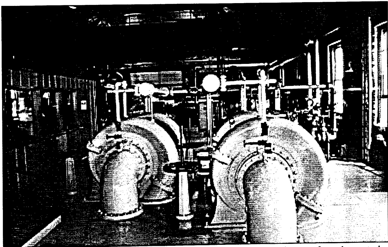
Figure 46. Drainage Pumping Station No. 3. View of interior looking east from the central portion of the building; in the foreground are two horizontal centrifugal constant duty pumps.
