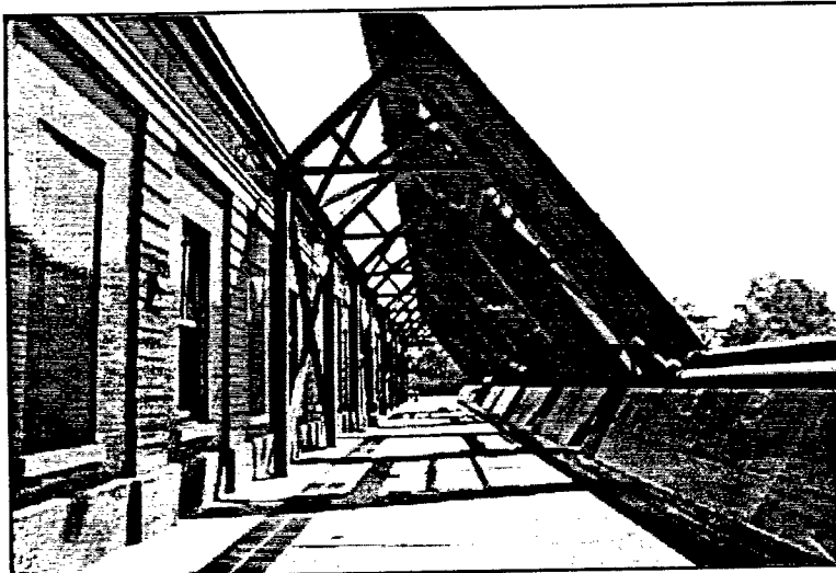
Figure 57. South facade of Drainage Pumping Station No. 6.
