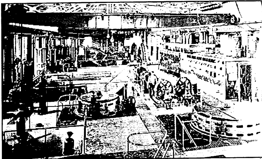
Figure 26. Interior view of Drainage Pumping Station No. 1 after installation of 12' Wood screw pumps and electrical equipment, ca. 1915. The Wood pumps are visible in the rear, the switchboard to the right, and in the foreground, the motors for the vertical screw pumps originally installed in the station ca. 1903-1904 (from Sewerage & Water Board 1915).
