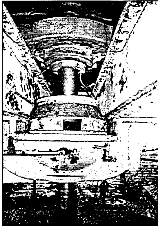
Figure 19. Lower portion of vertical centrifugal pump motor and drive shaft, of the type originally installed in Drainage Pumping Stations Nos. 1, 6, and 7, 1897-1903. Photographed at Drainage Pumping Station No. 7.
