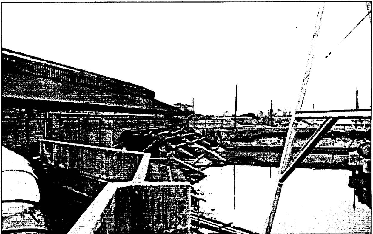
Figure 44. Drainage Pumping Station No. 3. View of discharge basin; 12' Wood pump at left, 14' Wood pumps at right (west) end of the station.
