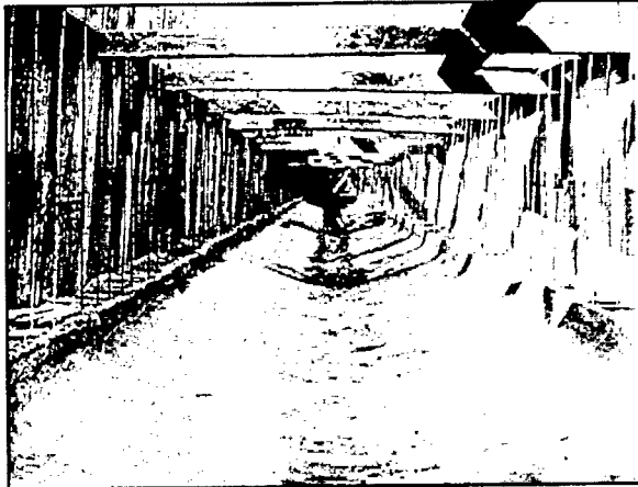
Figure 69. Interior of the Hagan Avenue Canal, shown during construction, ca. 1906. This concrete-lined and covered canal was constructed 1904-1906 (from Sewerage & Water Board 1906a).
