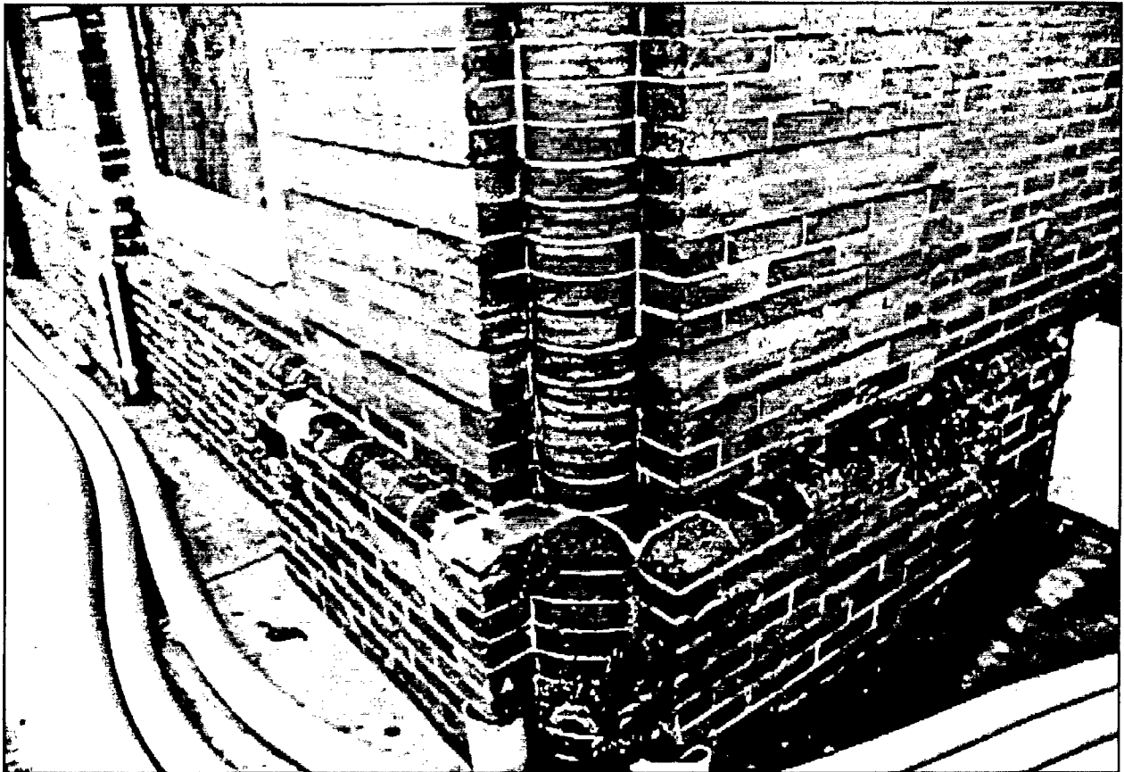
Figure 92. Drainage Pumping Station No. 1. View of lower portion of northwest corner of building, showing special round bricks and pilaster bases at corner.
