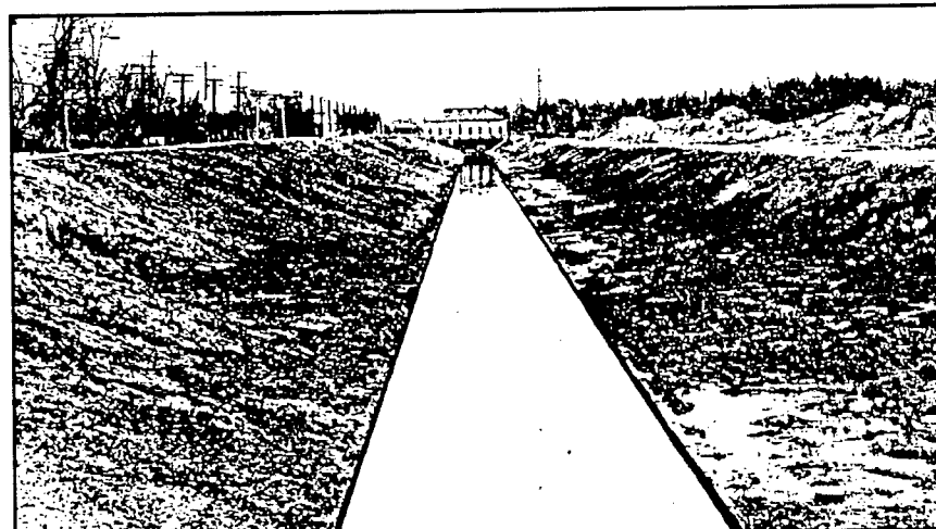
Figure 78. Lower end of the Metairie Relief Canal, approaching Pumping Station No. 6, 1914 (from Sewerage & Water Board 1914).
