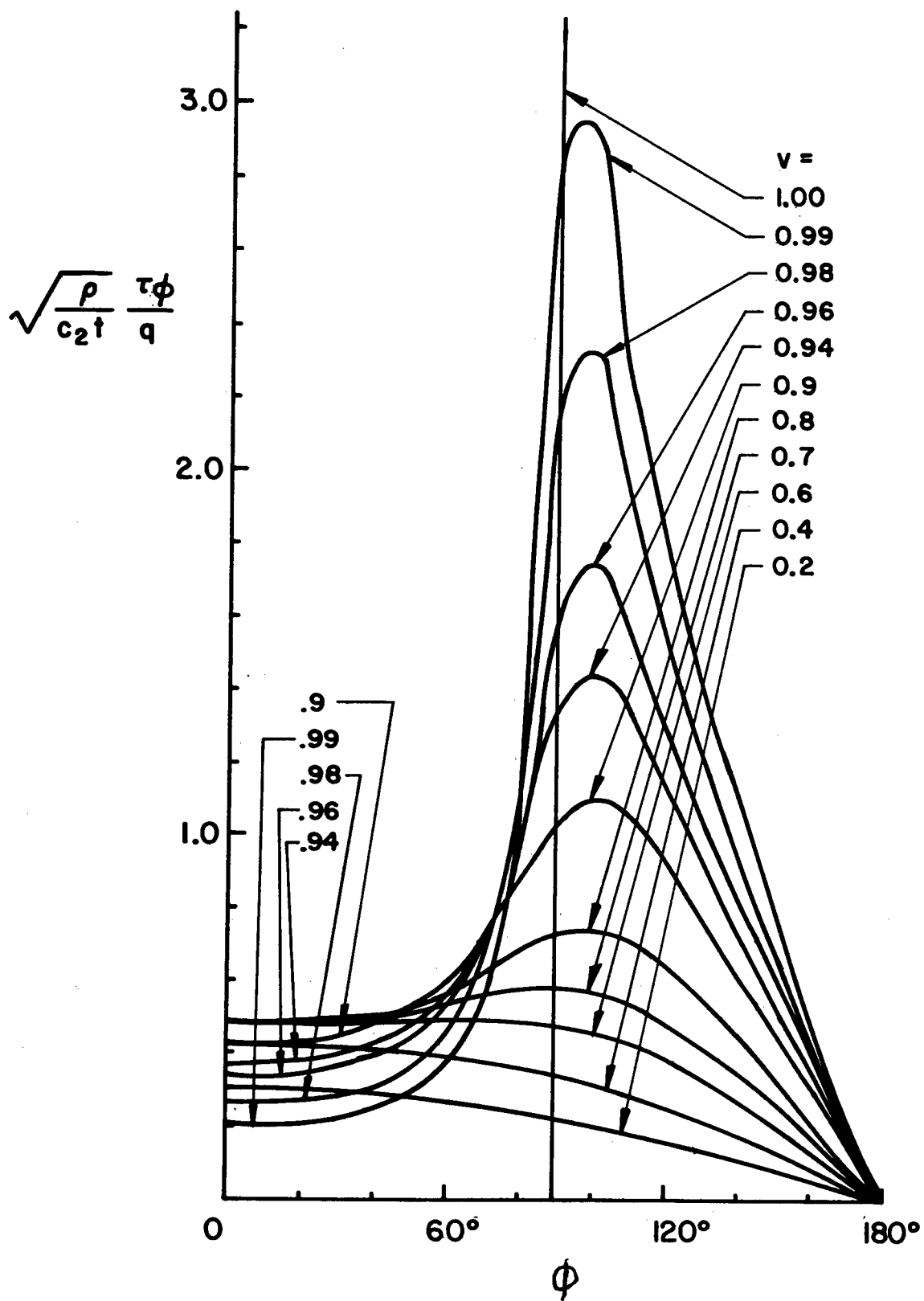
FIGURE 14 - ANGULAR VARIATION OF SHEAR CLEAVAGE STRESS
