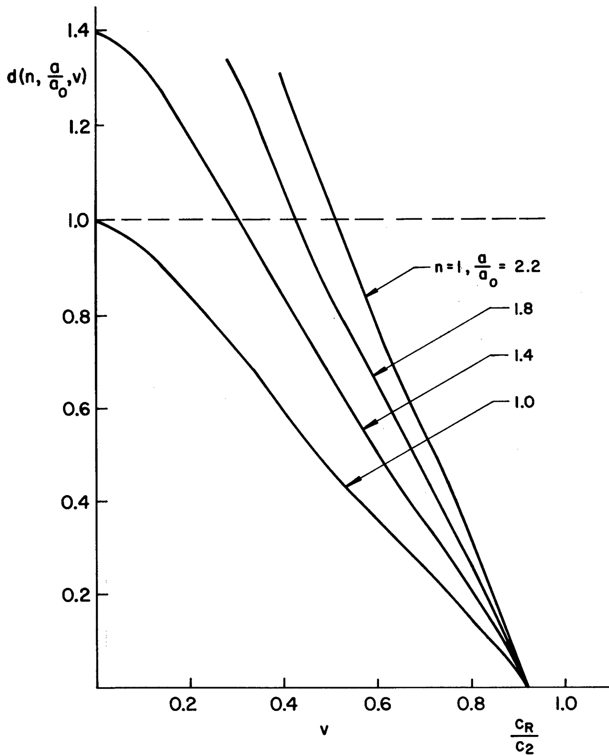
FIGURE 8 - ENERGY AVAILABLE FOR FRACTURE ACCELERATION
