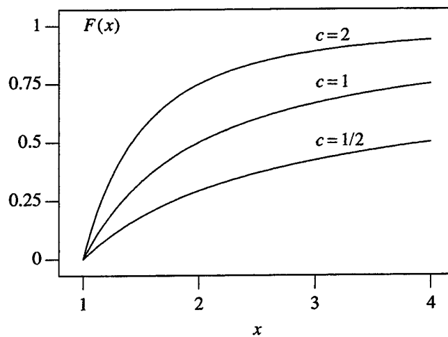
Figure 40. Pareto Distribution Functions.
