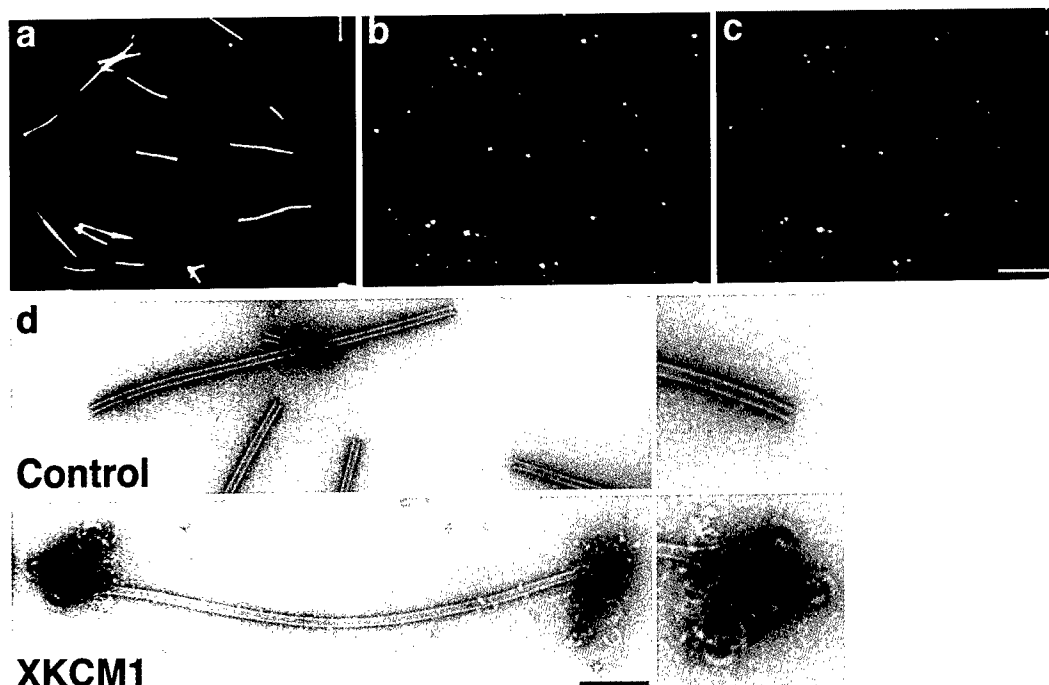
Figure 5. Targeting and Accumulation of XKCM1 at GMPCPP MT Ends in 5 mM MgAMPPNP
