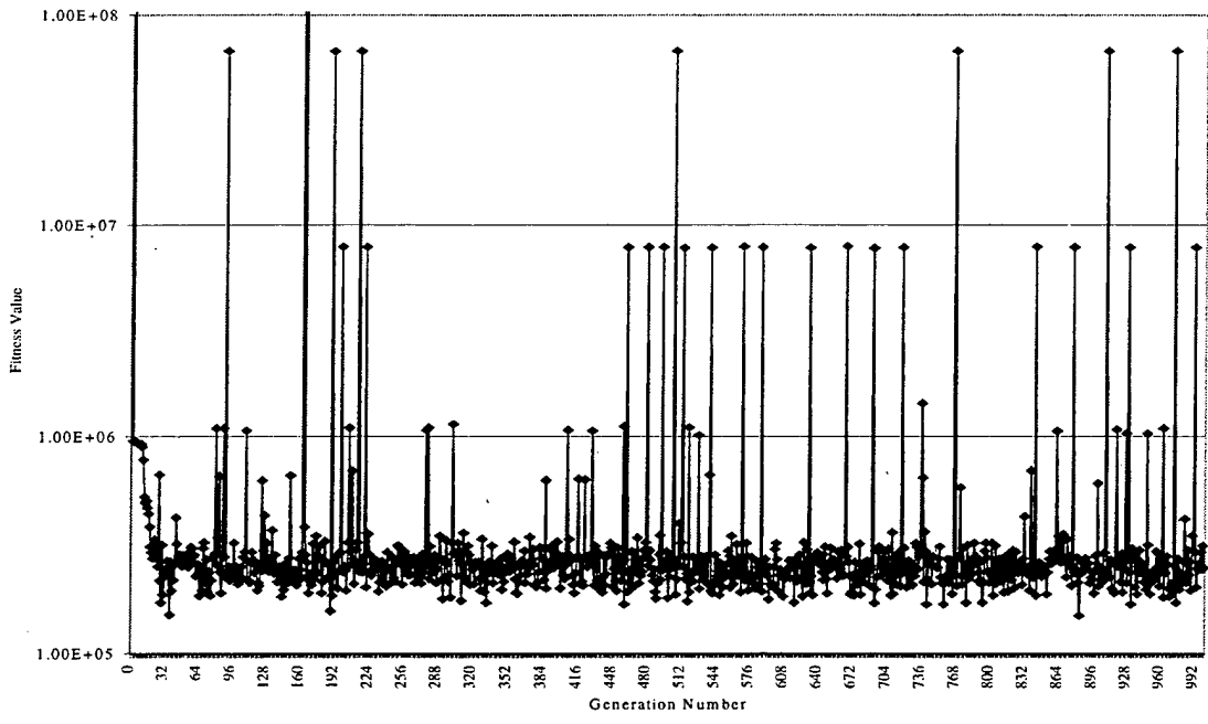
Figure 4. Average Population Fitness for One Run of a Population Size of 20 with a Probability of Mutation of 0.001
