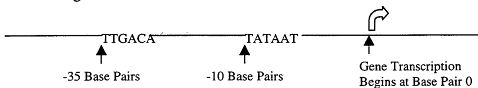
Figure 23. Promoter Consensus Sequences
