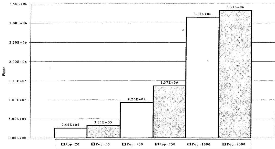
Figure 5. Average Fitness Values with a Probability of Mutation of 0.001
