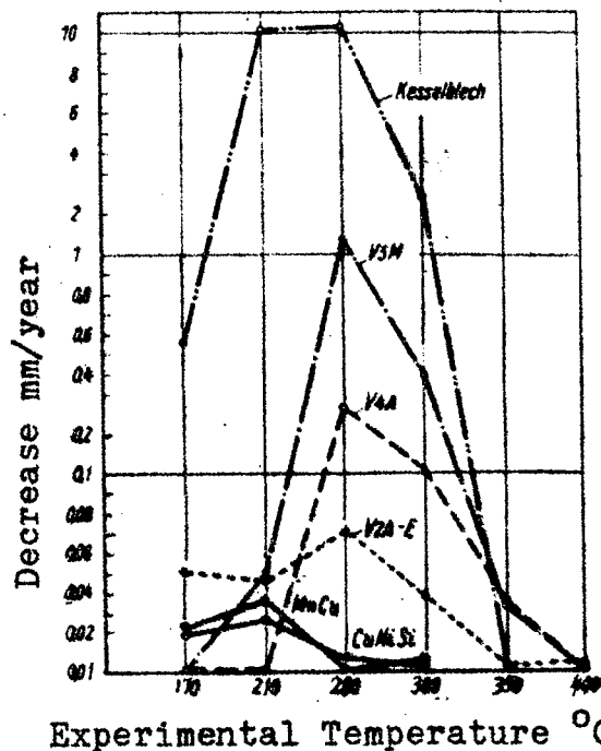
Figure 8 Experiments with Carbon Monoxide Effect on Various Steels at 250 atmospheres Absolute Pressure
