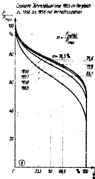
Planned Annual Curve 1965 Compared to 1956-8 (Relative Figures)
