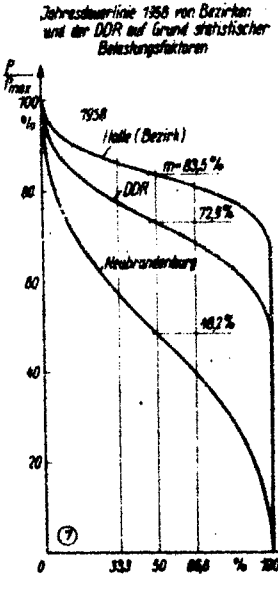
Annual Curve of Districts and GDR Based on Statistical Maximum Load Factors by 10 Percent
