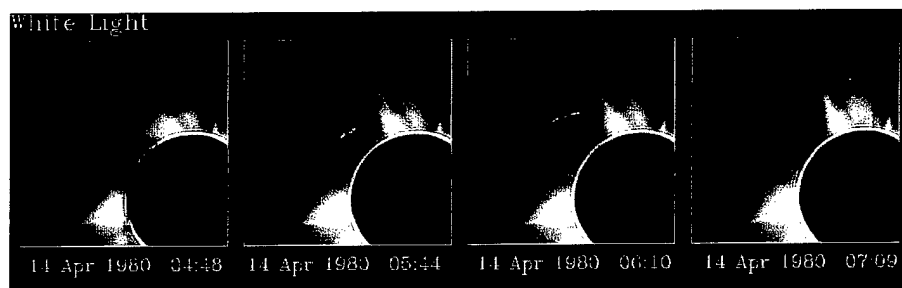
(Courtesy of High Altitude Observatory, National Center for Atmospheric Research.)
