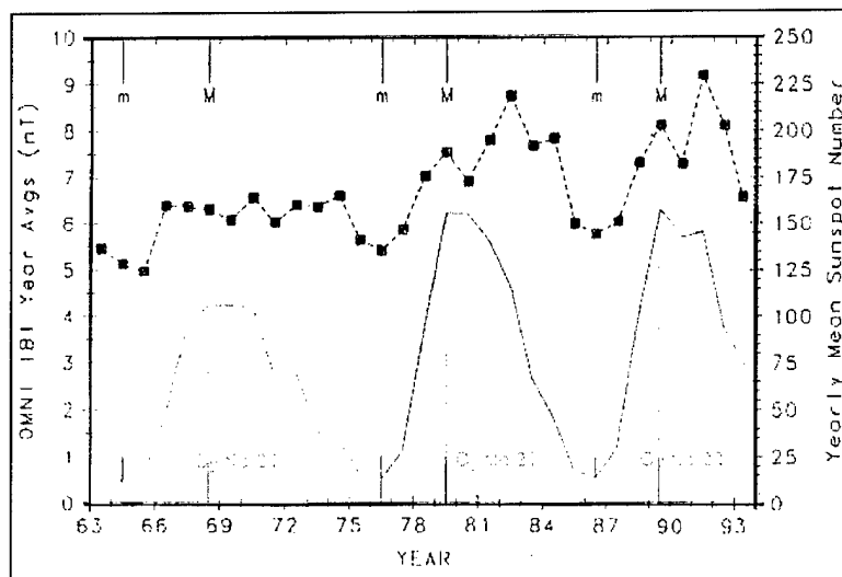
Figure 6.11. Composite of Yearly Averages of the Magnitude of the Interplanetary Field and Sunspot Numbers, 1963 to 1993
