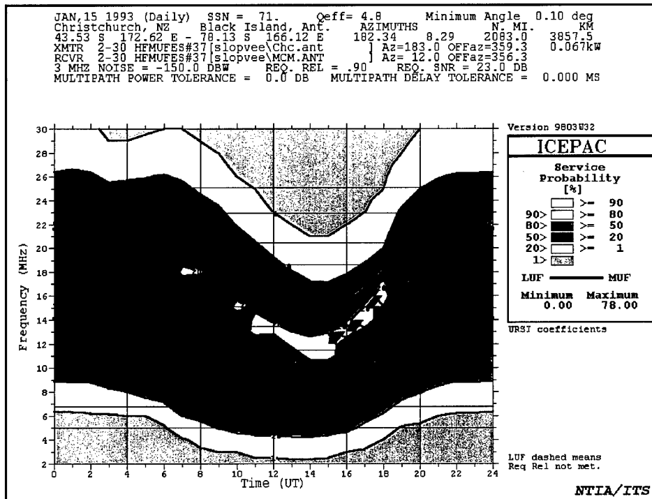
Figure 7.4. Christchurch-to-Black Island Service Probability
