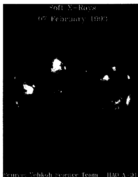
(Courtesy of Yohkoh Science Team.)
