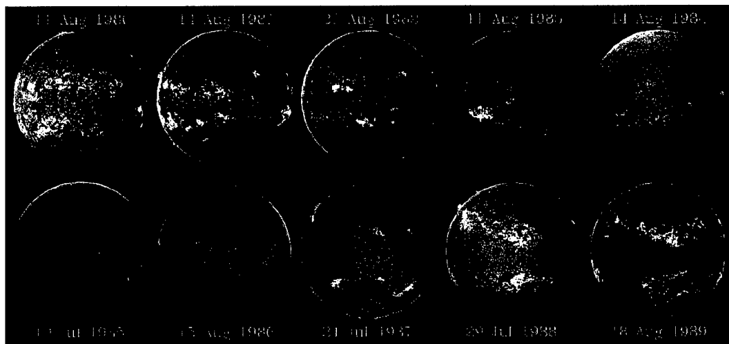
(Courtesy of Space Environmental Laboratory, National Aeronautic and Oceanographic Administration)
