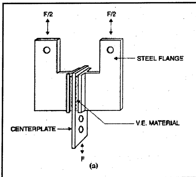
Figure 10. Flange-centerplate connection.
