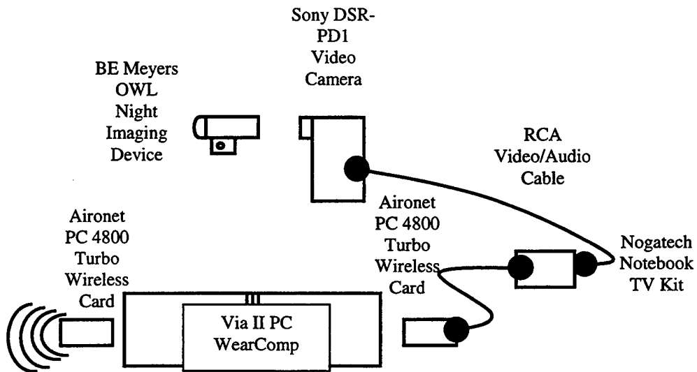
Figure 3.10 The VIEW System Diagram.
