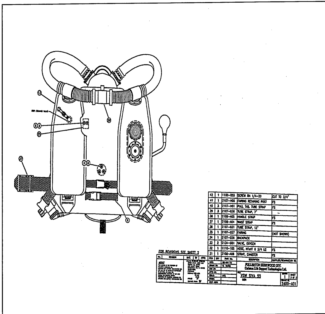
Figure 1. Schematic of Sherwood-Fullerton Siva 55-VSW UBA Counterlung Arrangement.
