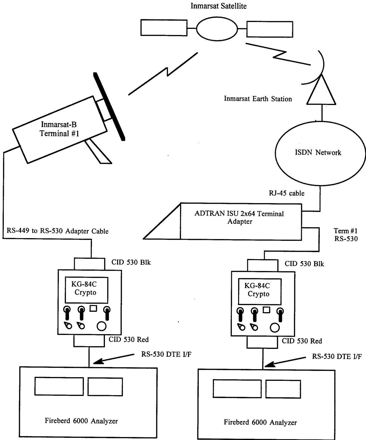
Figure 12 Inmarsat Compatibility Test with Two KG-84C Cryptos
