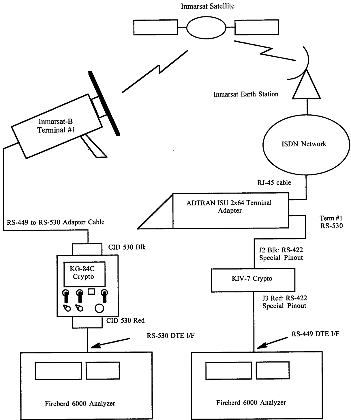
Figure 11 Inmarsat Compatibility Test with KG-84C and KIV-7 Cryptos
