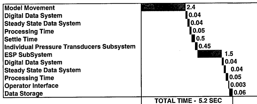
Fig.8. Current data cycle process and times.
