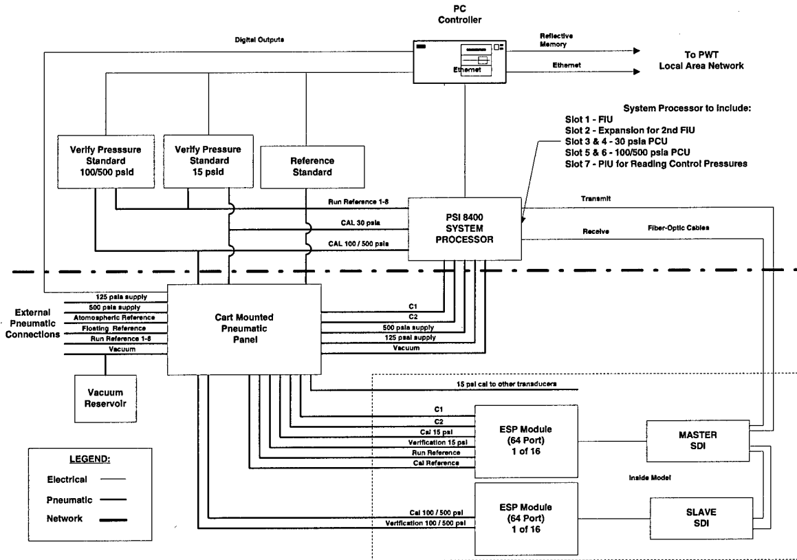
Fig. 6. PSS block diagram.
