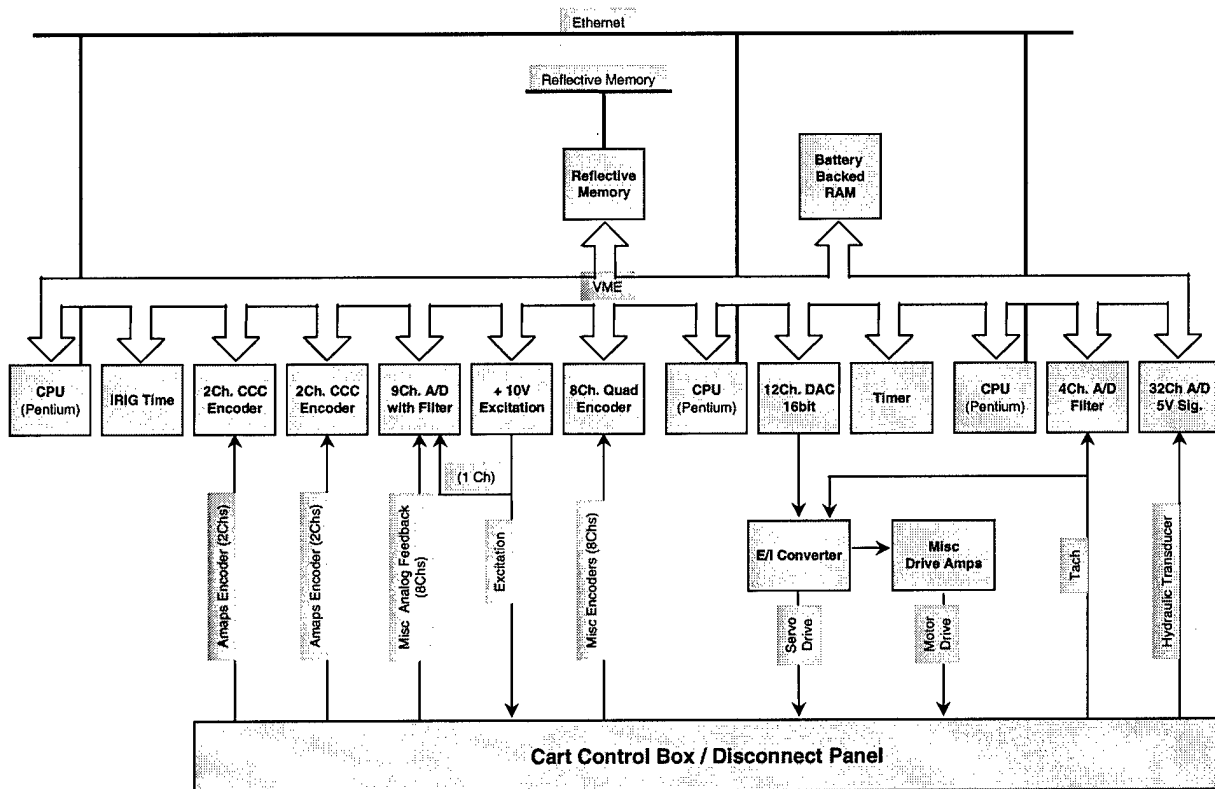
Fig. 7. Test article control block diagram.
