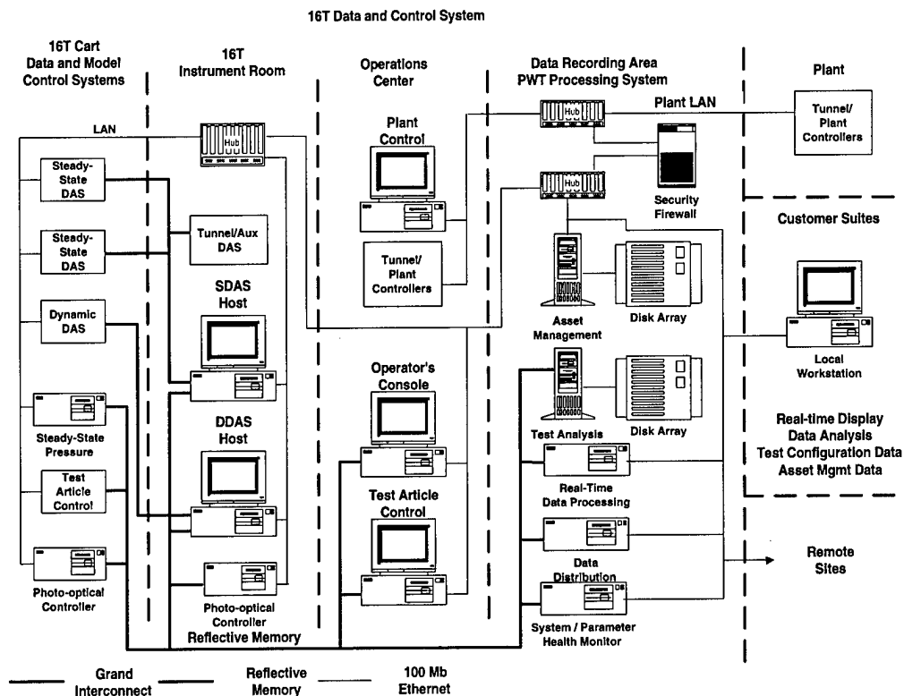
Fig. 4. Data Acquisition and Processing System (DAPS).
