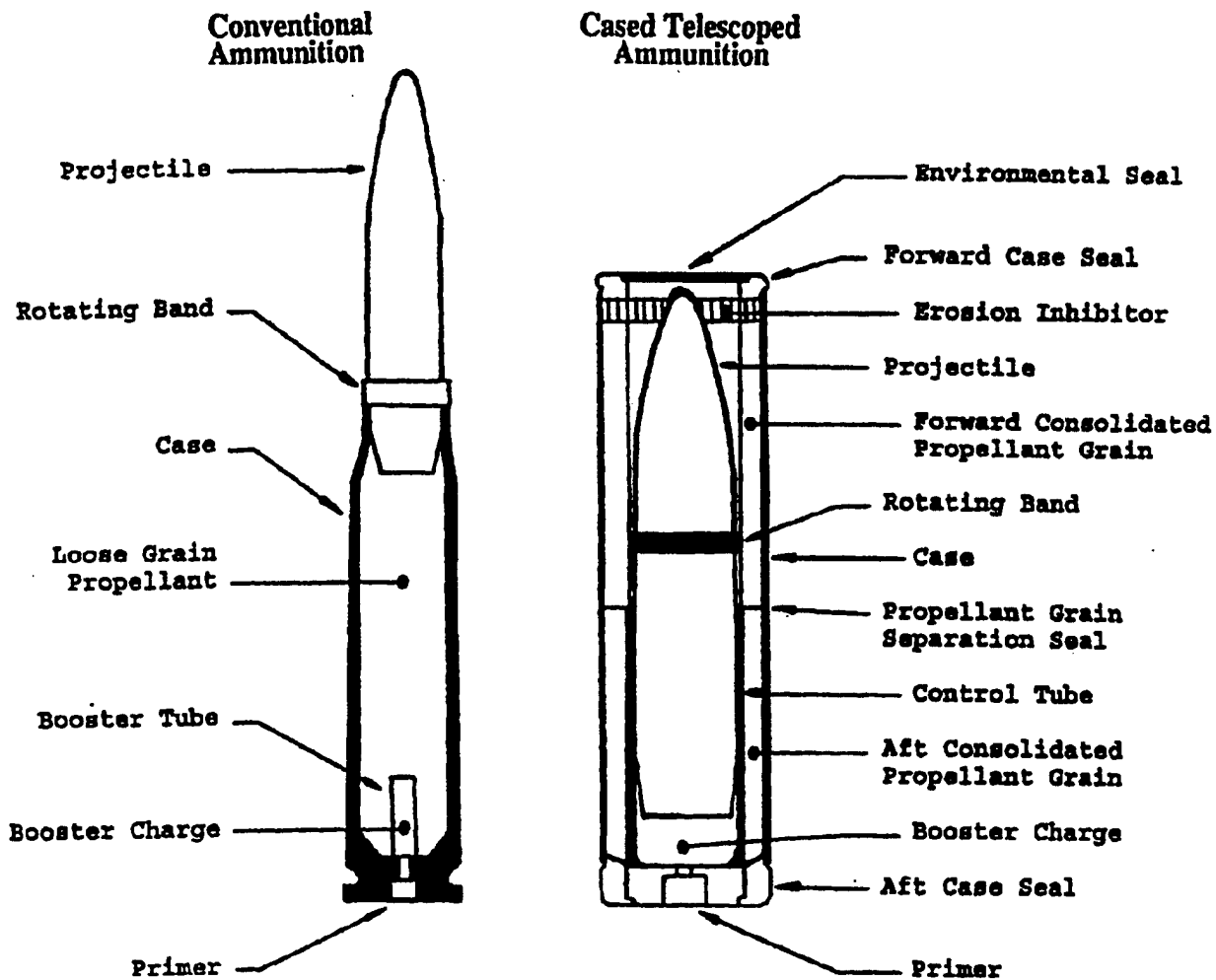
Schematic Comparison of Cased Telescoped Ammunition and Conventional Ammunition
