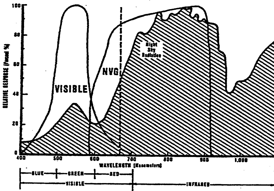
Figure 9: Moonless night spectral composition (MAWTS-1, 1995)
