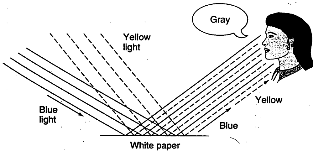
Figure 6: Additive mixtures for blue light and yellow light. (Matlin & Foley, 1997)
