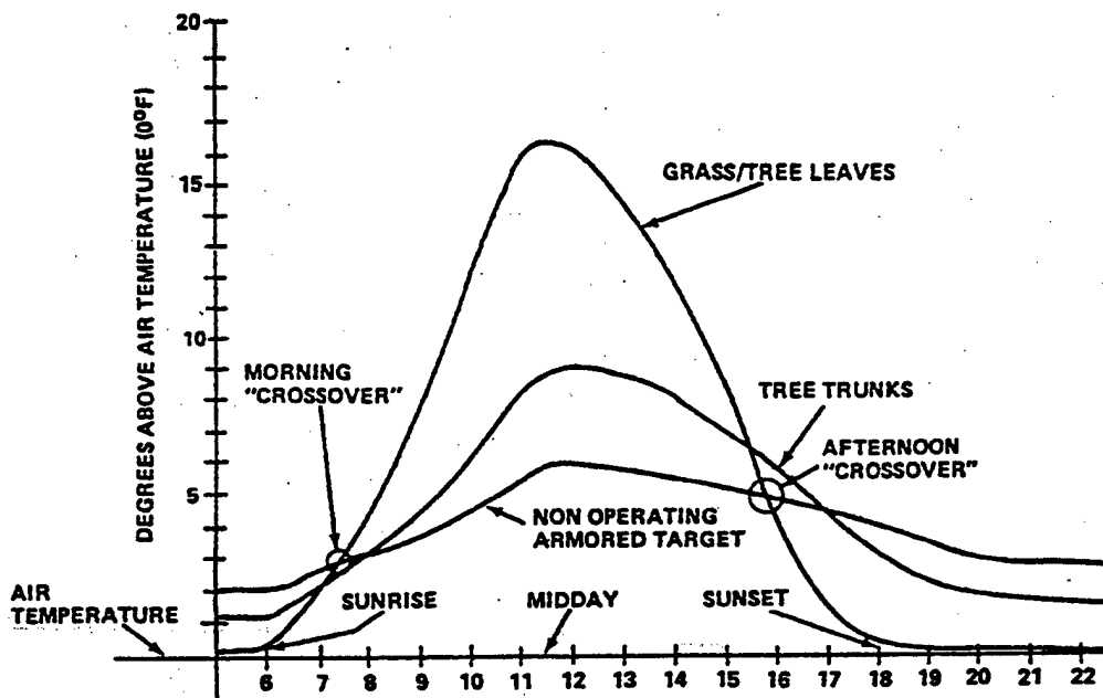
Figure 10: Diurnal cycle example (MAWTS-1, 1995)
