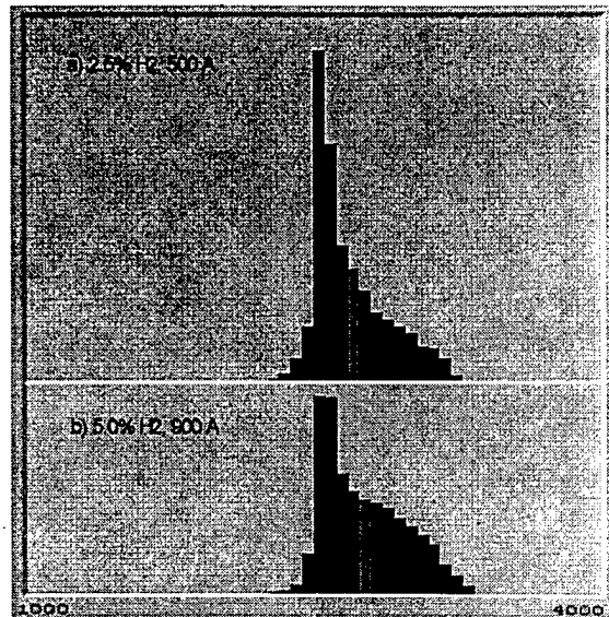
Figure 2. Temperature distributions of yttria-stabilized zirconia powders during plasma spraying. The peak corresponds to the melting point of the material.
