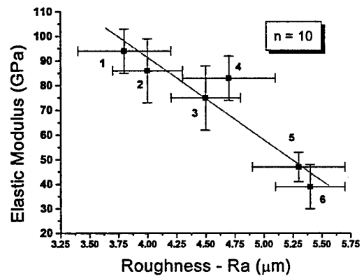
Figure 6. Elastic modulus-roughness relationship in nanostructured coatings.
