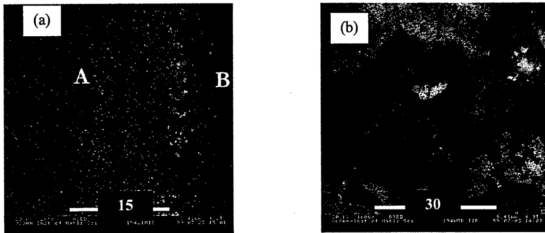
Figure 3. Wear track surface of N195 sliding against a Si 3 N 4 ball under a force of 4.9 N with 20,000 rotations. (a) before and (b) after ultrasonic cleaning.
