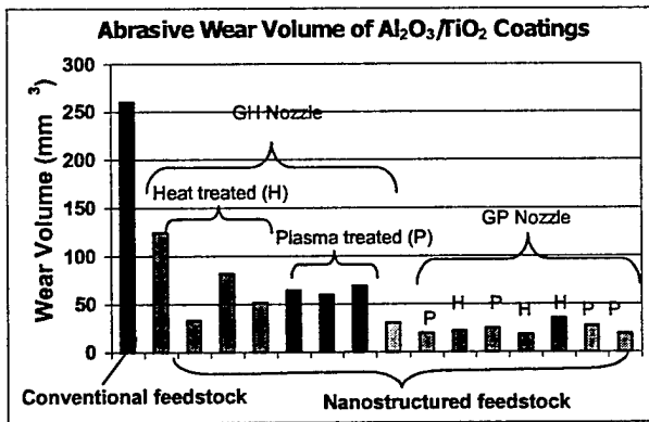
Figure 1. Wear property comparisons, nanostructured \text{Al}_2\text{O}_3/\text{TiO}_2 vs. conventional \text{Al}_2\text{O}_3/\text{TiO}_2
