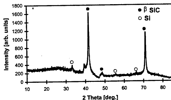
Figure 4. XRD pattern of SiC produced from chlorocarbodisilane mixture ( P=22\text{kW} , p=20\text{kPa} , d=170\text{mm} , stainless steel substrate).
