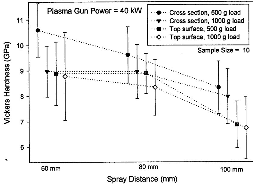
Figure 2. Change of microhardness of ATZ coating sprayed at different stand off distances.
