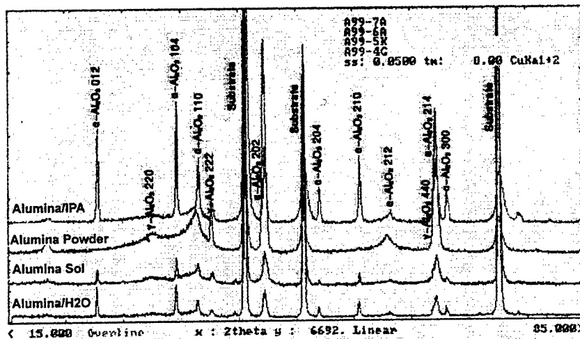
Figure 2. XRD scans of the as-sprayed alumina coatings
