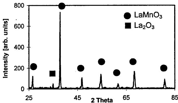
Figure 3. X-ray diffraction pattern of a TPCVD perovskite coating
