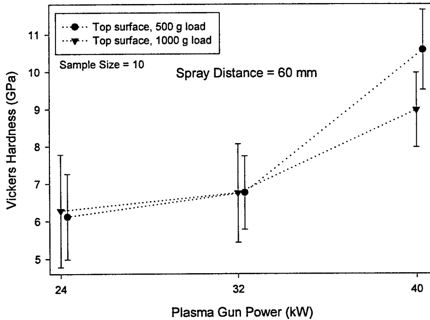
Figure 3. Change of microhardness of ATZ coatings sprayed using different plasma power at a 60 mm standoff distance.
