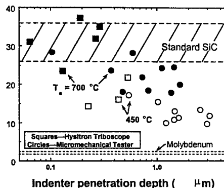
Figure 1. Measured hardness versus nanoindenter penetration depth of two silicon carbide films deposited at a substrate temperature of either
