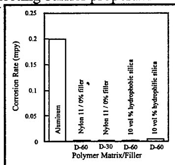
Figure 1. Corrosion rates of Al substrates coated with nylon 11 D-30 and D-60 with different types of nano-sized silica filler [no presoak].
