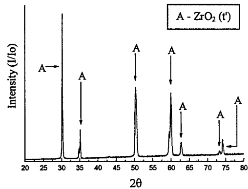
Figure 4. XRD pattern of the nanostructured coating.
