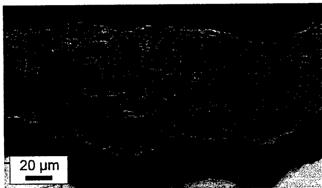
Figure 1. Optical micrograph of a cross-section of a suspension plasma sprayed perovskite coating
