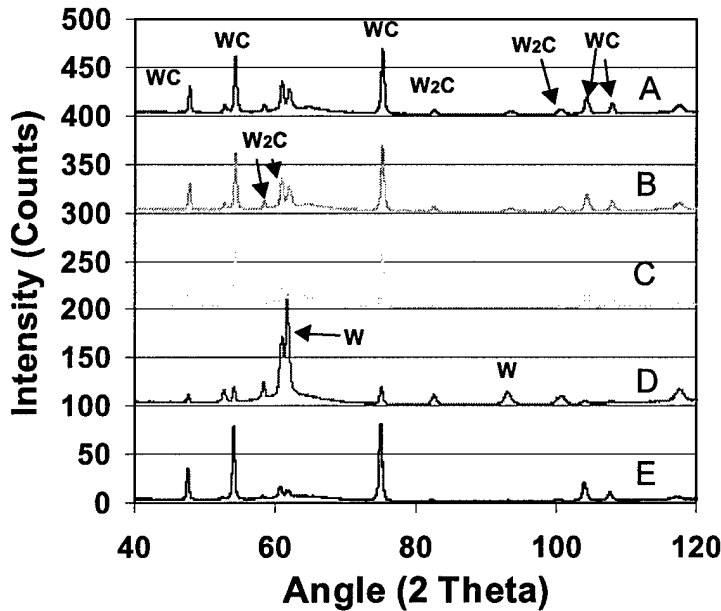
Figure 1. XRD analysis for the 5 coatings tested
