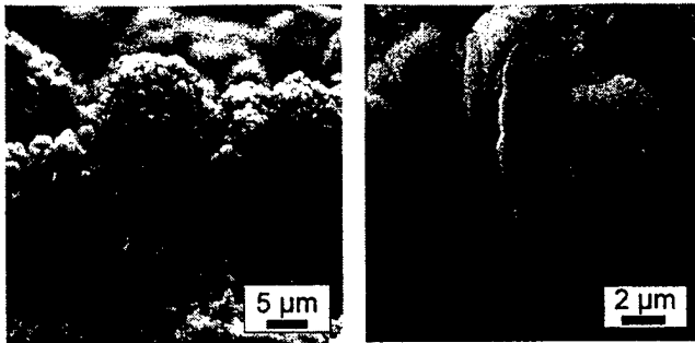
Figure 2. SEM images of fracture sections of TPCVD perovskite coating
