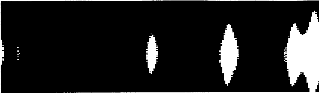
Figure 2. Argon Spectrum
