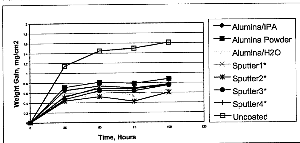
Figure 3: Oxidation behavior of the alumina coatings
