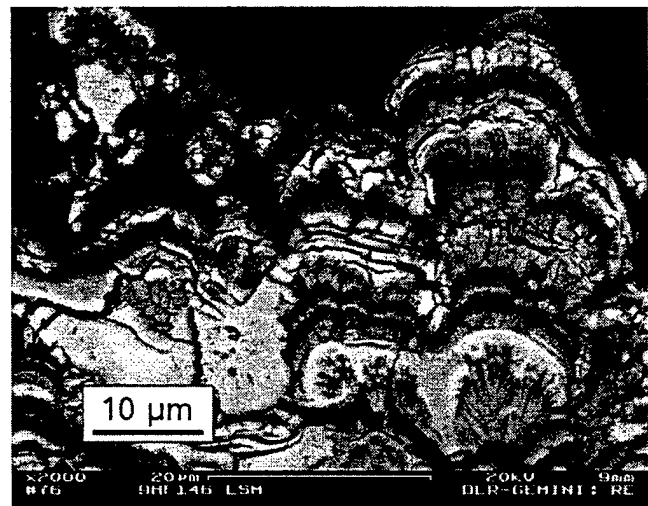
Figure 4. SEM image (back scattered electrons) of a cross section of a TPCVD perovskite coating
