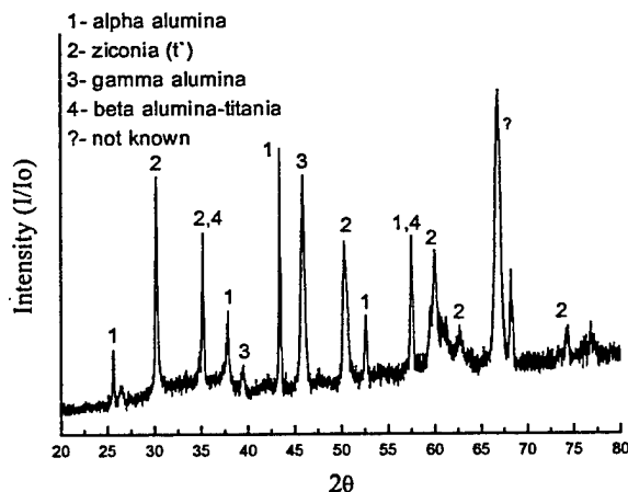
Figure 1. X-ray diffraction analysis of alumina-titania-zirconia coatings.
