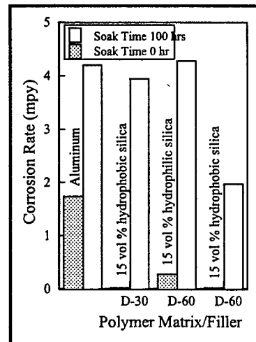
Figure 2. Corrosion rates of Al substrates with intentional damage and 2 soak times.
