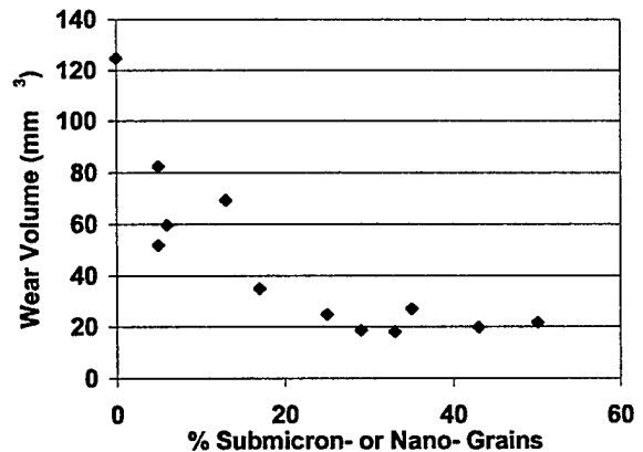
Figure 2. Plot of wear resistance vs. % of nano- or submicron structure.
