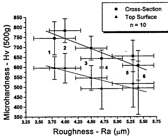
Figure 5. Microhardness-roughness relationship in nanostructured coatings.
