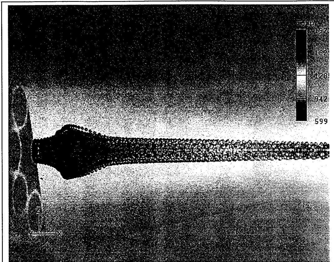
Figure 4. Particle flow in Metco DJ-2700 gun. Injection and nozzle area.
