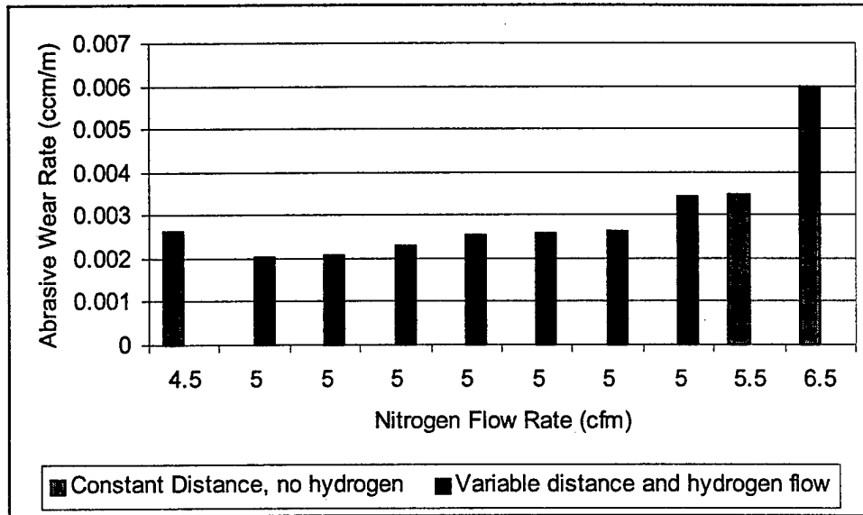
Figure 4. Effect of HEPS parameters on dry-sand-rubber-wheel wear rates for nano-sized WC[12%Co] coatings produced using solid sphere agglomerated powder feedstock.
