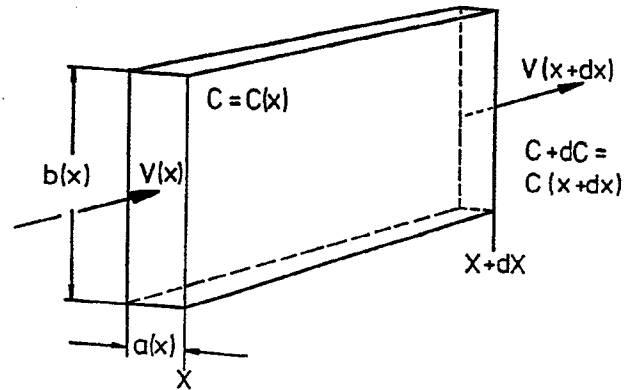
Figure 1: Part of a fracture along the percolating pathway at distance x from input between x and x + dx . The concentration increases along the distance by dc .
