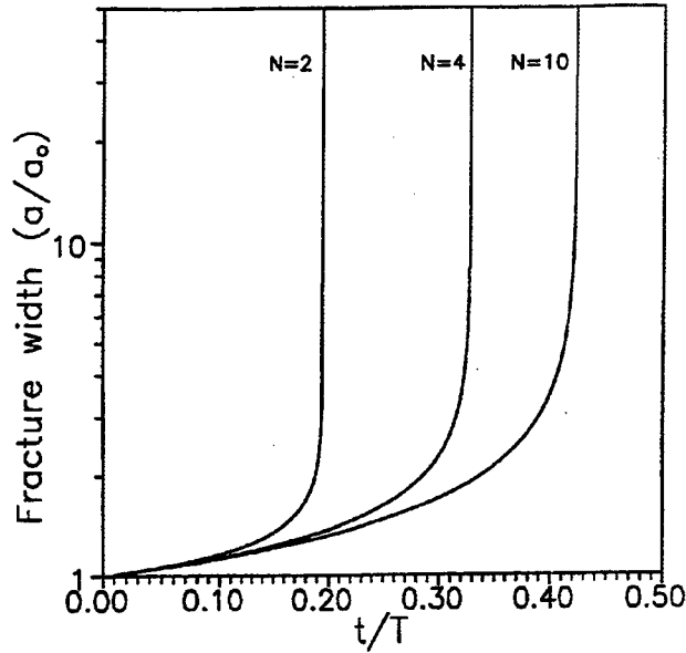
Figure 5: Evolution of the width of the idealized fracture as a function of time. The width is in units of a_0 and the time in units of T (cf. eq. 15a). The numbers on the curves give the order of the kinetics acting at the exit. Note that T depends on n . Therefore the time scales are different for n = 10, 4 , and 2 . The evolution of the fracture width is calculated from eq. 18 ( M = 10^4 and \Delta a/a_0 = 10^{-2} ).
