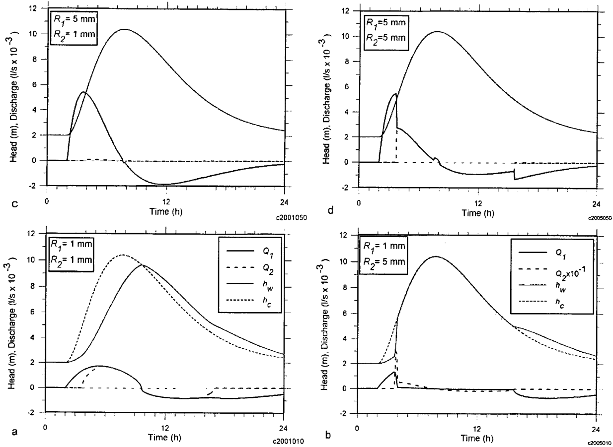
Figure 11: Tandem link results. (a) Tandem link results for R_1 = 1 \text{ mm} , R_2 = 1 \text{ mm} . (b) Tandem link results for R_1 = 1 \text{ mm} , R_2 = 5 \text{ mm} . Note: Q_2 is 10x axis scale. (c) Tandem link results for R_1 = 5 \text{ mm} , R_2 = 1 \text{ mm} . (d) Tandem link results for R_1 = 5 \text{ mm} , R_2 = 5 \text{ mm} .
