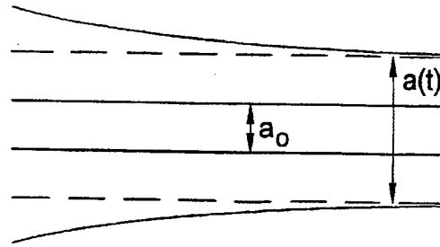
Figure 4: Profile of a fracture with initial width a_0 at time t after onset of karst evolution (solid line). The dashed line illustrates the profile that would have developed if the dissolution rate at the exit had been acting along the entire length of the fracture.
