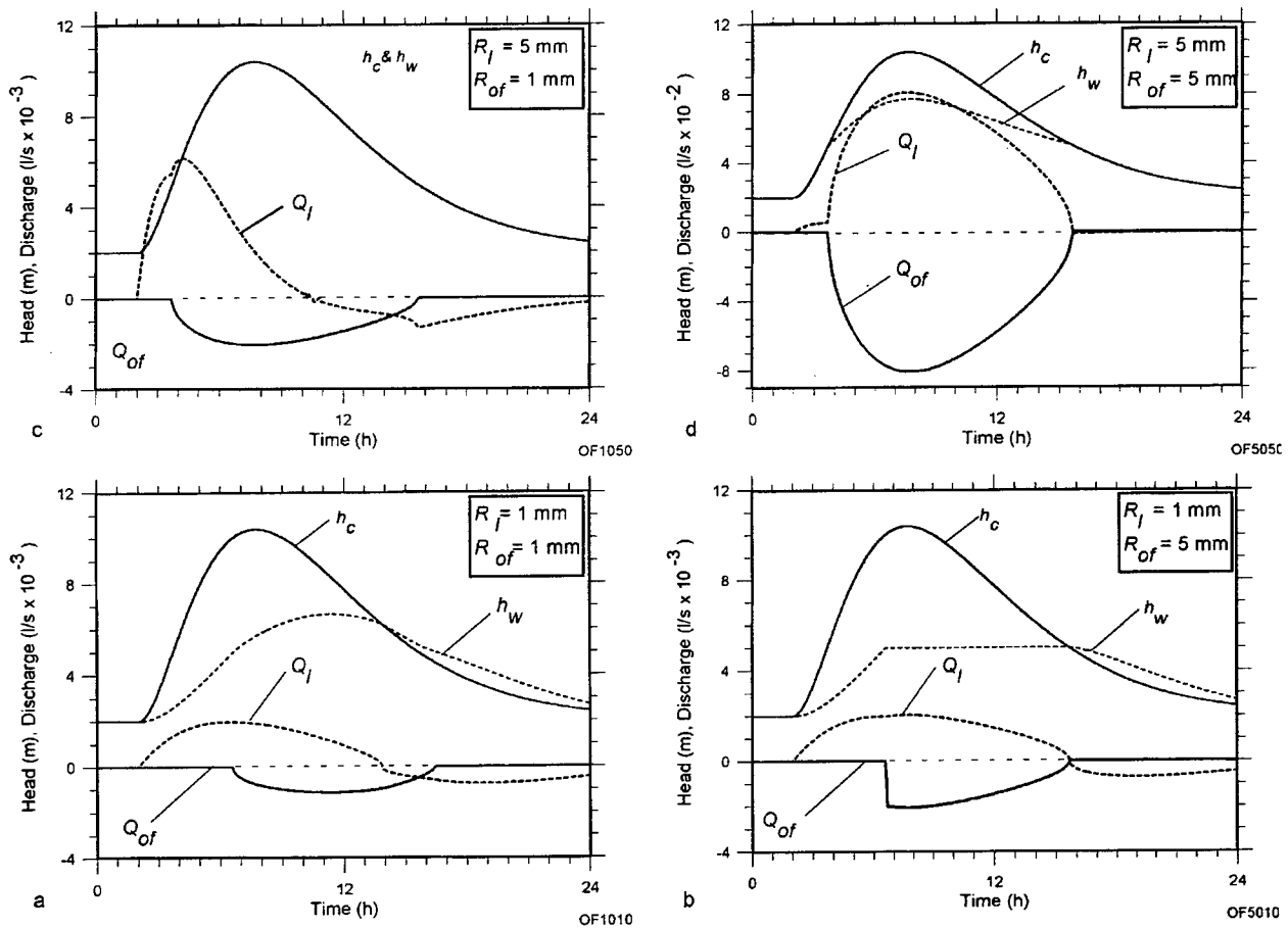
Figure 7: Overflow results: (a) Overflow results for link radius ( R_l ) = 1 mm, overflow radius ( R_{of} ) = 1 mm. (b) Overflow results for link radius ( R_l ) = 1 mm, overflow radius ( R_{of} ) = 5 mm. (c) Overflow results for link radius ( R_l ) = 5 mm, overflow radius ( R_{of} ) = 1 mm. (d) Overflow results for link radius ( R_l ) = 5 mm, overflow radius ( R_{of} ) = 5 mm. (Note discharge scale is an order of magnitude greater than in other graphs.)
