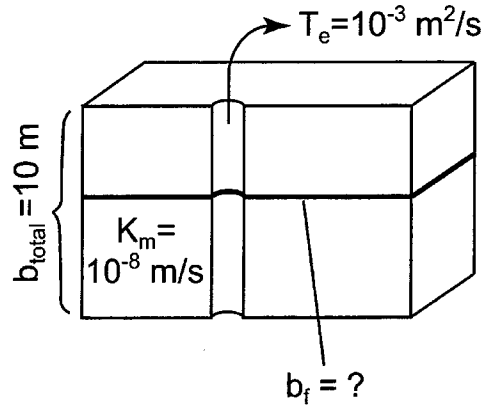
Figure 8: Often, the hydraulic aperture of a fracture intersecting a well is of interest (example 4). Using the transmissivity from a pump test combined with equation (5c), the hydraulic aperture can be determined.
