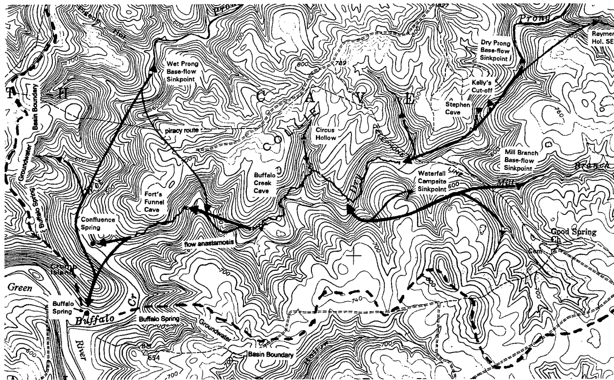
Figure 3: Map of the lower portions of the Buffalo Spring groundwater basin, showing key surface and subsurface features. Solid lines represent hypothesized groundwater flow routes. (1" = 2700')
