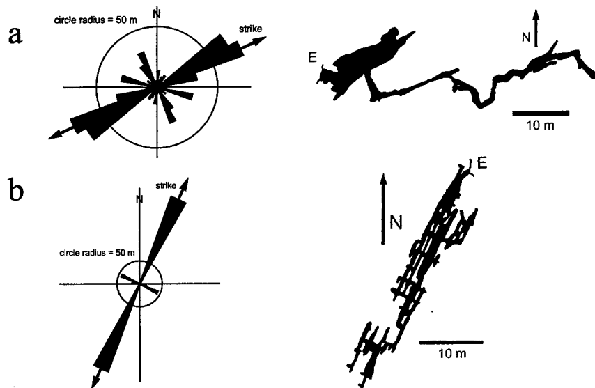
Figure 4: Rose diagrams of passage trends in caves in the Beekmantown Formation, Pennsylvania: (a) Emigs Cave, (b) Goods Cave (both from survey data by B. Smeltzer). The dominant strike-oriented joint patterns are clearly portrayed and provide a rough indicator of anisotropy ratios (see text for details). The outlines of the caves alone are sufficient to portray the preferred directions of groundwater movement.
