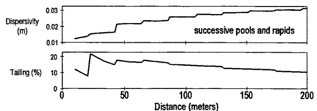
Figure 2: Scale effect on dispersivity and compensation of the tailing along the course of successive pools and rapids (results from the convolution approach based on CFD models).
