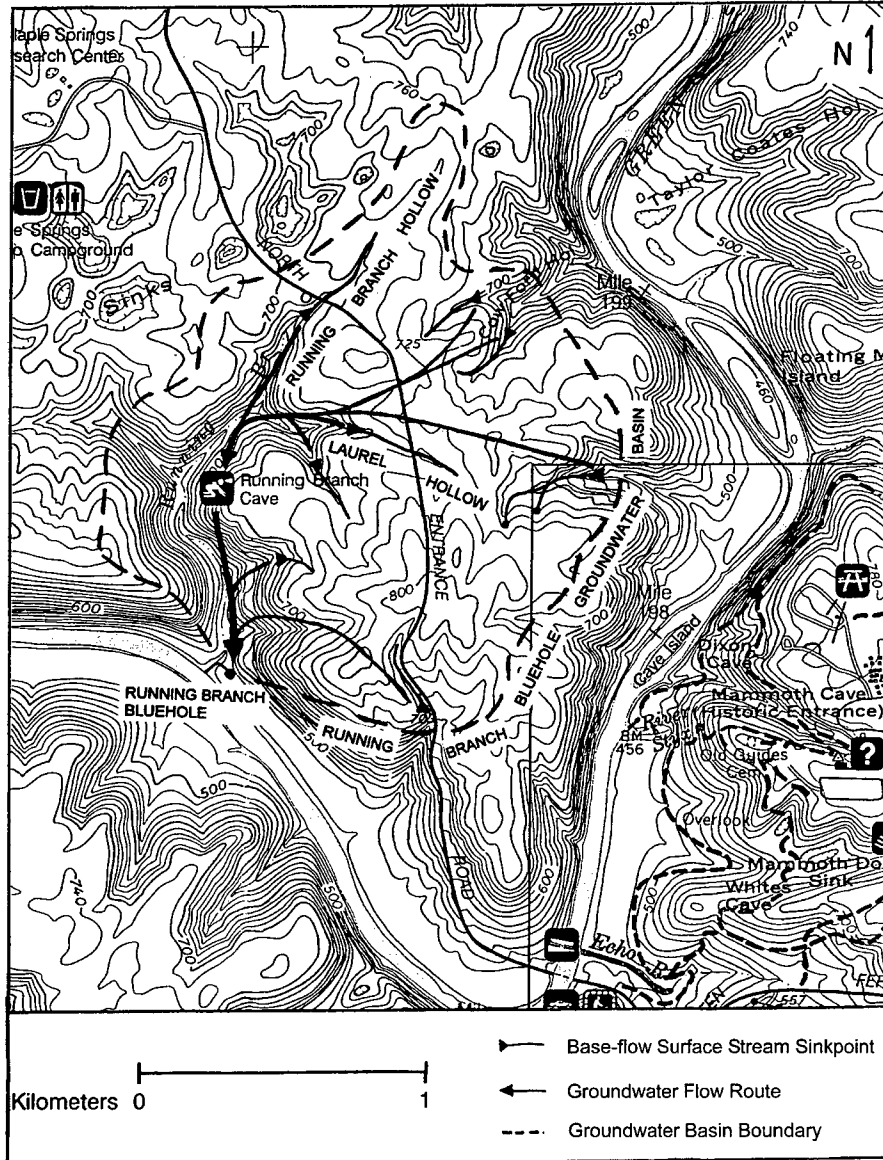
Figure 6: Map of Running Branch Bluehole groundwater basin, showing key surface and subsurface hydrologic features.
