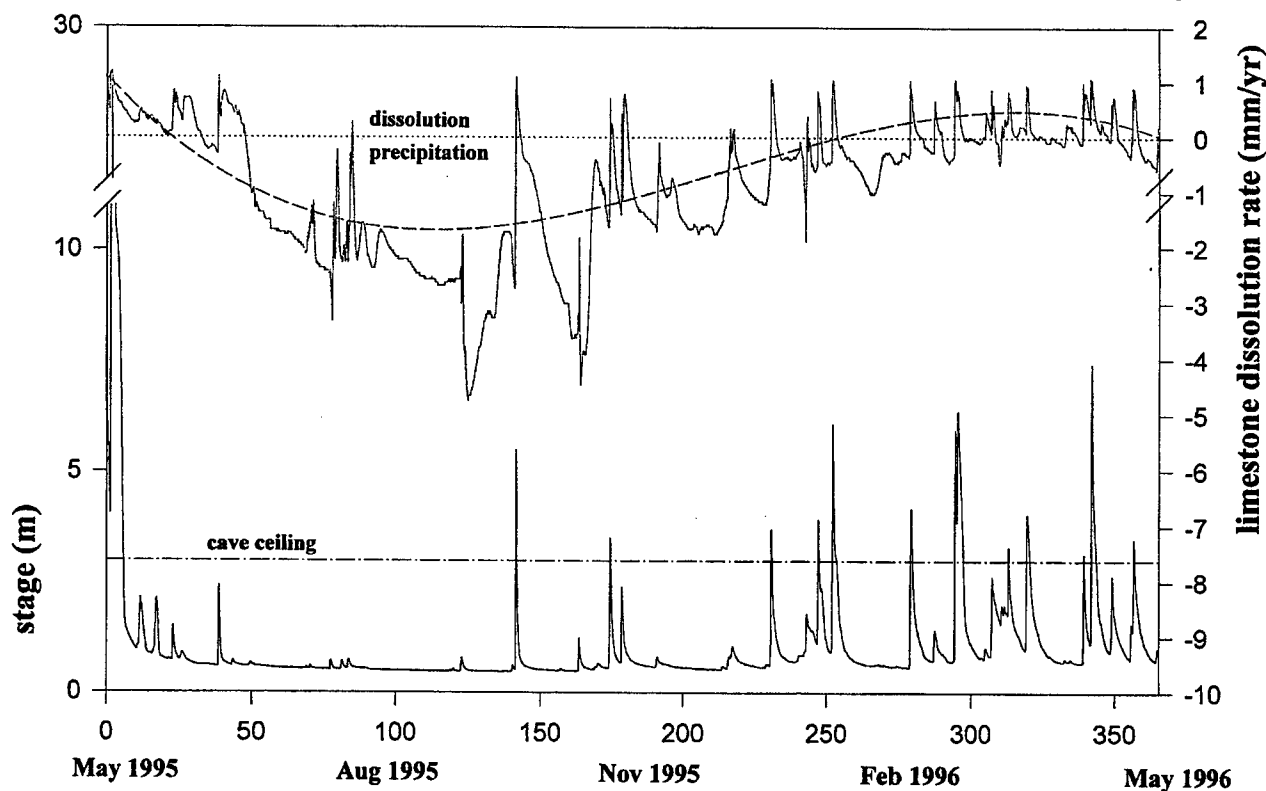
Figure 3: Stage and calculated limestone dissolution rates for 21,473 observations between May 5, 1995 to May 4, 1996 in Logsdon River. Measurements were made with two minute resolution, recorded hourly during static conditions. Rate calculations used the expressions of Plummer et al. (1978). The horizontal line in the bottom figure shows the level of the cave ceiling at the study site, and that in the upper figure indicates calculated equilibrium with respect to calcite dissolution. Negative dissolution rates predict calcite precipitation.
