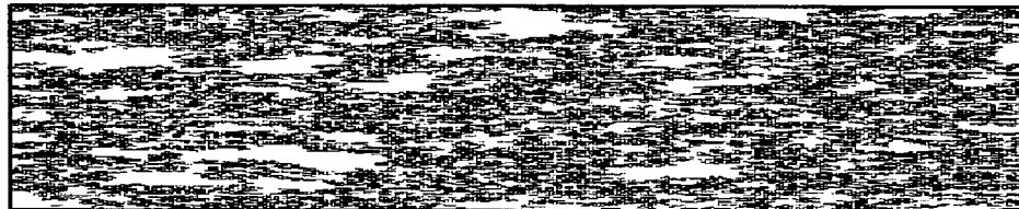
Figure 5b. Plan view of 5.0 m contact depth and horizontal conduit locations - Large scale grid ( x = 5,000 m, y = 1,000 m, z = 7.5 m)
