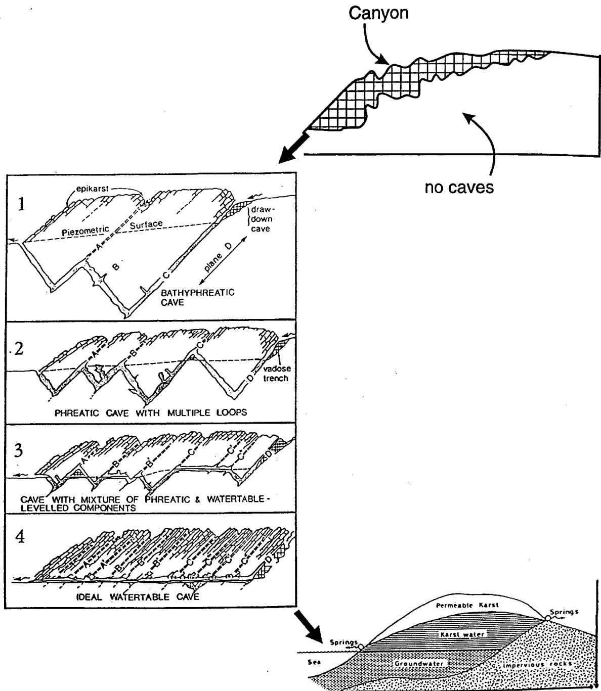
Figure 5: The four-state model of cave system geometrics (Ford 1971 et seq. ) amplified to include: above right State 0, where fissure frequency and/or aperture is too low to permit cavern genesis; below right, State 5, where fissure frequency and/or matrix porosity are too high to permit caves to develop to an enterable scale.
