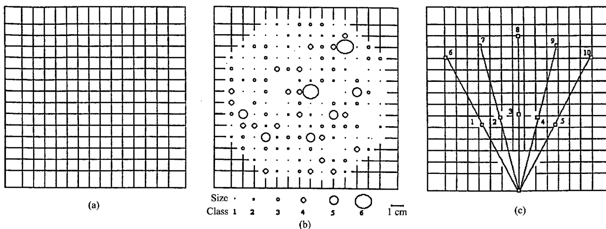
Figure 1: Schematic diagrams (a) of the grid pattern, (b) of the location and size of sinkholes, and (c) of the injection locations,
