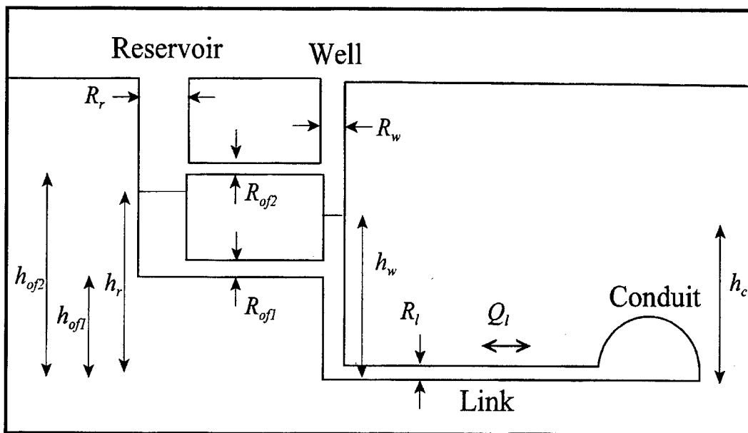
Figure 12: Tandem overflows between the reservoir and well. For all simulations, R_l = 5 \text{ mm} . R_w = 0.05 \text{ m} , f = 0.05 , l = 10 \text{ m} . Overflows lie 5 and 7 meters above link. Standard conduit hydrograph.
