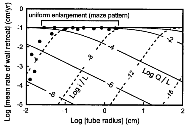
Figure 6: Many alternate routes are able to enlarge simultaneously at roughly the same rate, regardless of size, if they are all able to sustain high discharges (e.g. because of steep hydraulic gradients) or short flow distances. Maze caves, epikarst, and pervasive labyrinthine porosity are produced in this way. Very small openings, or those with low Q/L or i/L will not be competitive.
