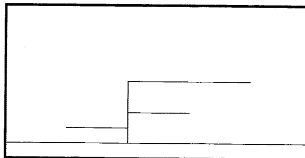
Figure 3c: Plan view of 5.5 m contact depth and horizontal conduit locations - Small scale grid ( x = 1,000 m, y = 500 m, z = 7.5 m)
