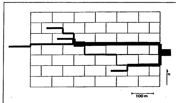
Figure 1: Mathematically simulated karst flow system designed with coupled expressions describing fluid flow and limestone dissolution kinetics to study factors that determine conduit selectivity (Groves and Howard, 1994b).
