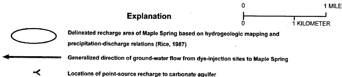
Figure 2: Time-of-travel estimates to Maple Spring, assuming porous-media flow, compared to dye-tracing results.
