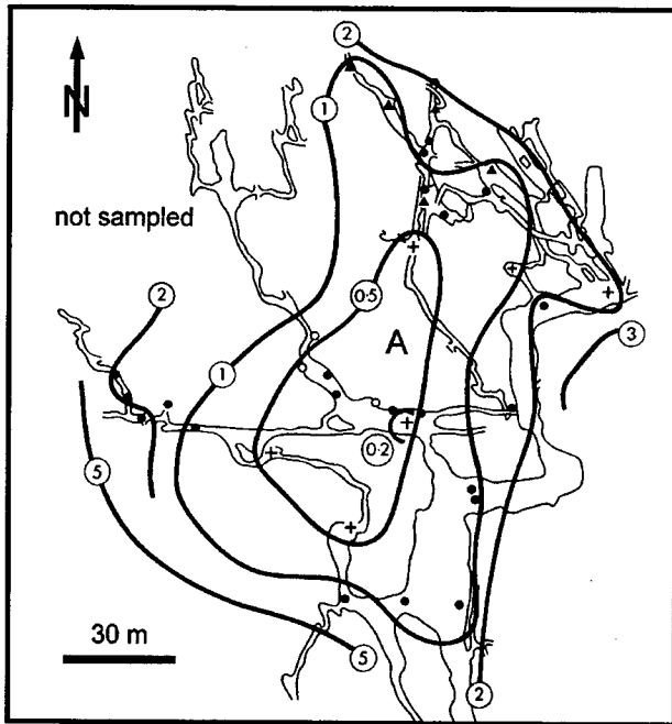
Figure 10: Distribution and first-arrival time (days) or vadoso seepage into underlying cave passages in GB Cave, Mendip Hills, U.K., as determined from dye injection at point A (from Smart and Friederich, 1986). The carbonate units are prominently fractured and dip steeply southward. Vadoso seepage tends to be highly dispersed, in contrast to the flows that are capable of forming conduits.
