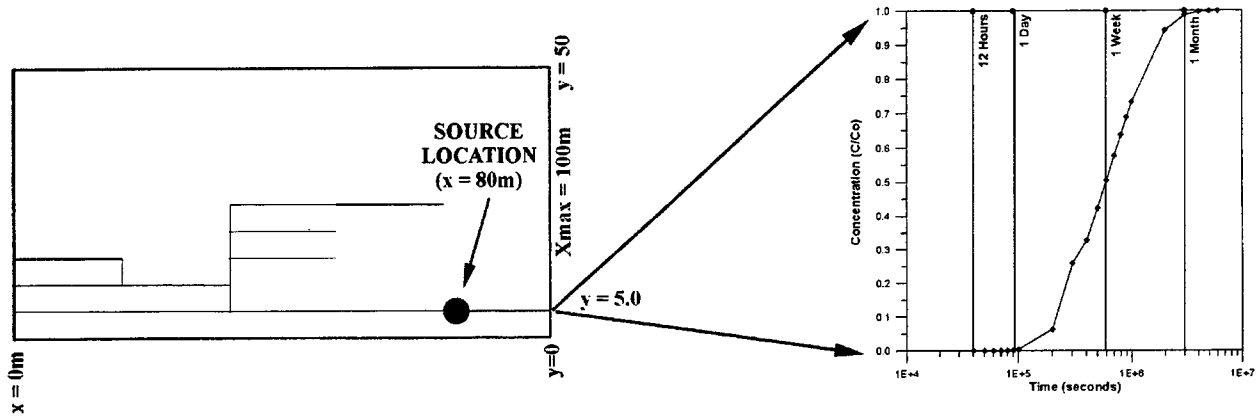
Figure 6. Simulation results - time of concentration to observation nodes - Small grid simulation ( x = 100 m, y = 50 m, z = 7.5 m)
