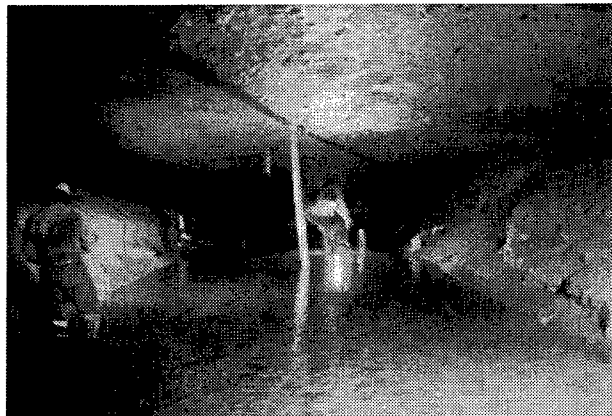
Figure 2: Logsdon River, Mammoth Cave Kentucky, showing the bottom three meters of a 145 m deep well through which water samples are collected under varying conditions. Another well, just out of the picture in the sediment alcove along the left side of the passage, delivers probes that measure temperature, stage, specific conductance, and velocity with two-minute resolution. Photo by Chris Groves.
