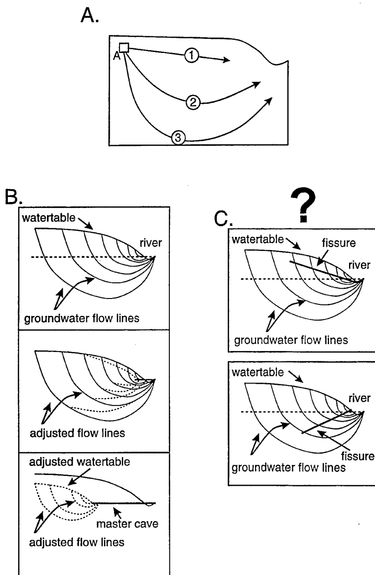
Figure 4: (A) Detail of the water-table cave model proposed by A. C. Swinnerton (1932). (B) The water-table cave model of Rhoades and Sinacori (1941). (C) How will the Rhoades and Sinacori model evolve if inappropriately oriented fissures are superimposed on it?
