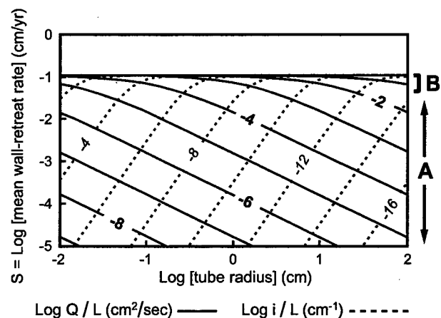
Figure 3: Mean rate of wall retreat (cm/yr) as a function of discharge ( Q ), flow distance ( L ), hydraulic gradient ( i ), and tube radius ( r ) in tubular conduits at 10° C and P_{\text{CO}_2} = 0.01 atm ( C_s = 212 mg/L CaCO 3 ). Values of i/L are valid only for laminar flow. A = region of varied growth rates ( Q/rL < 0.001 cm/sec); B = maximum possible solutional growth rate, limited by chemical kinetics. (From Palmer, 1981.)
