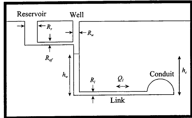
Figure 8: Definition diagram for overflow to adjacent reservoir. For all simulations, R_w = 0.05 m, R_l = 5 mm, f = 0.05 , l = 10 m. Standard hydrograph.
