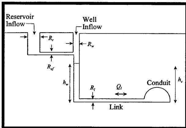
Figure 15: Definition diagram for surface recharge of the well and the reservoir. The recharge is likely to appear as a subsurface inflow.
