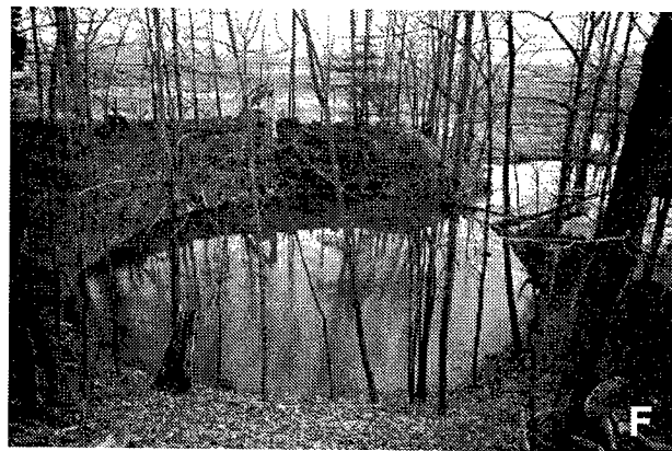
A: Epikarst exposed in Salem Limestone quarry, Indiana. B: Sinkhole development in a suburban lawn, Bowling Green, Kentucky. C: Mature sinkhole configuration, McClung's Cave, West Virginia. D: Karren topography and sinkholes (dolines), Croatia. E: Spring in Slovenia fed by a large cave system, Planinska jama (water-supply flume on left). F: Artesian karst spring rising into a valley filled with 30 m of late Pleistocene glacial and alluvial deposits, N.Y.
