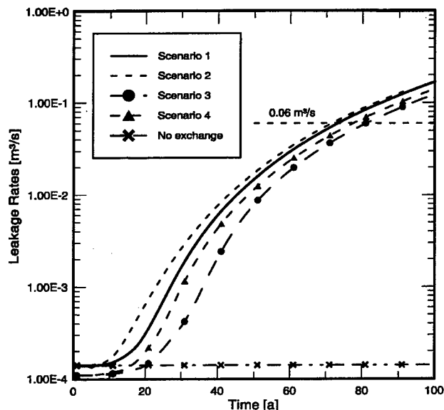
Figure 3: Development of leakage rates with time for the different scenarios. Also included is the leakage rate for a model with boundary conditions of Scenario 1, but no exchange between the fissured and conduit system.
