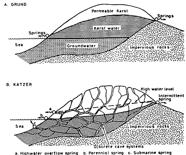
Figure 1: Groundwater flow models for the Dalmatian karst according to (A) Grund (1903); (B) Katzer (1909).
