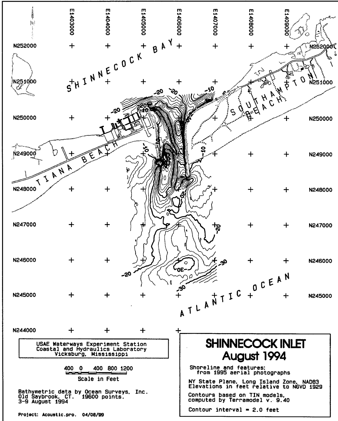
Figure B17. 3-9 August 1994
