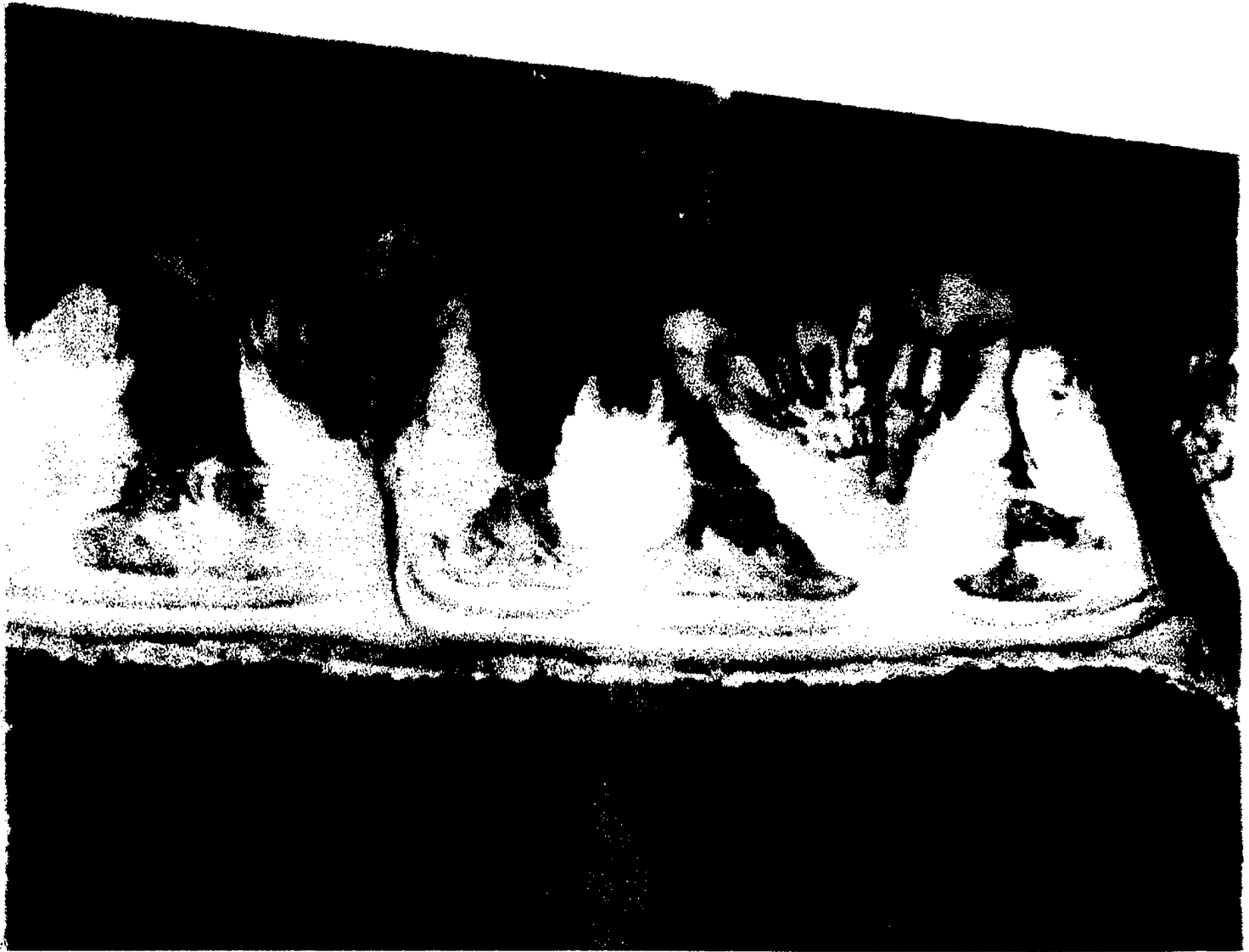
Figure 7. Mosaic of posthurricane aerial photographs taken 24 September 1938 (The tremendous power of this storm can be seen in the large numbers of washovers. Three breaches through barrier were cut, although westernmost one had almost closed and one widened over time and became present Shinnecock Inlet. Mosaic prepared by BEB or possibly USC&GS, from Engineer Waterways Experiment Station archives in Vicksburg, Mississippi. Shalowitz (USC&GS cartographic engineer) made measurements of inlets using these photographs (Howard 1939)) (Original photograph is 55 in. wide. This figure is 78 percent of full size.)
