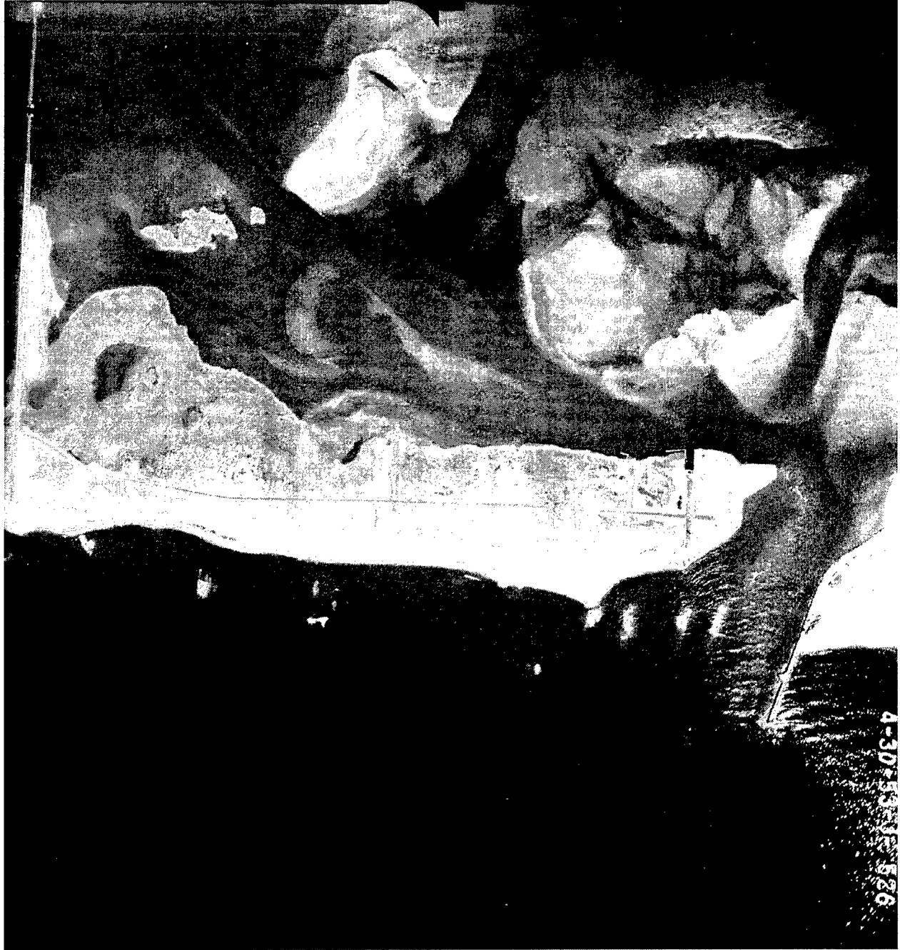
Figure A17. 30 April 1953 (East jetty has been completed. Channel has rotated to a NE-SW orientation, eroding inner shore of east beach to stone jetty, and a spit extends from the west beach into the inlet. A dredged navigation channel runs through the flood shoal to the northwest, where it meets Long Island Intracoastal Waterway at Ponquogue Bridge)
