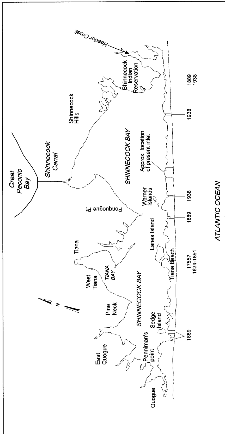
Figure 5. Location of historical inlets opening into Shinnecock Bay (Based on 1889-1890 USC&GS charts (modified from Leatherman and Joneja 1998))
