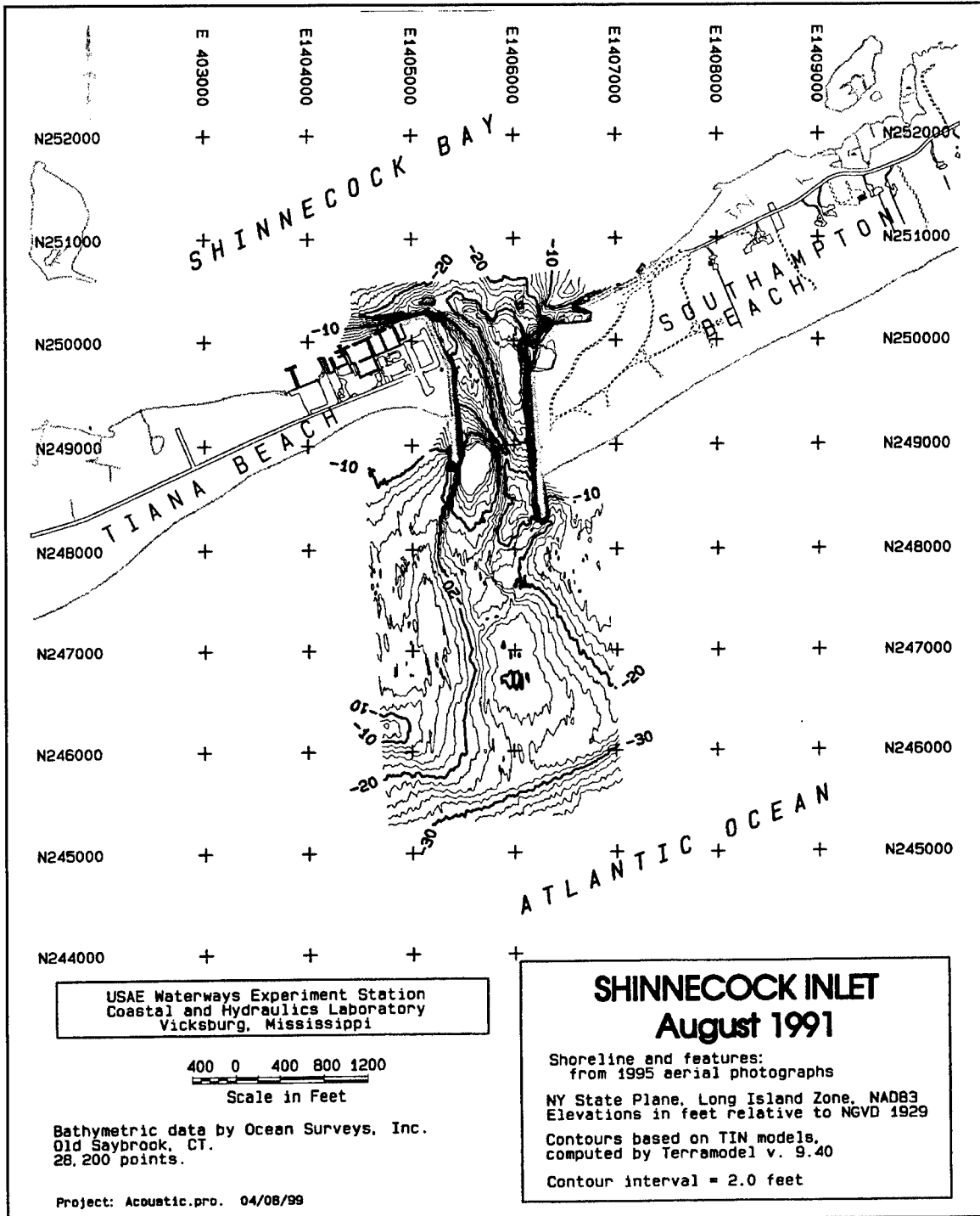
Figure B13. August 1991
