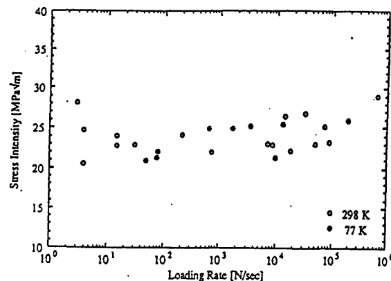
Figure 1. Effects of loading rate and test temperature on toughness of Nb-10Si (3).
