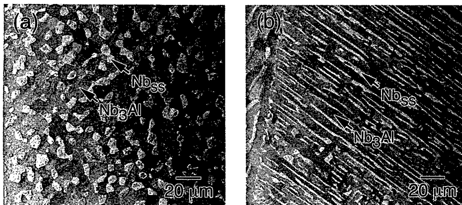
Fig.1 Scanning electron micrographs of Nb-18Al-31Mo annealed at 1500 °C for 100 h after isothermal forging (a) and solution treated at 1900 °C for 3 h and annealed at 1500 °C for 100 h after isothermal forging (b).
