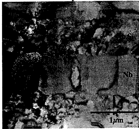
Figure 1: TEM cross-section of a Nb/Nb 5 Si 3 microlaminate after annealing at 1200°C for 3 hours showing the discrete layering, sharp interfaces, and lack of second phase formation in the Nb layers.
