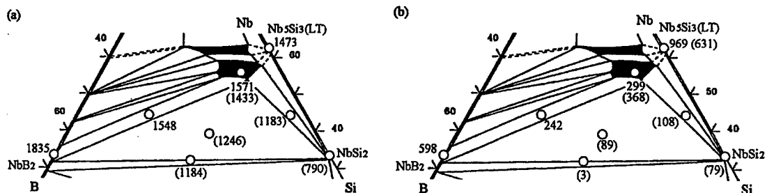
Fig. 3 (a) Microvickers hardness at room temperature and (b) yield stress in compression at 1673K for PSM powder compacts consolidated at 1973K and 1873K. Hardness and yield stress values for compacts consolidated at 1873K are shown in parentheses.
