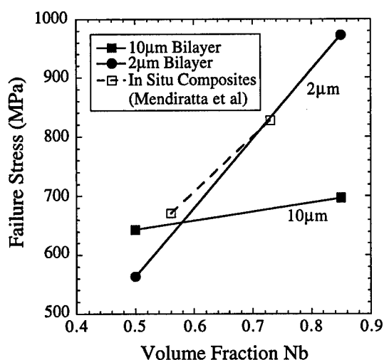
Figure 3: Failure Strength of Nb/Nb 5 Si 3 microlaminates. Note that strength tends to increase with volume fraction of Nb.
