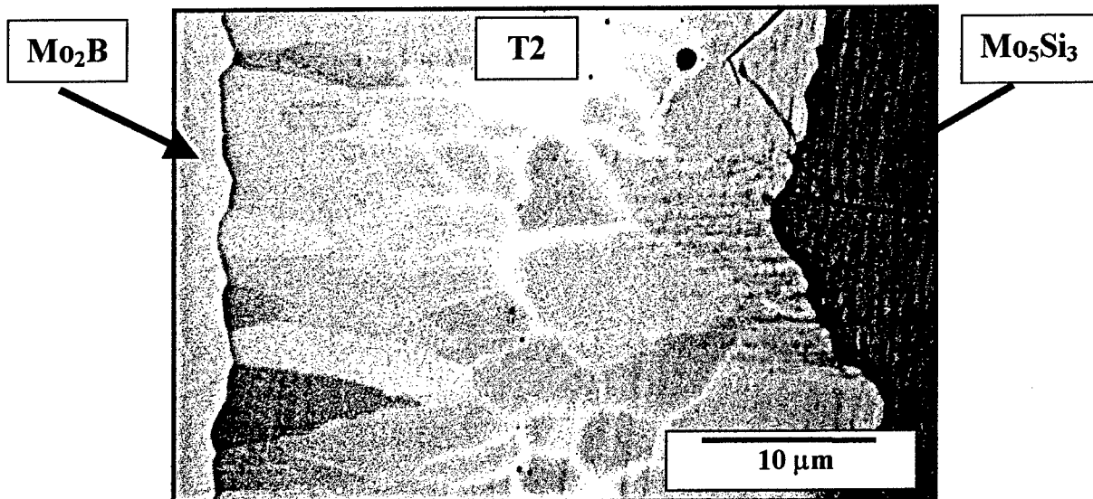
Figure 6: Back-scattered image of the cross section of the diffusion couple \text{Mo}_2\text{B}/\text{Mo}_5\text{Si}_3 annealed at 1600^\circ\text{C} for 400 hrs.
