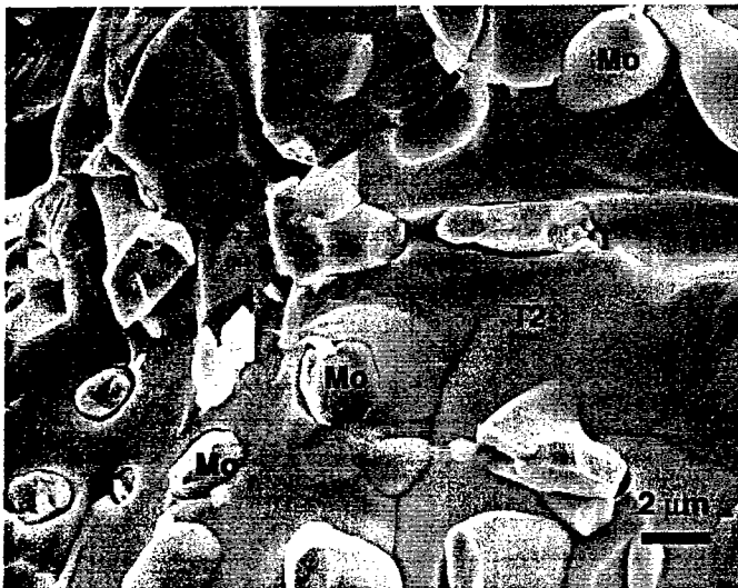
Fig. 1. Room temperature fracture surface of Mo-12Si-8.5B (at. %) illustrating ductile phase toughening due to \alpha -Mo inclusions
