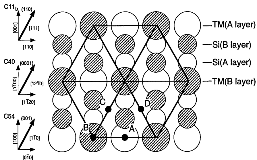
Fig.1 Atomic arrangements in the TMSi_2 layers and crystallographic directions are given with respect to C11 b , C40 and C54 structures.
