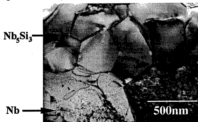
Figure 2: TEM cross-section of a Nb/Nb 5 Si 3 interface in a microlaminate which was annealed at 1400°C for 100 hours. Notice the sharpness of the interface, and the lack of significant interfacial grooving.
