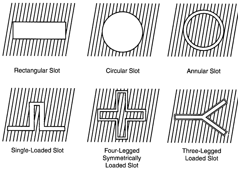
Figure 25. Frequency Selective Surface Geometries
