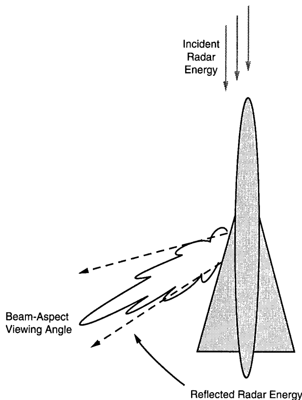
Figure 18. Radar Reflection from an Aircraft Planform with a Highly Swept Straight Leading Edge
