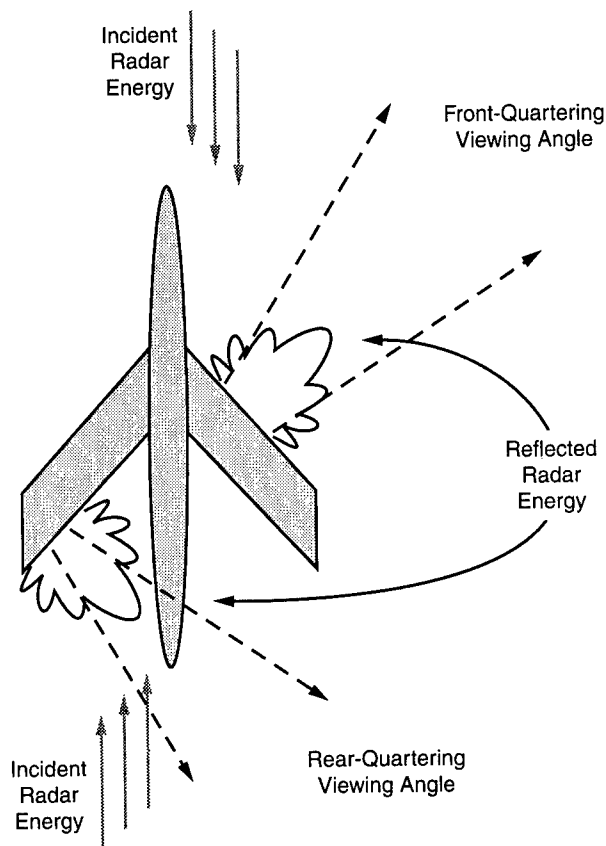
Figure 16. Radar Reflections from Aircraft Planform with Increased Wing Sweep
