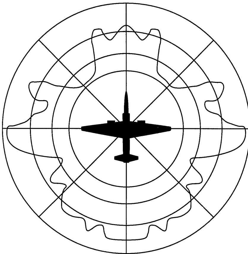
Figure 7. All-Azimuth Plot of an Aircraft RCS
