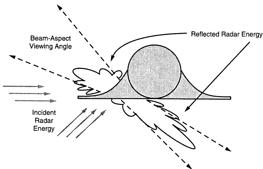
Figure 22. Aircraft with Chine and Fuselage Blended
