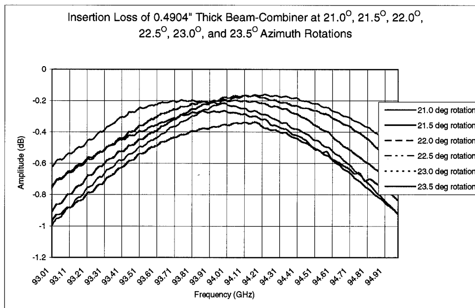
Figure 4. Insertion loss of dichroic beam combiner as a function of incidence angle.
