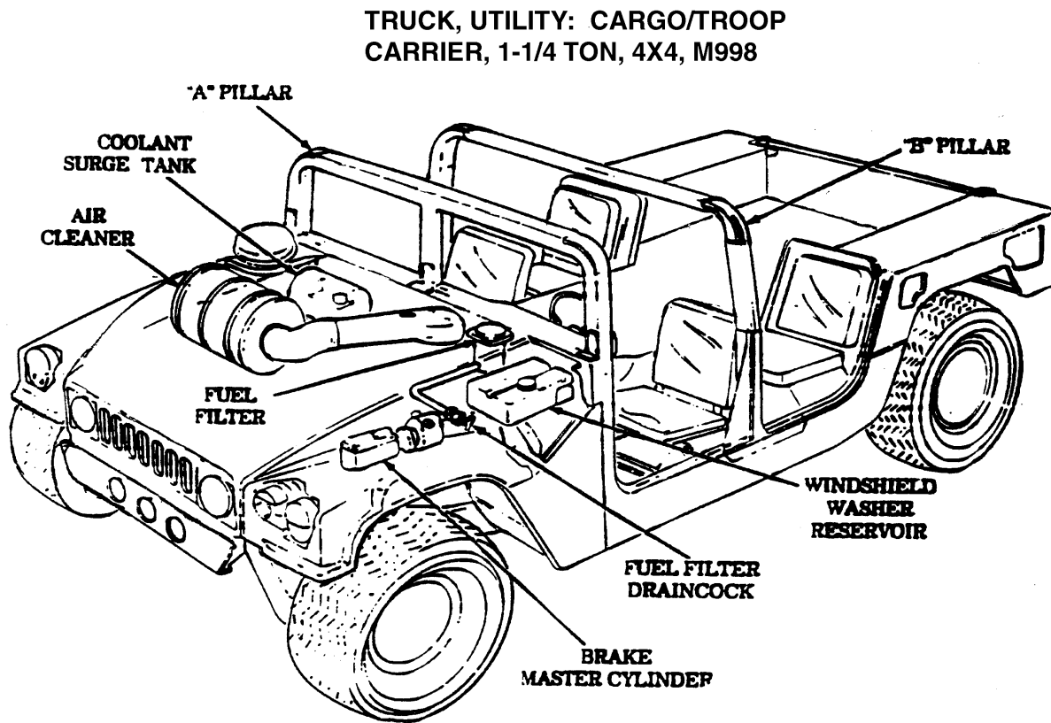
Figure 1. HMMWV: Major components.
