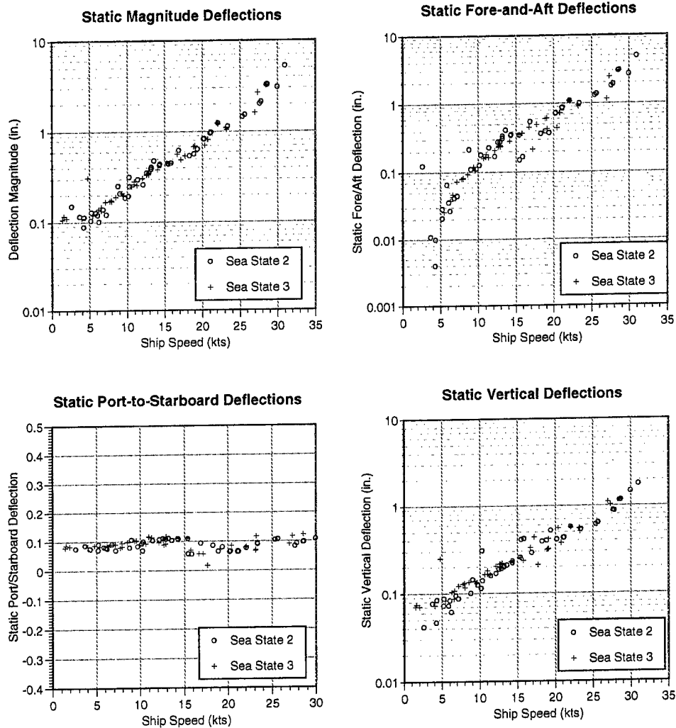
Figure 5. USS Radford SDRW Static Deflections vs. Ship Speed (Log/Linear Scale)
