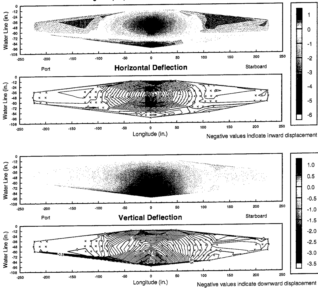
Figure 3: USS Radford SDRW Deflection Color Contour Plots
