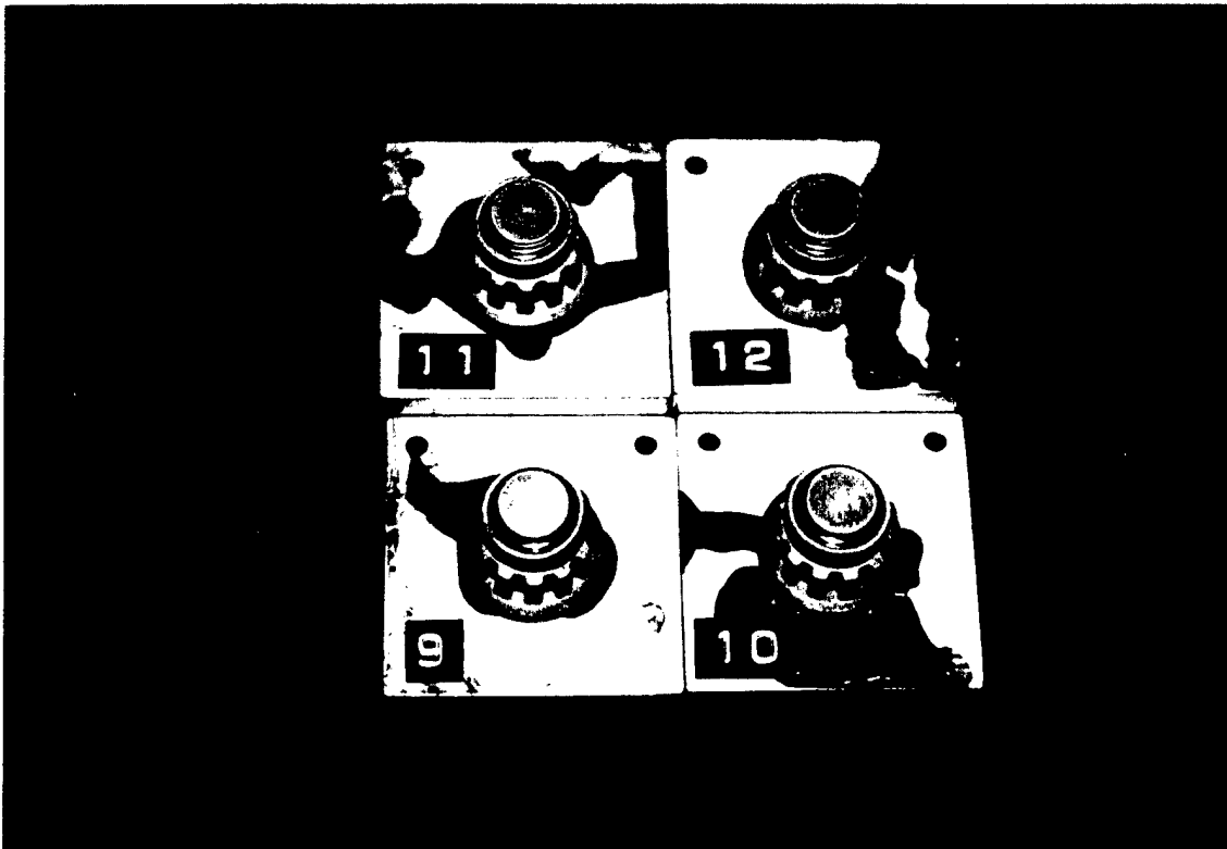
Figure 7. Inconel 718 Nickel-Based Superalloy Nuts With Antiseize Solid Film Lubricant (MoS 2 ) Before Salt Spray Exposure. Reduced 25%.
