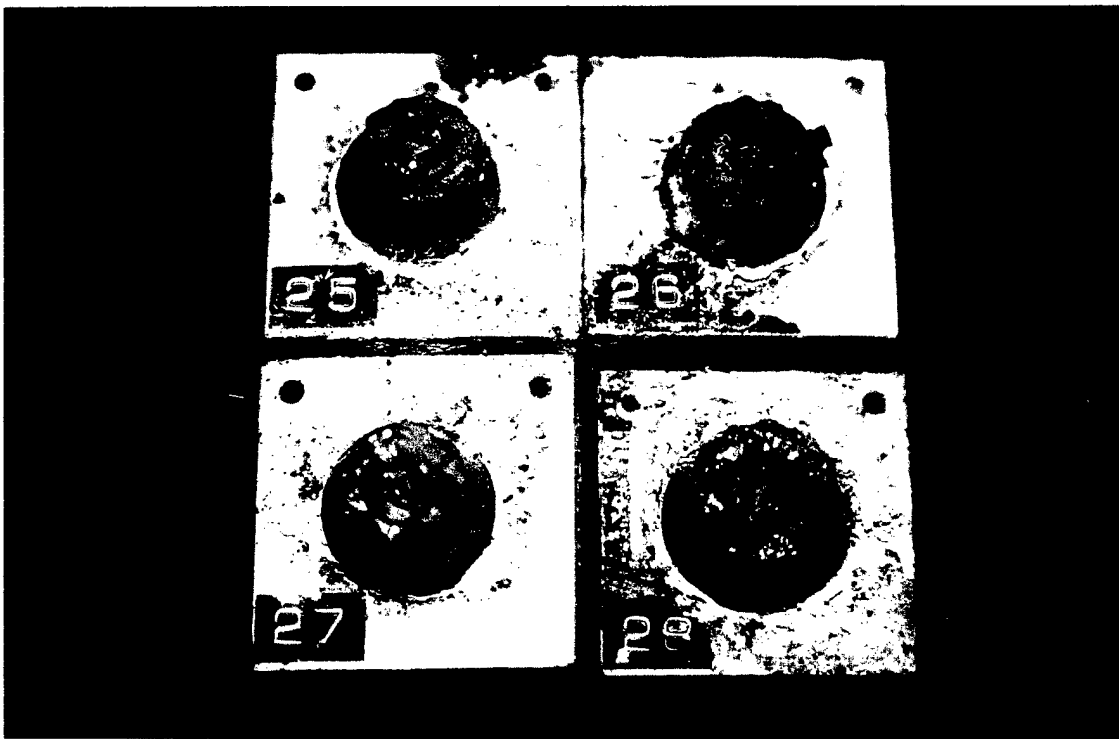
Figure 82. H11 Chromium Hot Work Tool Steel Nuts With Antiseize Solid Film Lubricant (MoS 2 ) 62 Days of Salt Spray. Reduced 25%.
