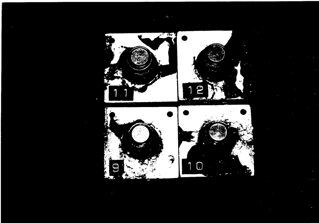
Figure 41. Inconel 718 Nickel-Based Superalloy Nuts With Antiseize Solid Film Lubricant (MoS 2 ) After 30 Days of Salt Spray. Reduced 25%.
