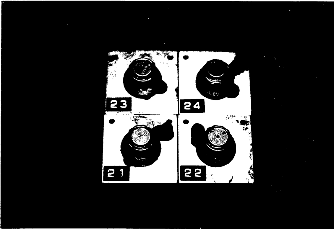
Figure 13. H11 Chromium Hot Work Tool Steel Nuts With Cadmium Electroplate Before Salt Spray Exposure. Reduced 25%.
