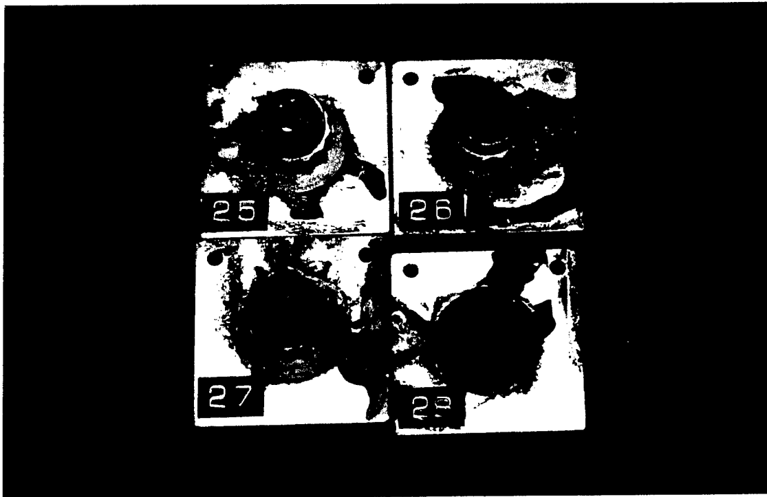
Figure 32. H11 Chromium Hot Work Tool Steel Nuts With Antiseize Solid Film Lubricant (MoS 2 ) After 15 Days of Salt Spray. Reduced 25%.
