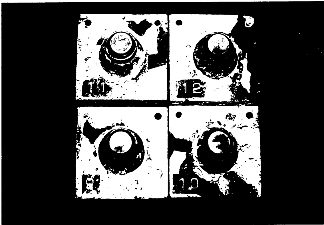
Figure 75. Inconel 718 Nickel-Based Superalloy Nuts With Antiseize Solid Film Lubricant (MoS 2 ) After 62 Days of Salt Spray. Reduced 25%.
