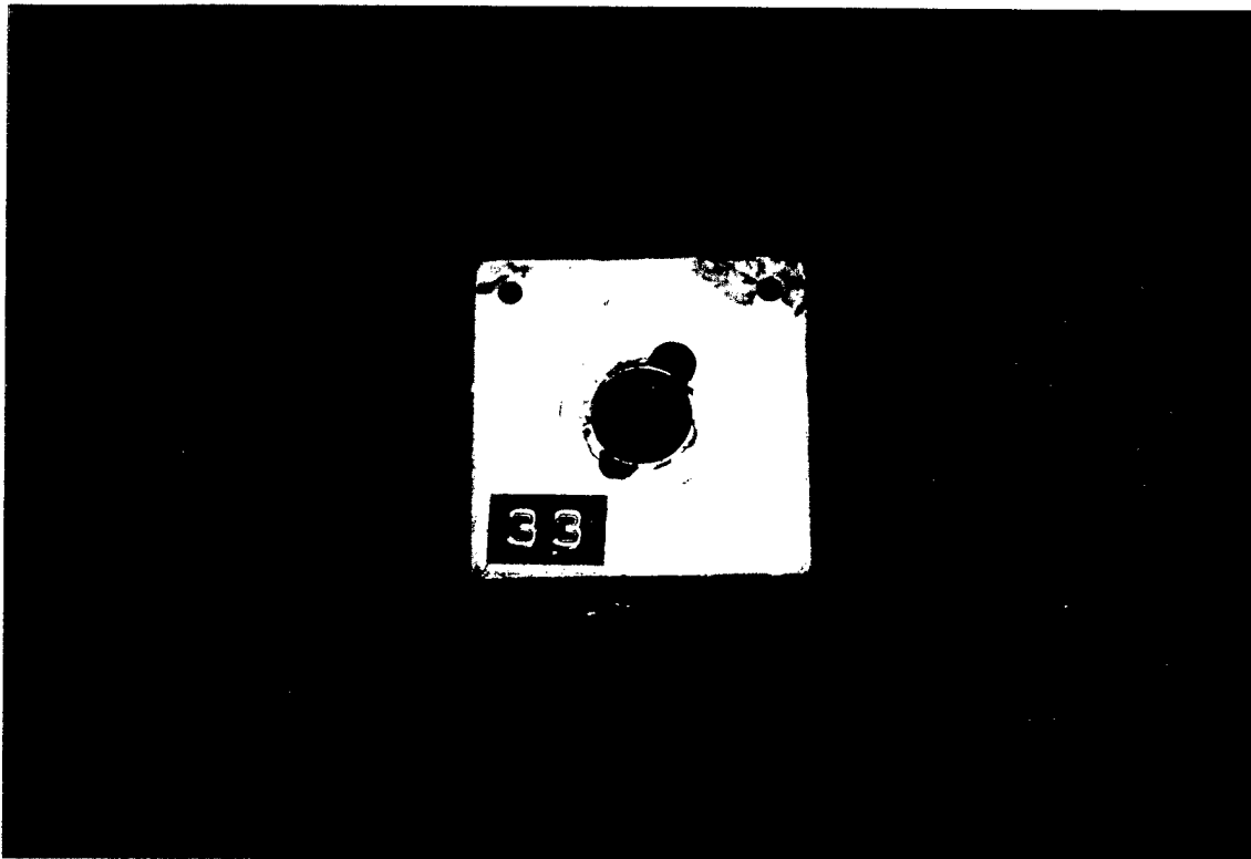
Figure 69. Aluminum Control Block After 44 Days of Salt Spray. Reduced 25%.
