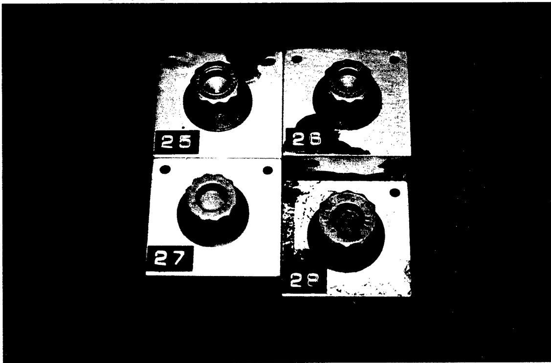
Figure 14. H11 Chromium Hot Work Tool Steel Bolt Heads With Antiseize Solid Film Lubricant (MoS 2 ) Before Salt Spray Exposure. Reduced 25%.
