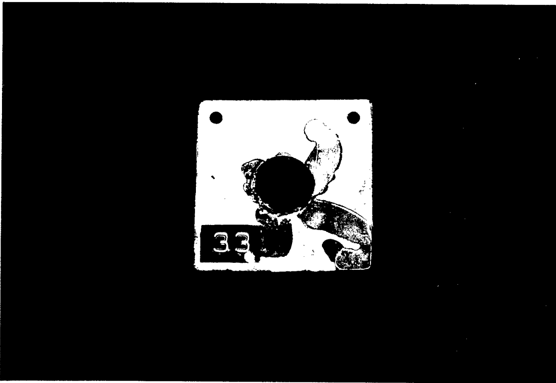
Figure 86. Aluminum Control Block After 62 Days of Salt Spray. Reduced 25%.
