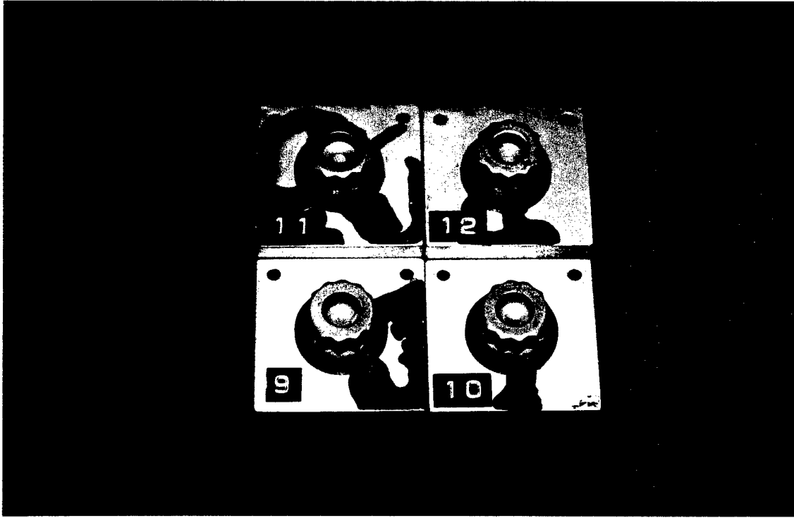
Figure 6. Inconel 718 Nickel-Based Superalloy Bolt Heads With Antiseize Solid Film Lubricant (MoS 2 ) Before Salt Spray Exposure. Reduced 25%.
