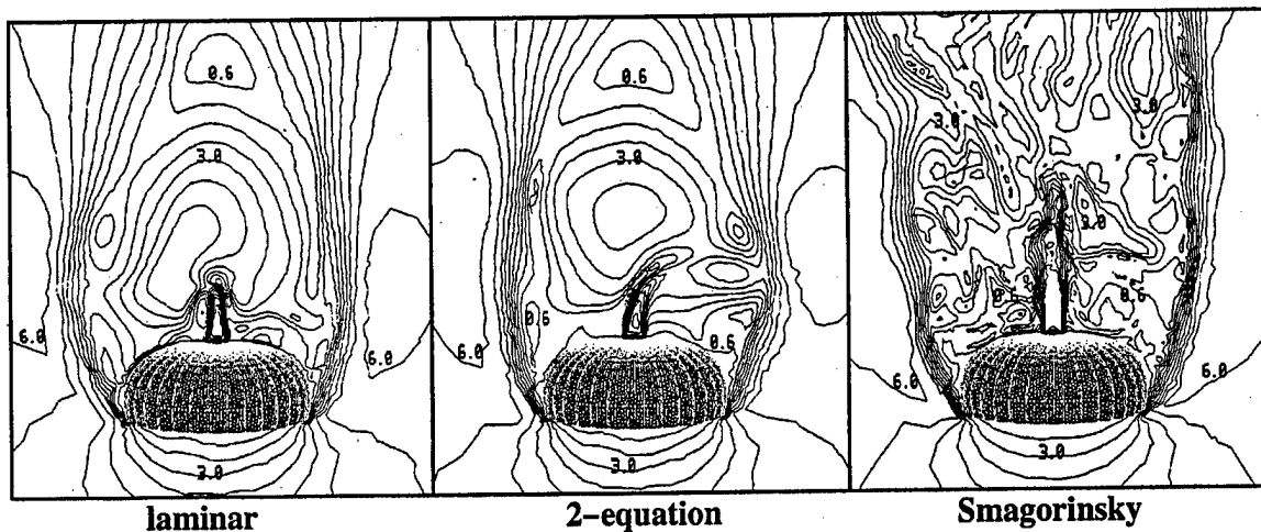
Figure 7. Computed Velocity Magnitude Contours:
