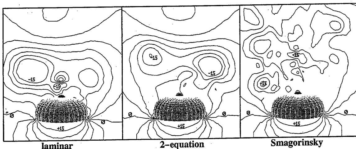
Figure 6. Computed Pressure Contours.
