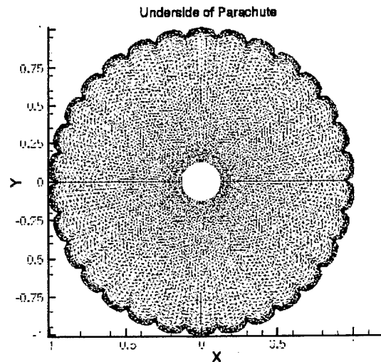
Figure 1. Computational Surface Mesh for T-10.
