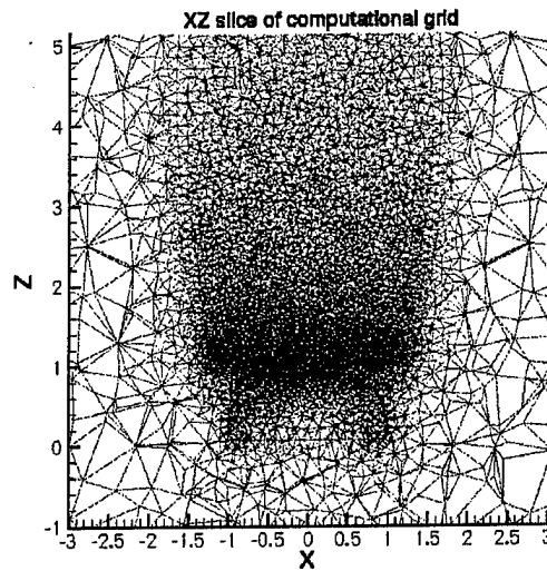
Figure 2. Slice of Computational Mesh in x-z.
