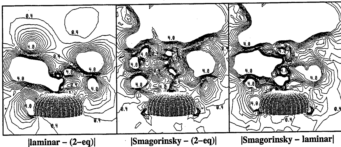
Figure 9. Computed Pressure Comparisons (contours of \delta p between the simulations).
