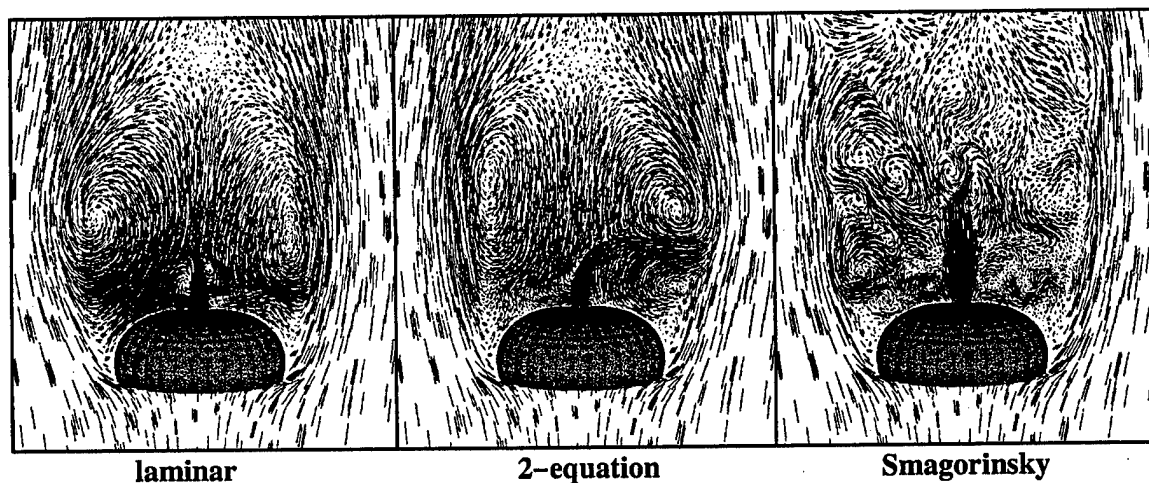
Figure 8. Computed Velocity Vectors.
