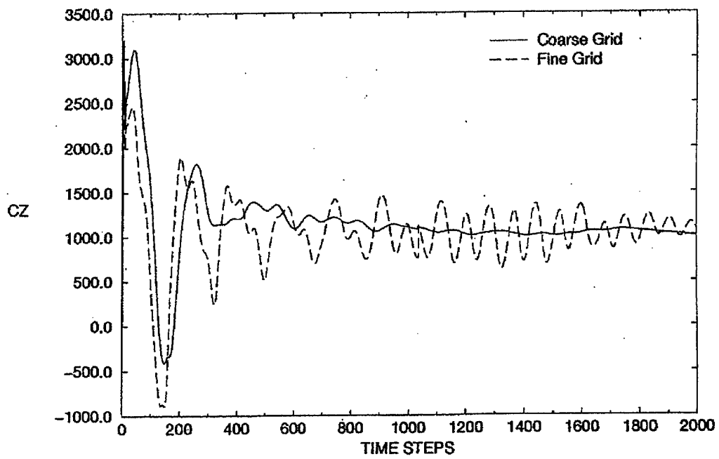
Figure 17. Convergence of Drag for G-12 Canopy.
