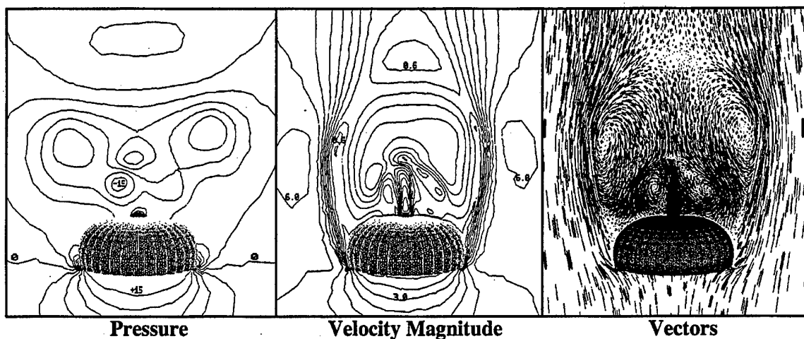
Figure 11. Computed Results With One-Equation Model.
