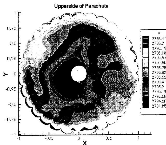
Figure 5. Pressure Contours on the Upper Surface.
