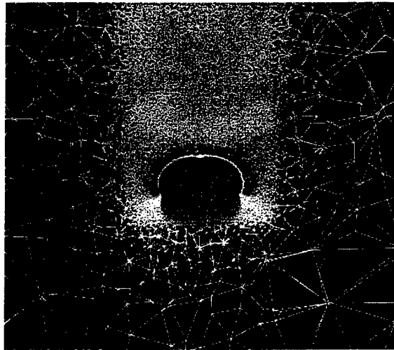
Figure 14. Mesh for G-12 Parachute Without Payload.
