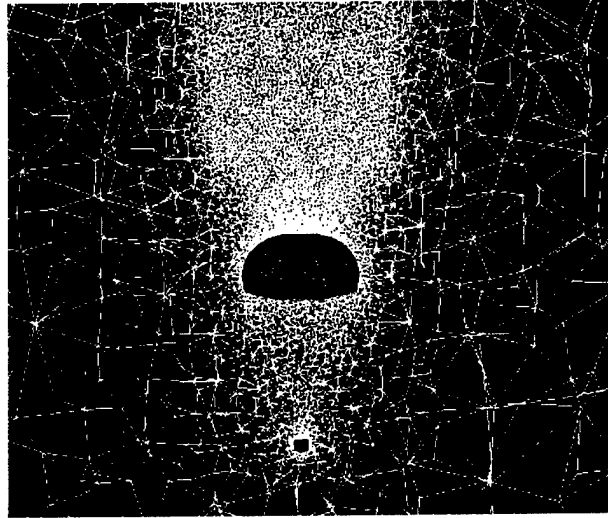
Figure 18. Mesh for G-12 Parachute With Payload.
