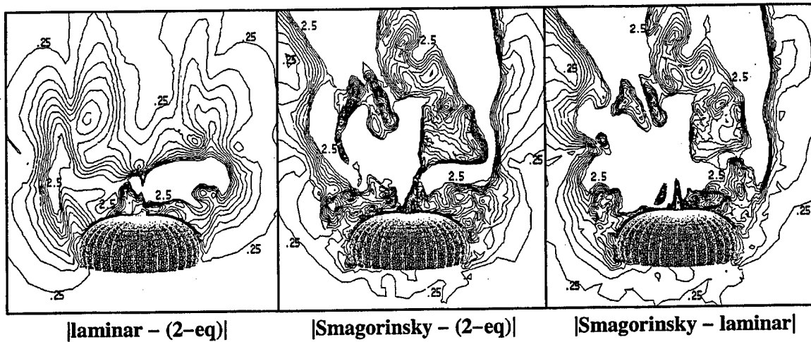
Figure 10. Velocity Magnitude Comparisons (contours of \delta |v| between the simulations).
