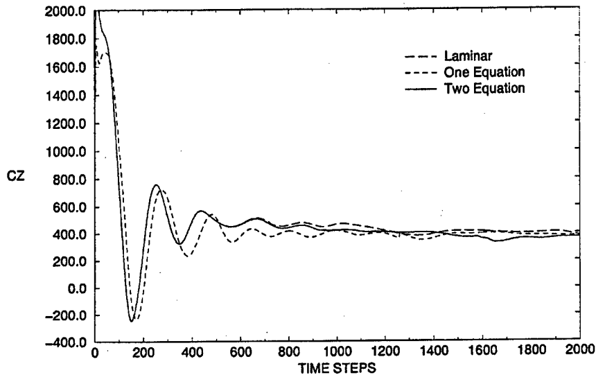
Figure 13. Time History for Drag for T-10 Parachute.
