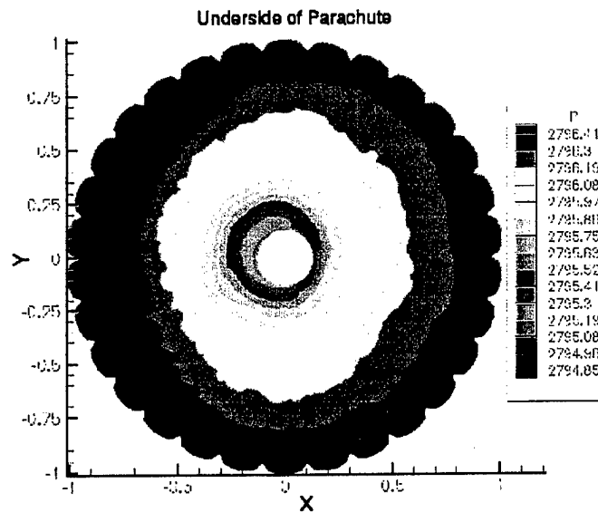
Figure 4. Pressure Contours on the Lower Surface.
