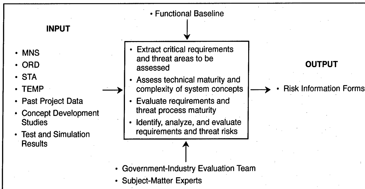
Figure 5-7. Threat and Requirement Risk Assessment Technique Input and Output
