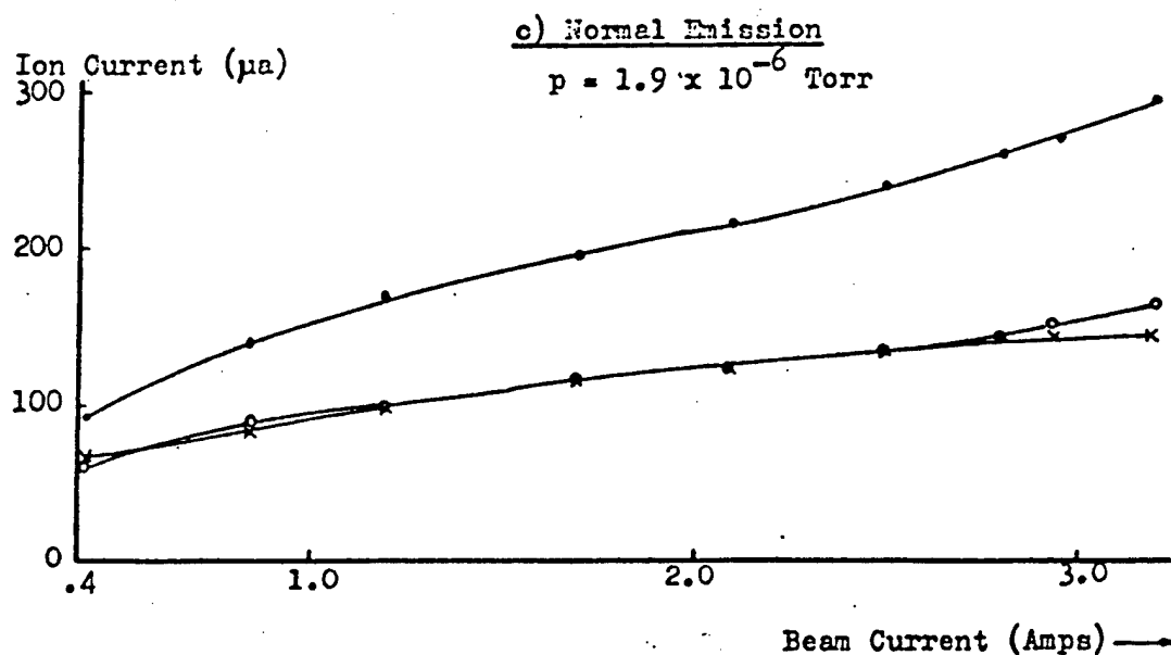
FIG.31 ION CURRENT vs. BEAM CURRENT(METHOD I)
