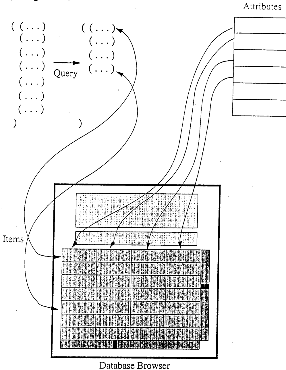
Figure 2.11. Set/Database browser.
