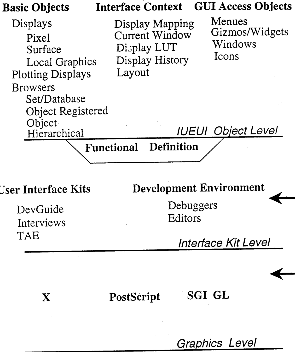
Figure 2.1. Interface Levels.
