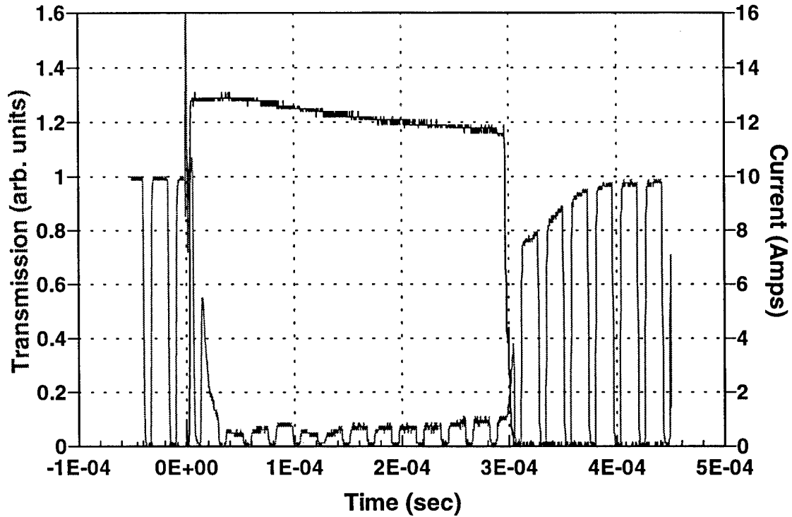
Figure A1. A plot of the plasma current and the microwave transmission for an EG mode plasma. Source frequency is 11 GHz. The background gas is oxygen at 31 mTorr (4.13 Pa). The magnetic field is 280 gauss ( 2.8 \times 10^{-2} T) and the capacitor bank charge voltage is 3.5 kV.
