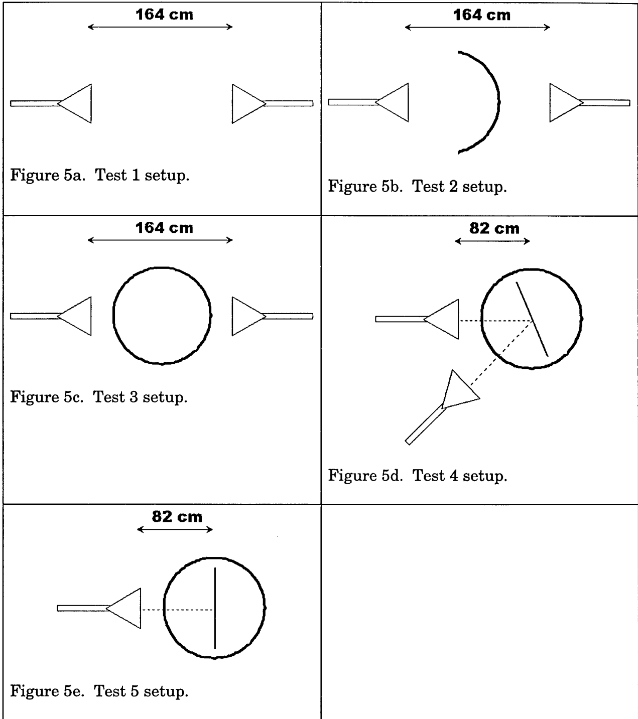
Figures 5a-e. Experimental arrangements for the five part test of reflected microwaves without a sheet plasma present.
