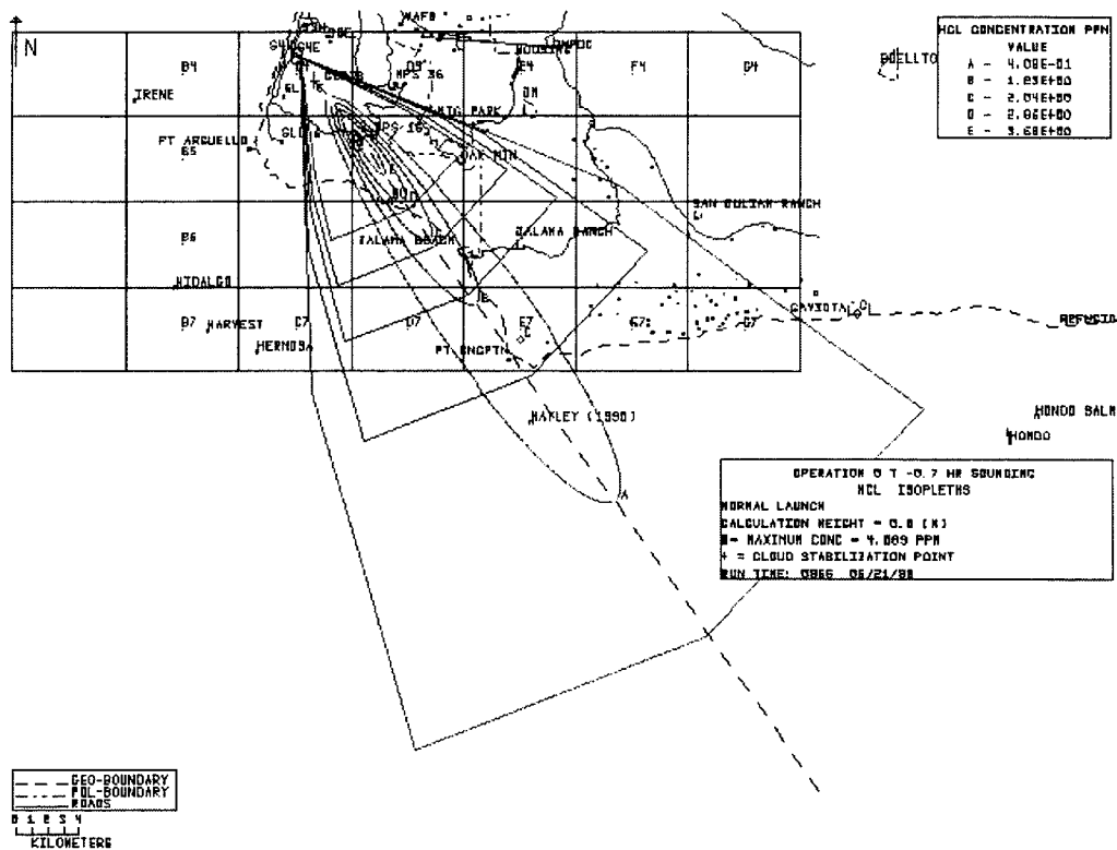
Figure 6A. HCL Surface Height Concentration Isopleth Predictions from REEDM Version 7.08 for A-18 Mission Using T-0.7h Rawinsonde Data.
