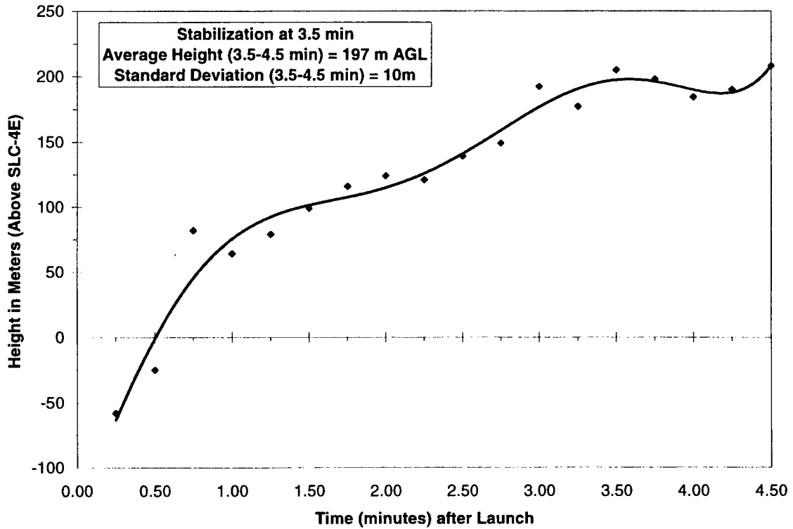
Figure 10. Cloud rise for the bottom of the A-18 cloud (PLMTRACK upper and PLMVOL lower).
