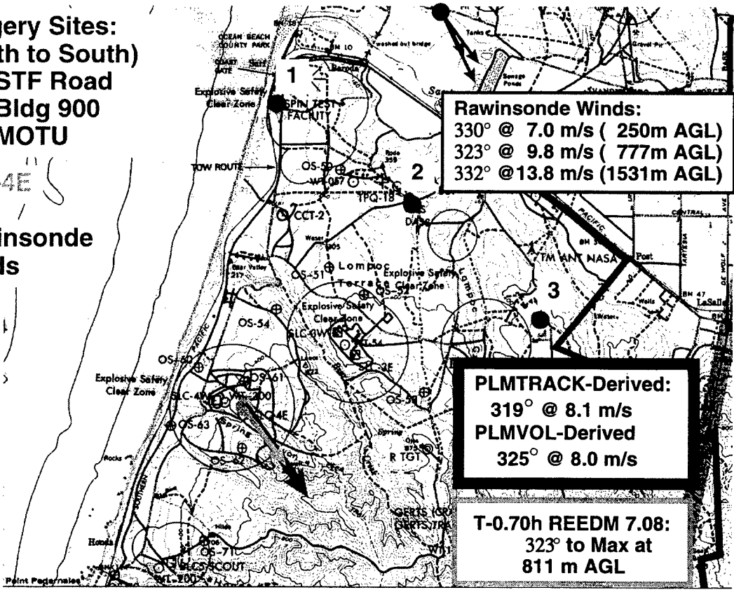
Figure 4. A Map Documenting the Imagery Sites, the A-18 Ground Cloud's Bearing (derived from infrared imagery), the T-0.7h REEDM Prediction for the Ground Cloud's Bearing ( at stabilization height), and the 01:52 GMT (T-0.7h) Rawinsonde Wind Directions at the Predicted Cloud Stabilization Heights (Bottom, Middle and Top).
