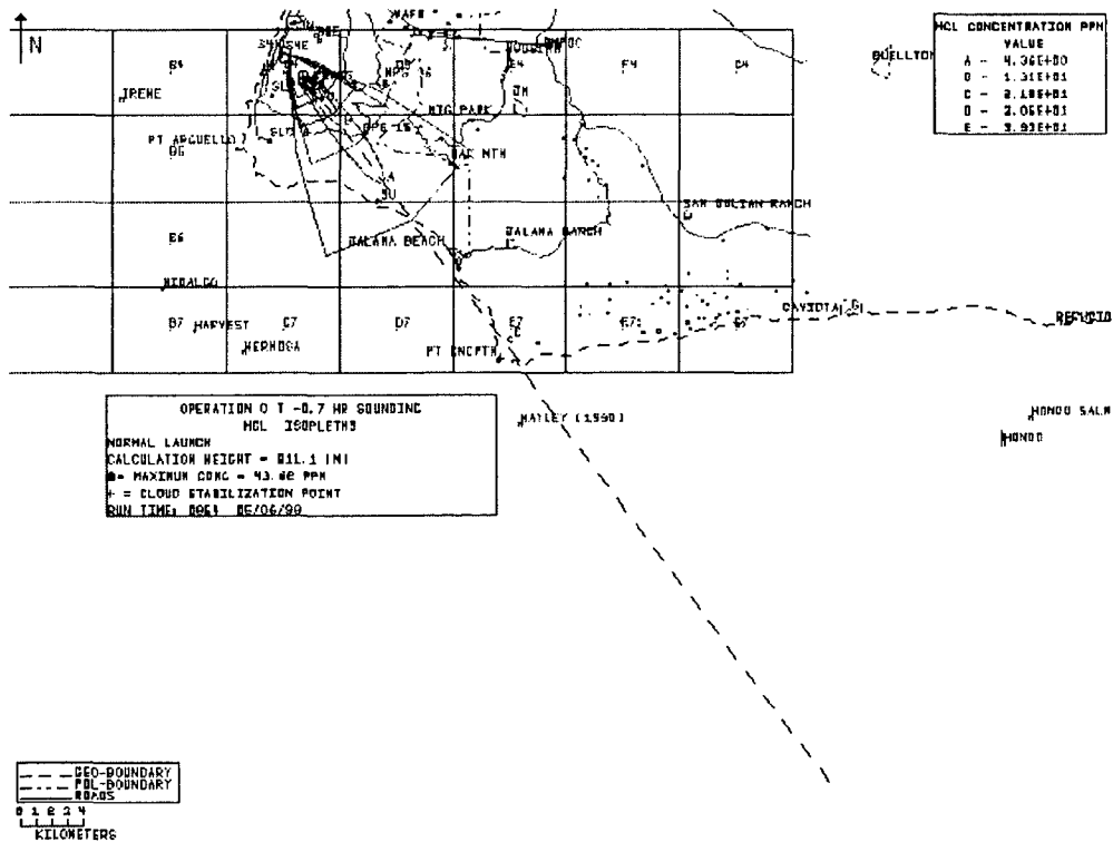
Figure 3A. HCl Stabilization Height Concentration Isopleth Predictions from REEDM Version 7.08 for A-18 Mission Using T-0.7 h Rawinsonde Data.
