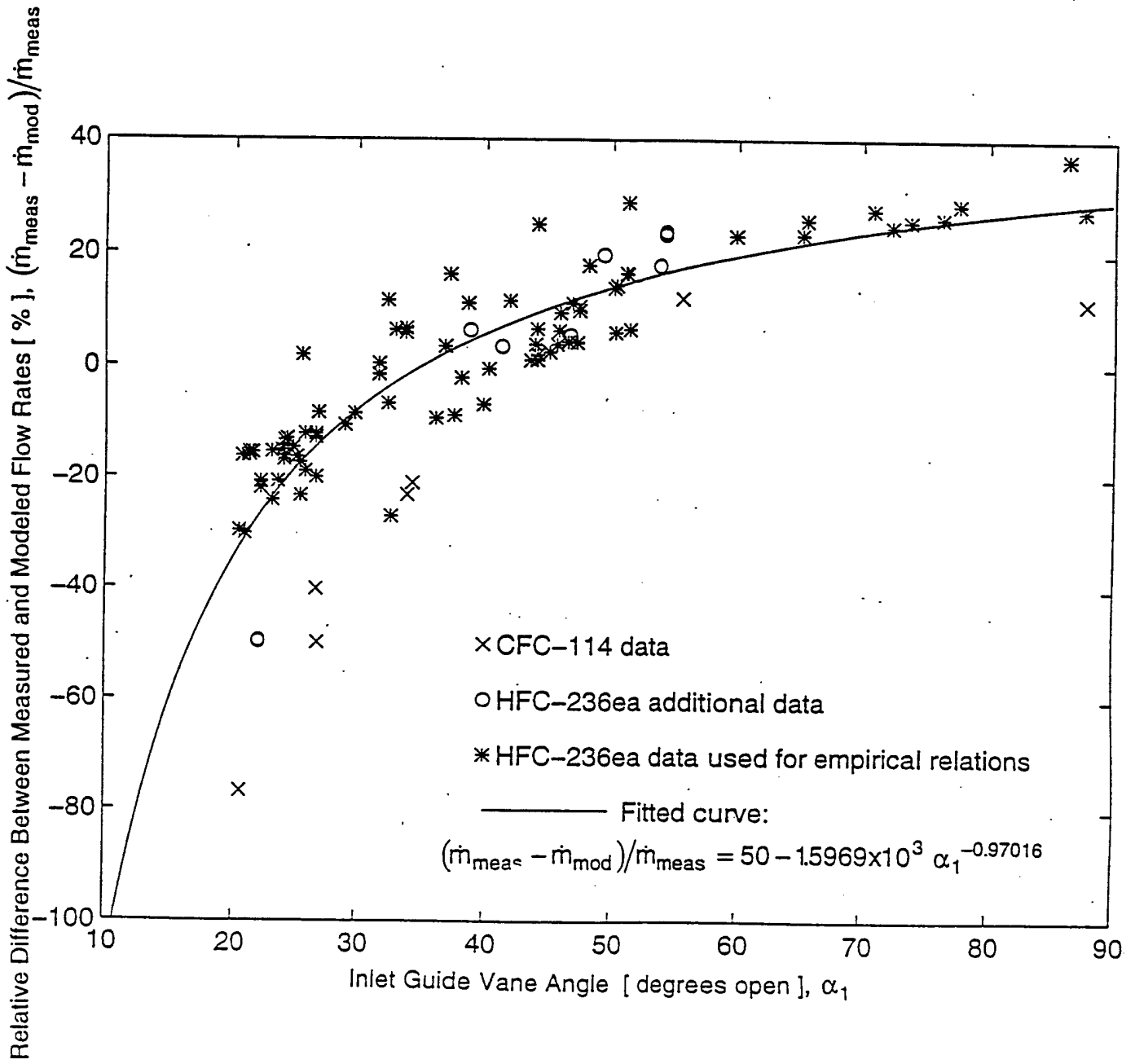
Figure 5.5. Flow rate prediction error as function of guide vane angle.
