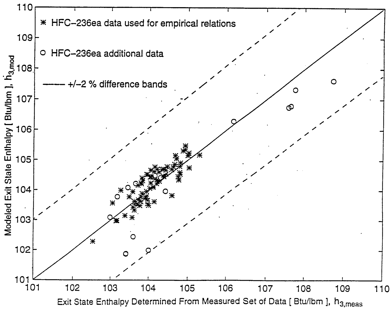
Figure 5.7. Comparison between modeled and measured exit enthalpies for HFC-236ea data points.
