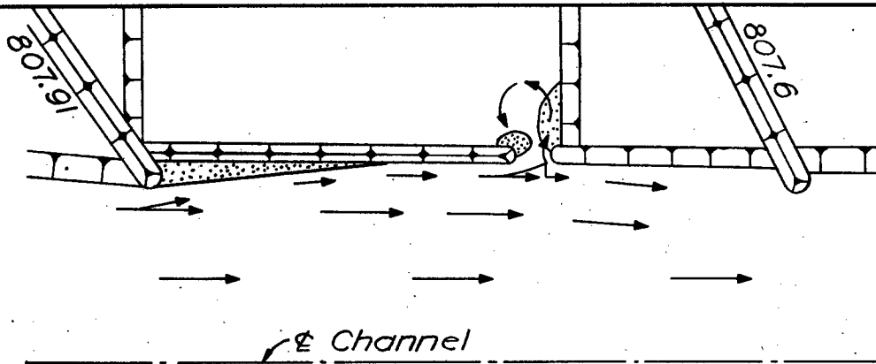
FIG. 1 - Basin formed by trail dike parallel to channel alignment. Entrance formed by opening in dike.
