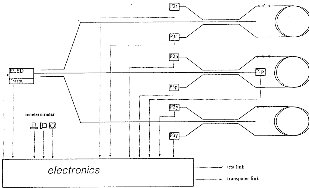
Fig. 7 Principle configuration of the IMU
