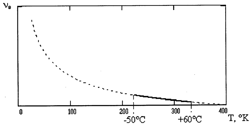
Fig. 5.18. Theoretical dependance v_B versus absolute temperature.
