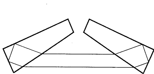
Four-prism Cavity with Reversed Second Prisms.
