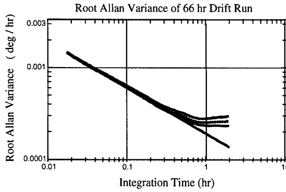
Figure 8: Rate uncertainty (dotted line) vs. integration time for the Honeywell precision FOG. The solid straight line is the \tau^{-1/2} asymptote of the data, revealing 0.00019^\circ/\sqrt{hr} ARW. The curved solid lines show the error bars of the variance determination.
