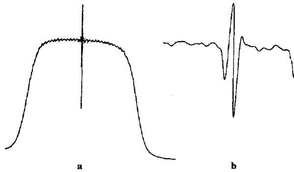
Fig. 12.13. The output pulse of the interference NI (a - the whole output pulse, b - the central part of the pulse in a bigger scale).
