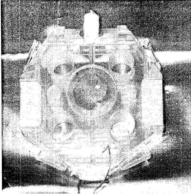
Fig. 6. 7. The Ring Laser with TRP Cavity.
