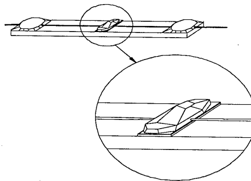
Fig.9.2. Exterior view of fiber optic polarizer
