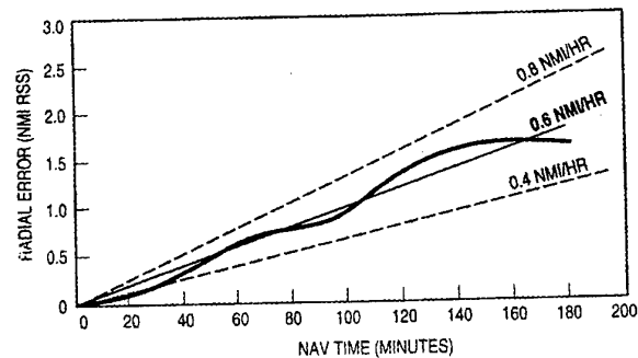
Figure-11 Typical Navigation Performance for ZLG Based Inertial System
