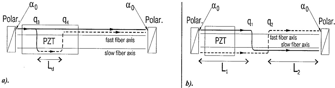
Fig.9.8. Two main mechanisms of arising of the quadrature signal (amplitude modulation of the optical signal in the FOG).
