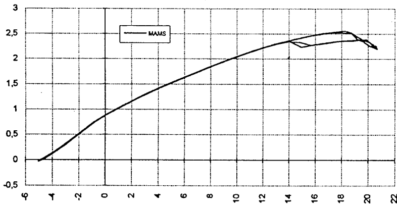
Figure 6.4 Lift Coefficient versus the Angle of Incidence as Windtunnel Test Result
