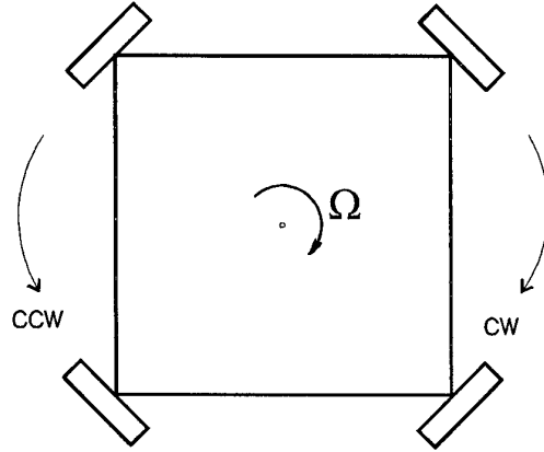
Fig. 5.7 The four-mirrors ring laser gyroscope sensor rotating with an angular rate \Omega .
