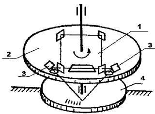
Fig.12.33. The method of direct recording the circular scales by means of the interference pattern formed by waves counterpropogating in the ring laser cavity.
