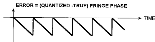
Figure 9b - Gyro Quantization Error
