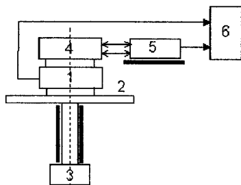
Fig.12.1. Schematic of the ring laser goniometer. 1 ring laser, 2 rotary table, 3 spindle with drive, 4 turning and 5 non-moving parts of angle converter, 6 counter.
