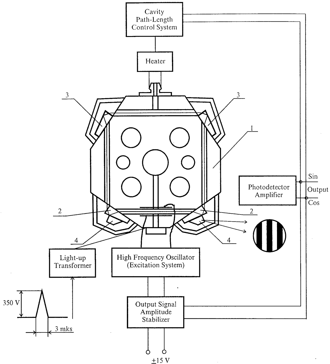
Fig 6.6. TRP LG structure diagram.
