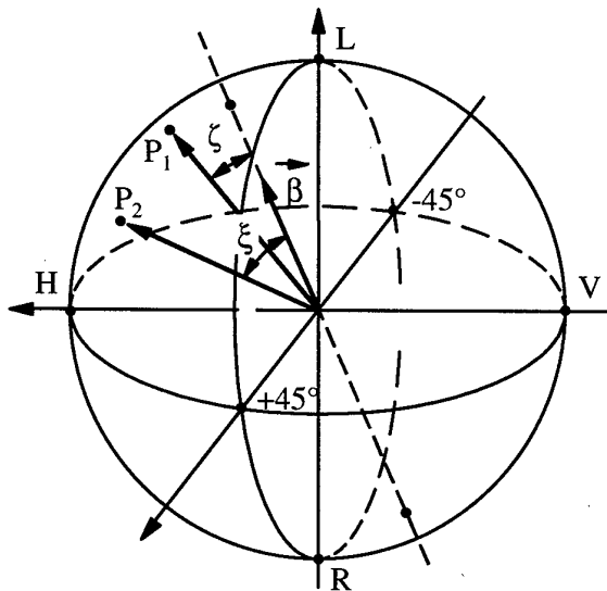
Figure 13: Sensitivity of polarization states P_1 and P_2 to arbitrary non-reciprocal birefringence
