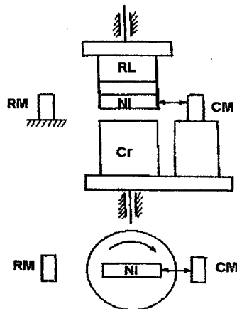
Fig.12.26. The scheme of the laser goniometer system in the diffractometer.
