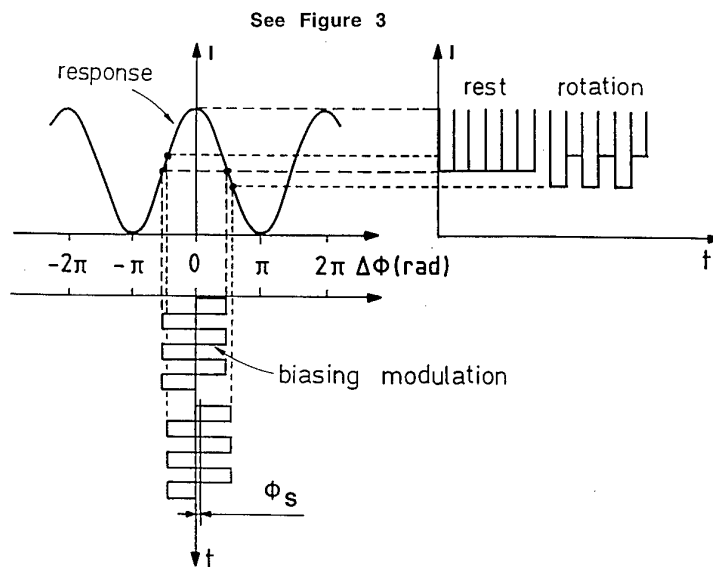
Figure 10 Generation of a modulation of the phase difference using the delay through the coil
