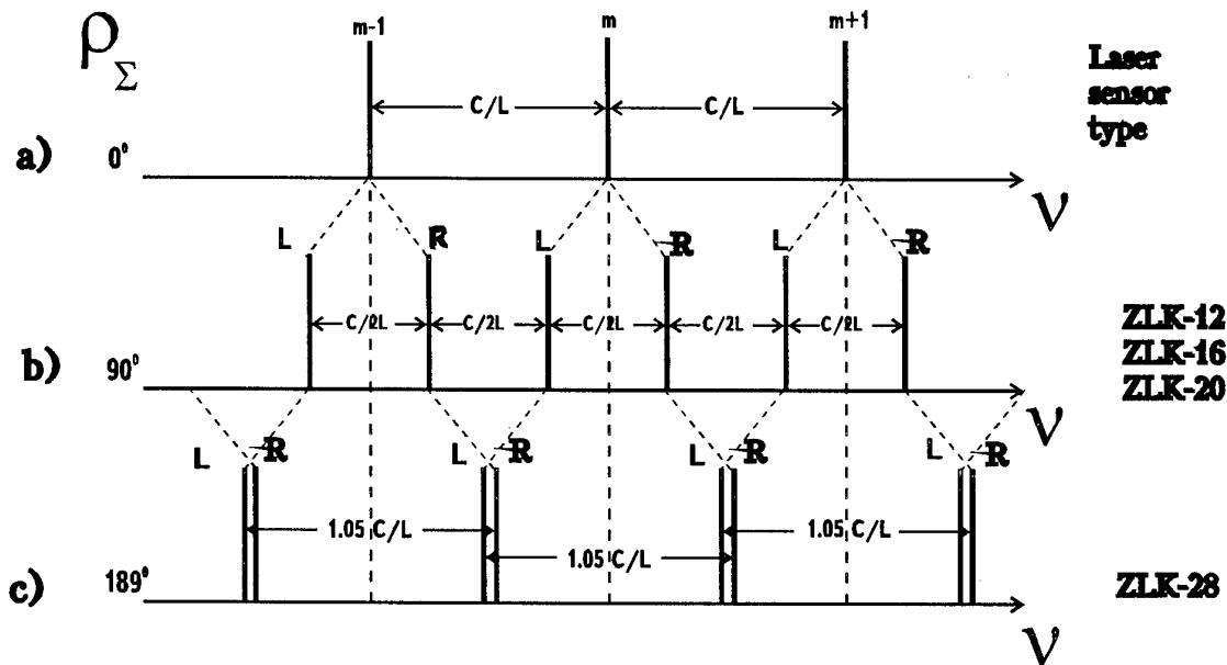
Fig. 5.9. The spectrum of natural frequencies of out-of-plane cavities as a function of a total angle of rotation \rho_\Sigma and types of sensors with out-of-plane cavities: a) a cavity with an equivalent plane contour, b),c) out-of-plane laser cavities: b) two-frequency ring lasers, c) four-frequency ring lasers.
