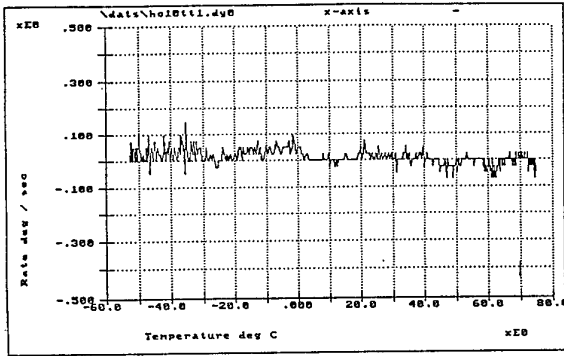
Fig. 5 Bias Error as Function of Temperature
