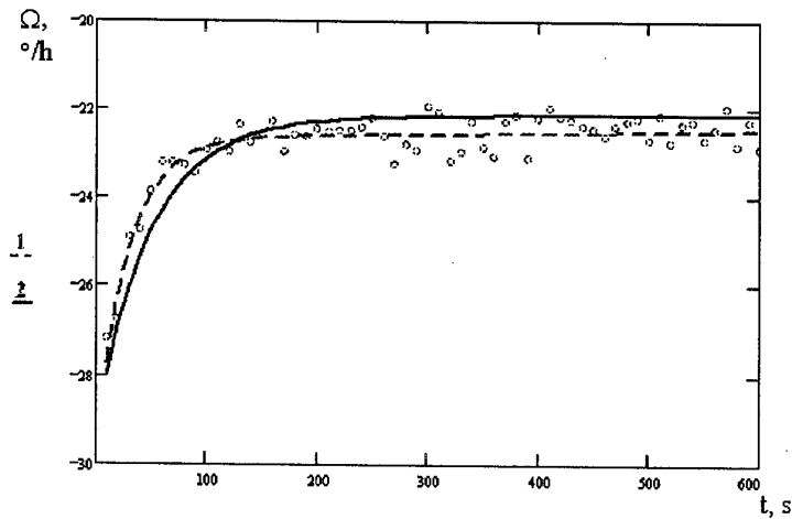
Fig. 5.20. Zeeman laser gyro typical dependence of zero drift \Omega vs time after turn-on (line 1 - average line of output data; line 2 - line of algorithmic correction).
